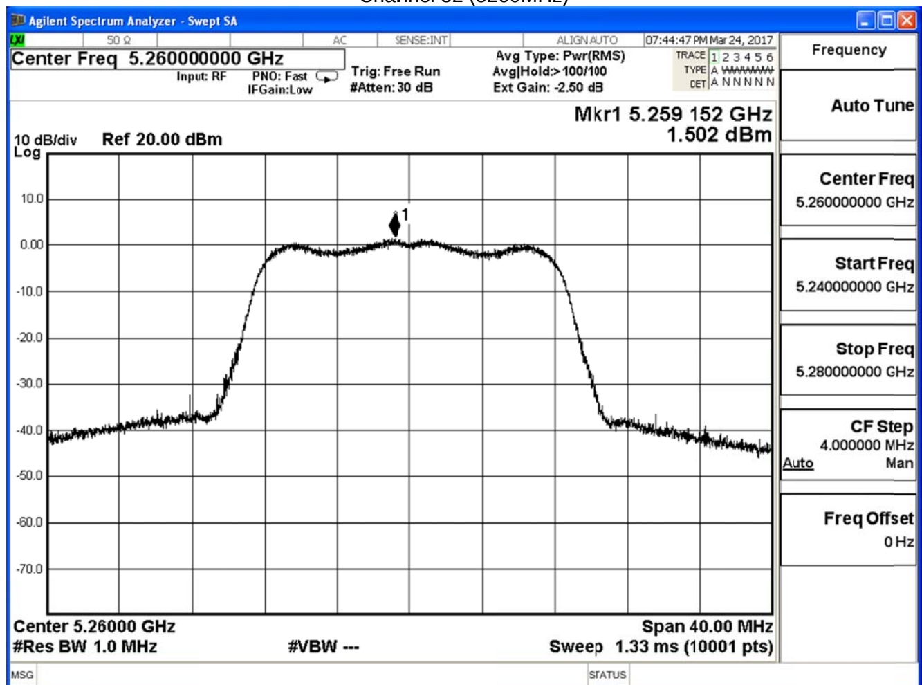
Channel 52 (5260MHz)
