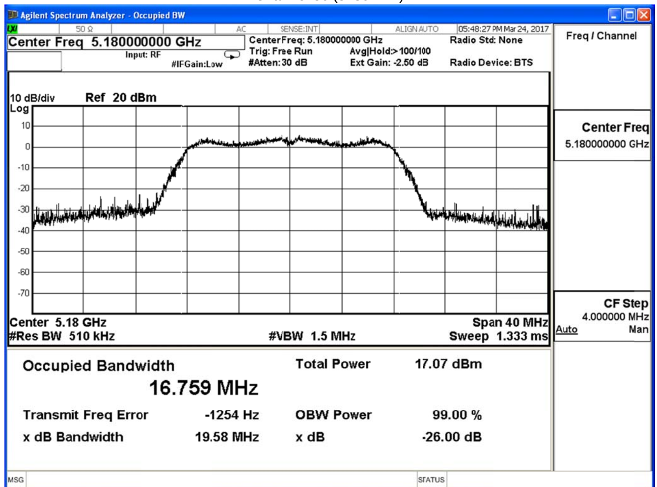
Channel 36 (5180MHz)
