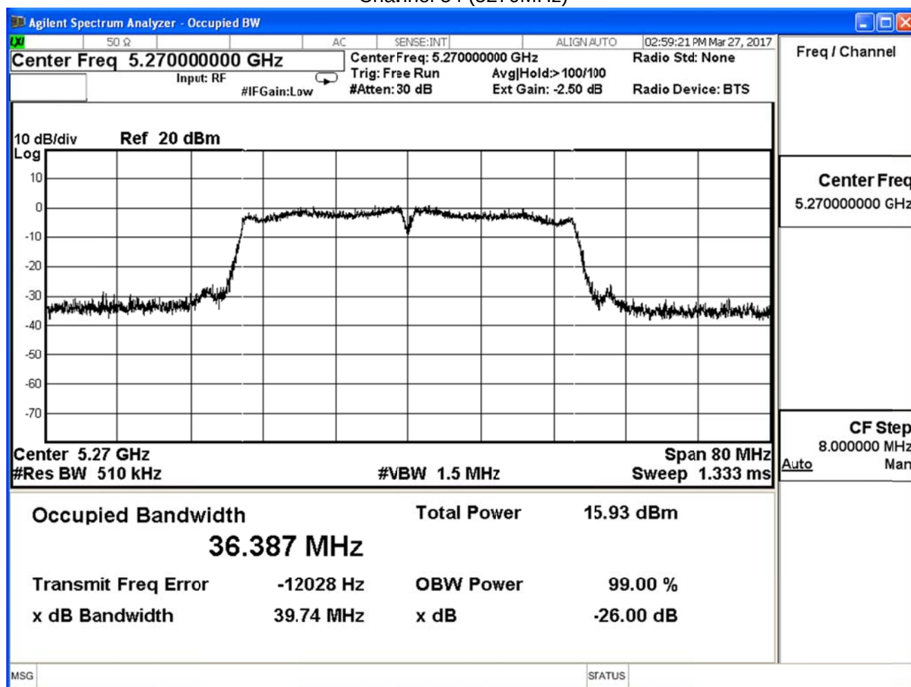
Channel 54 (5270MHz)
