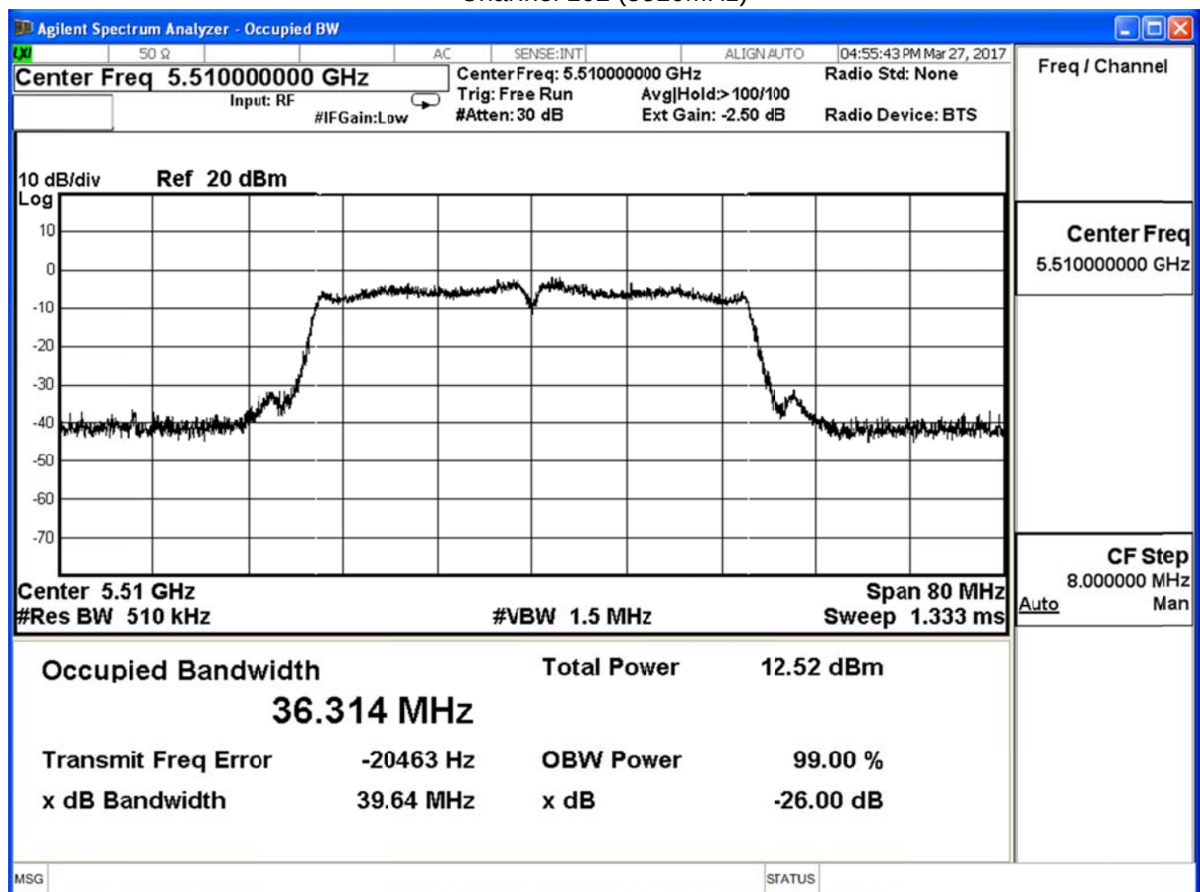
Channel 102 (5510MHz)
