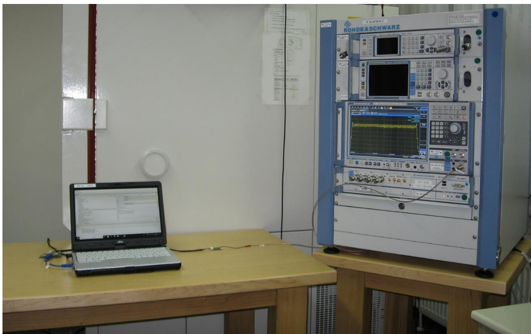
RF-conducted measurements
