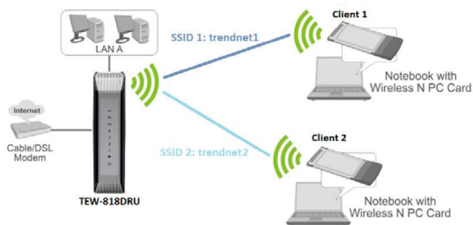
Access Point Mode with Multiple SSID
