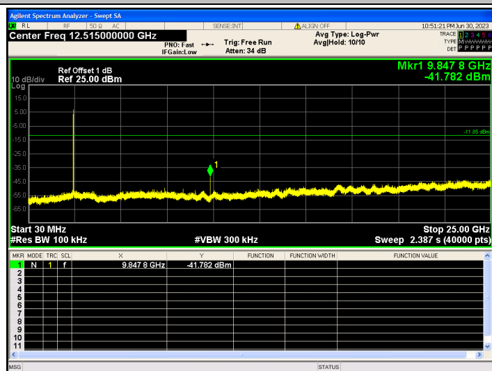
802.11g_2412_0~Reference
