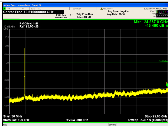
802.11n(HT20)_2462_0~Reference
