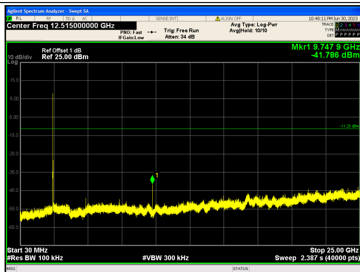
802.11b_2462_0~Reference
