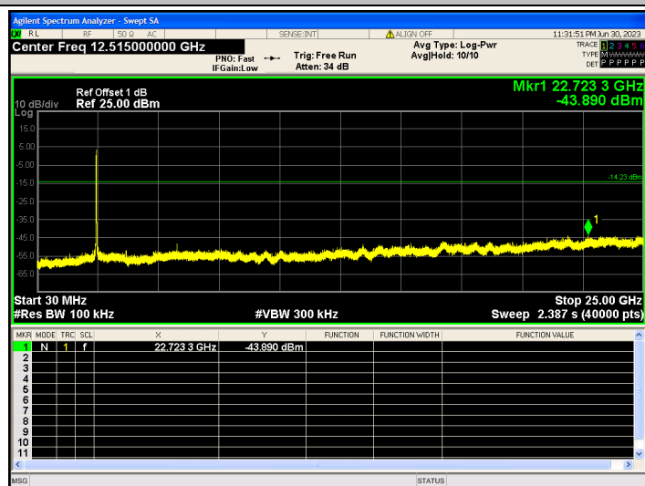
802.11n(HT40)_2422_0~Reference
