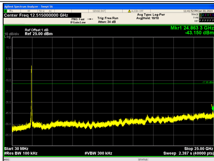
802.11n(HT40)_2452_0~Reference
