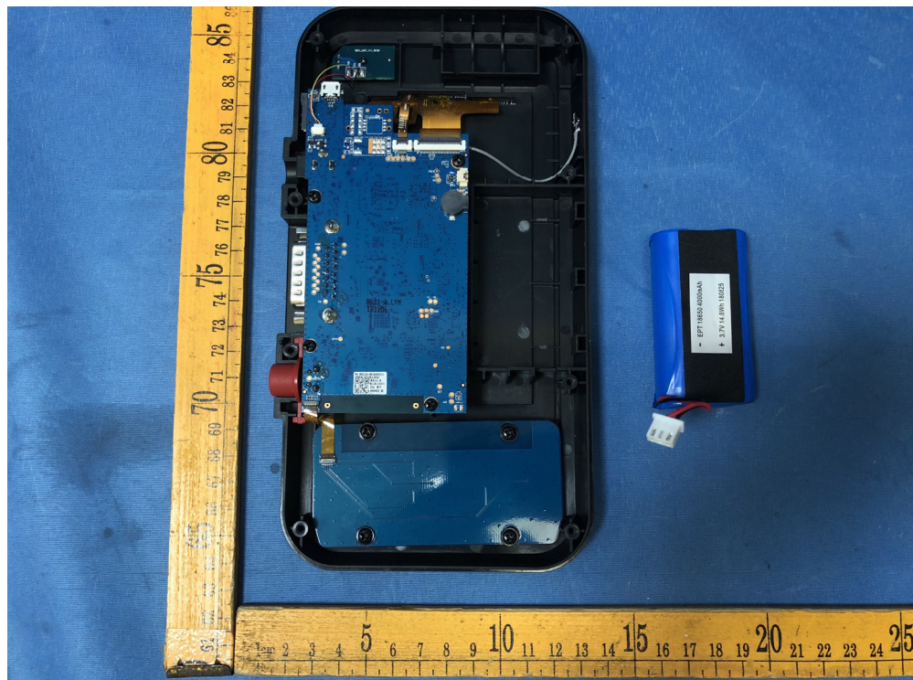
WIFI ANT.
