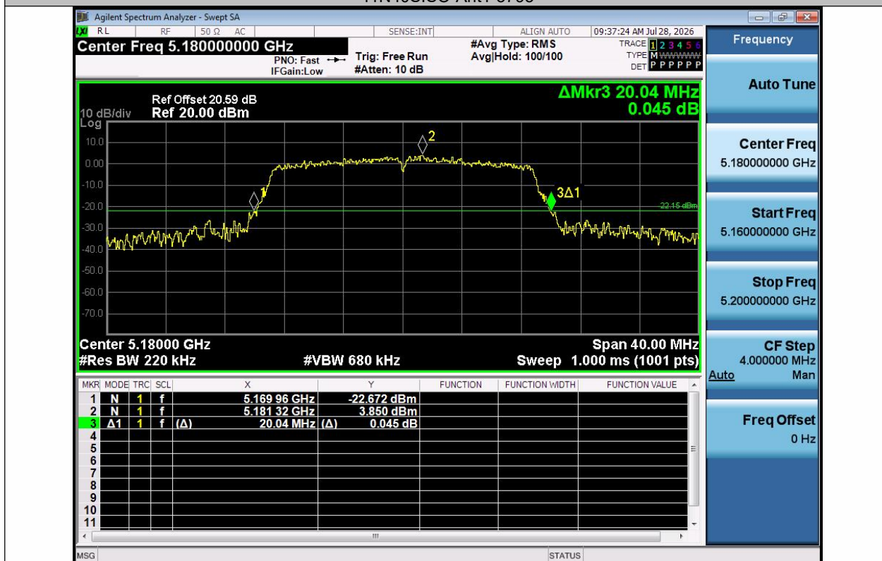
11AC20SISO-Ant1-5180
