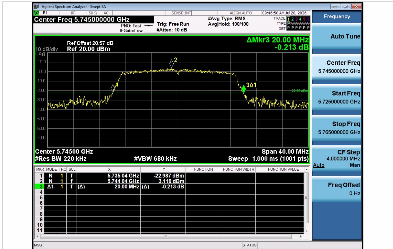
11AC20SISO-Ant1-5745
