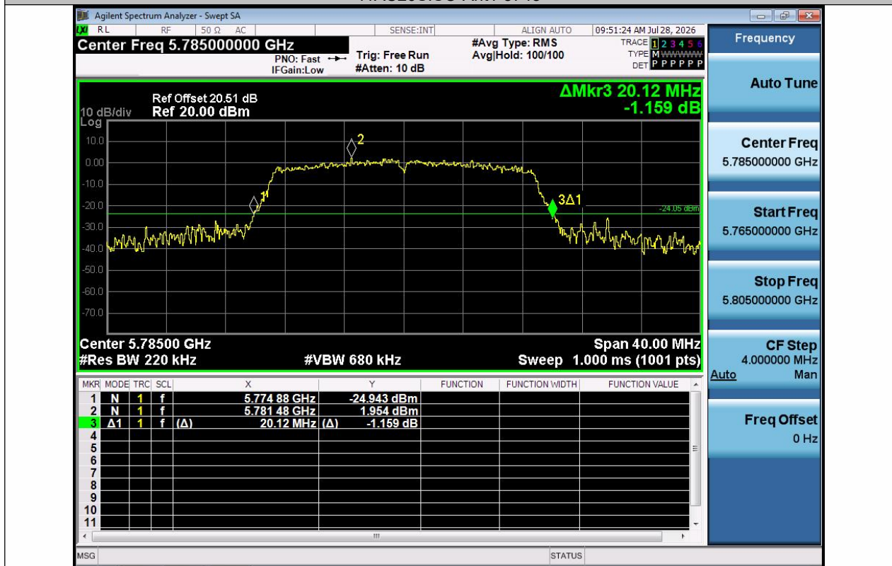
11AC20SISO-Ant1-5785
