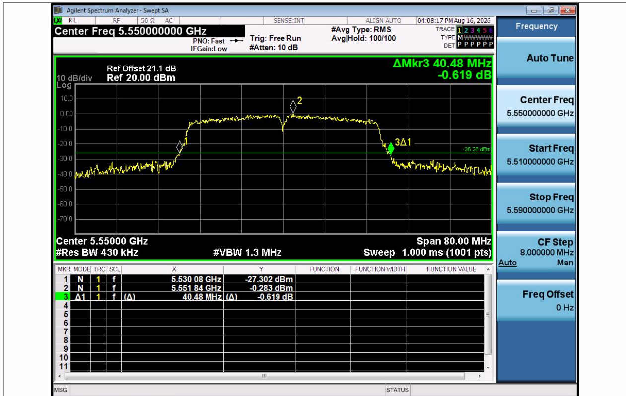
11AC40SISO-Ant1-5550
