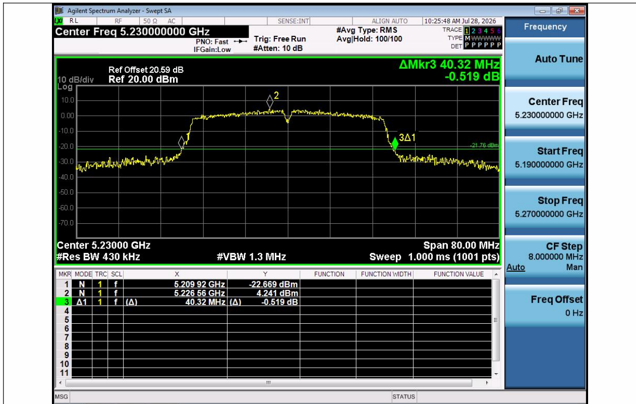
11AC40SISO-Ant1-5230
