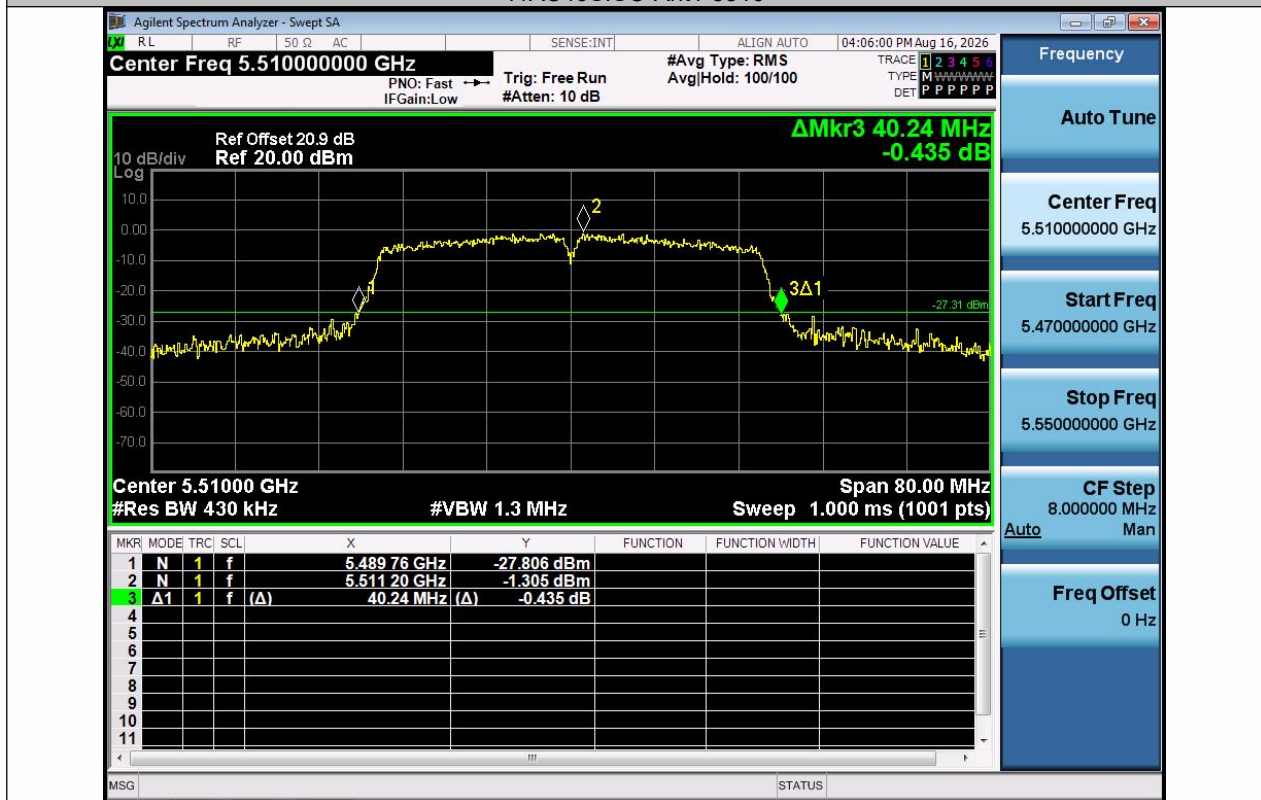
11AC40SISO-Ant1-5510
