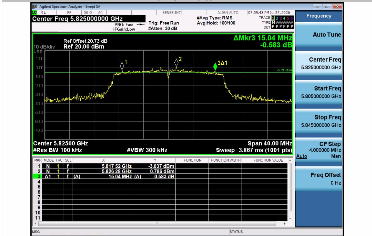
11N20SISO-Ant1-5825-PASS
