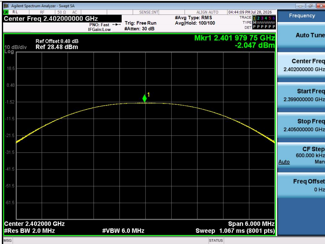
BLE_1M-Ant1-2402-PASS
