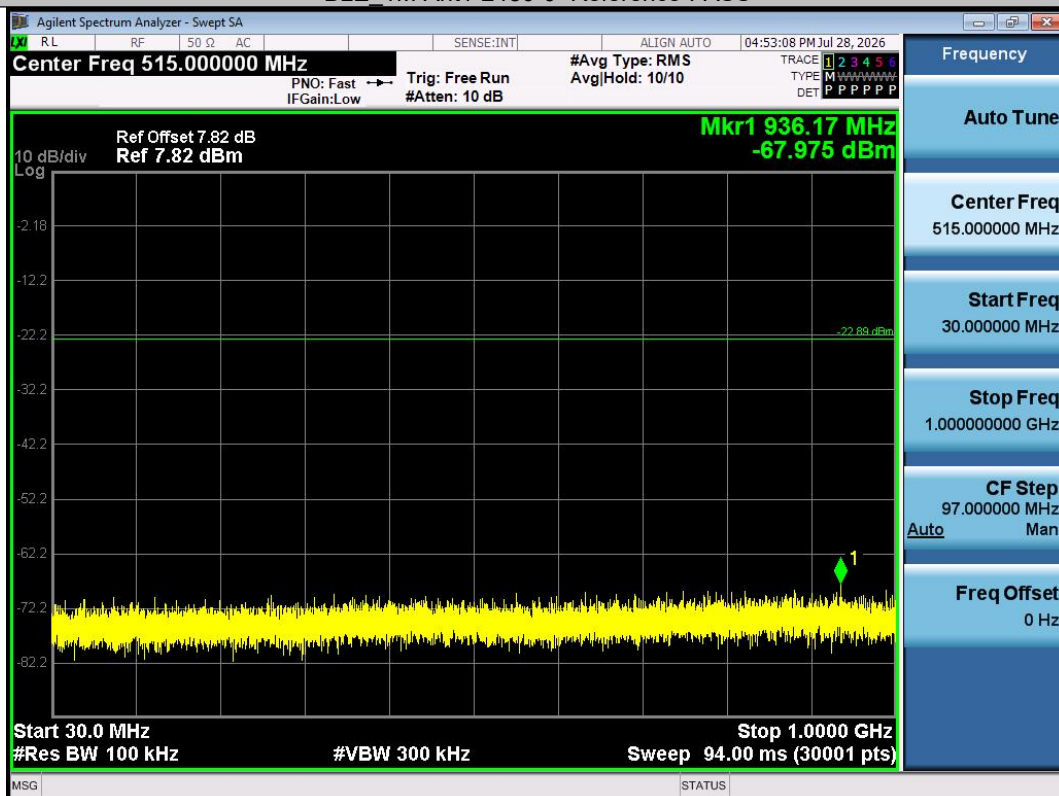
BLE_1M-Ant1-2480-30~1000-PASS
