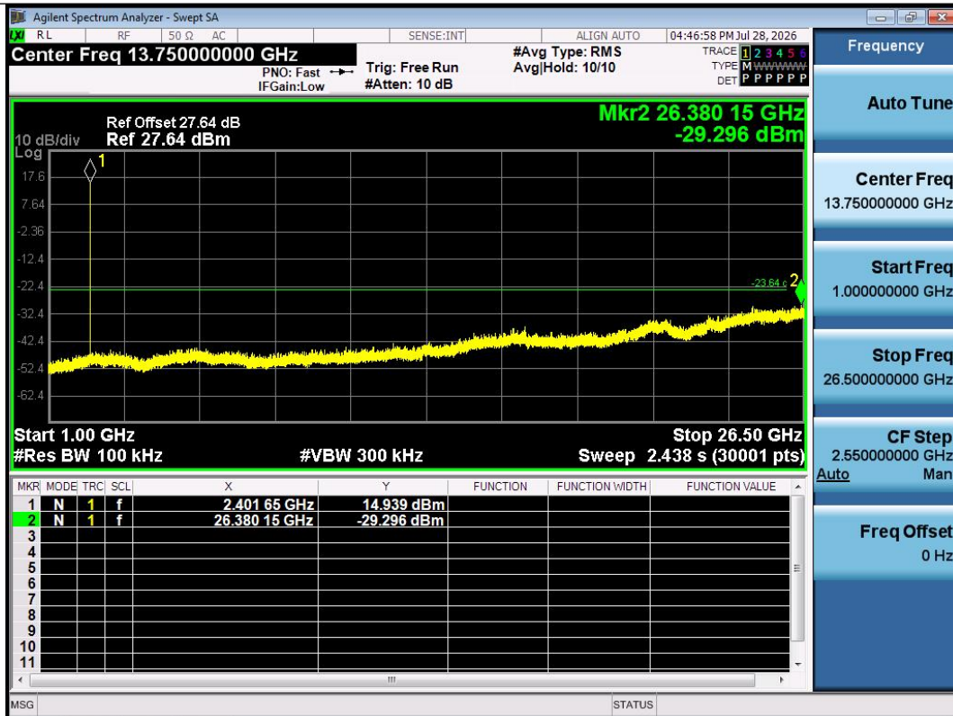
BLE_1M-Ant1-2402-1000~26500-PASS
