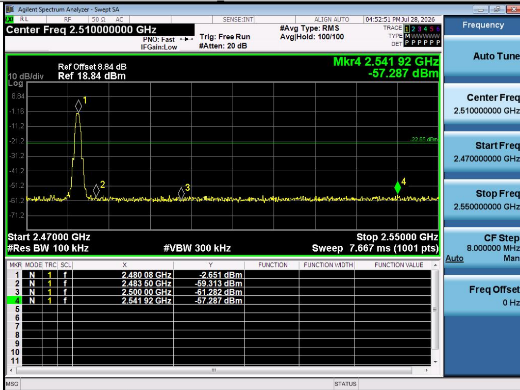
BLE_1M-Ant1-2480-PASS
