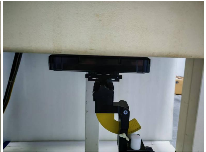
Fig-4.2 Rear Face of EUT with 0 cm Gap (Head Mode)
