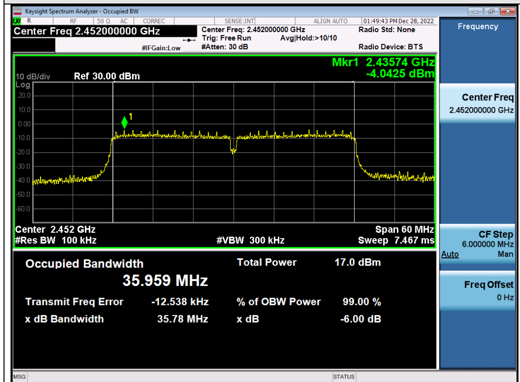
Test Graph 802.11n40 ANT1 2452 MCS0 DTSBW
