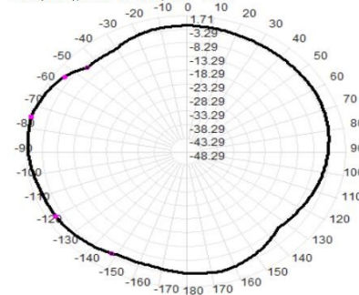
Total(H-XY), Max= 1.71dBi, CirD=10.02
