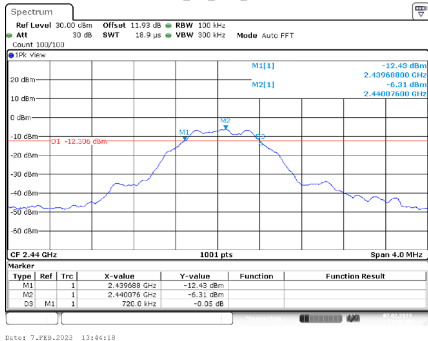
BLE_1M_Ant1_2440
