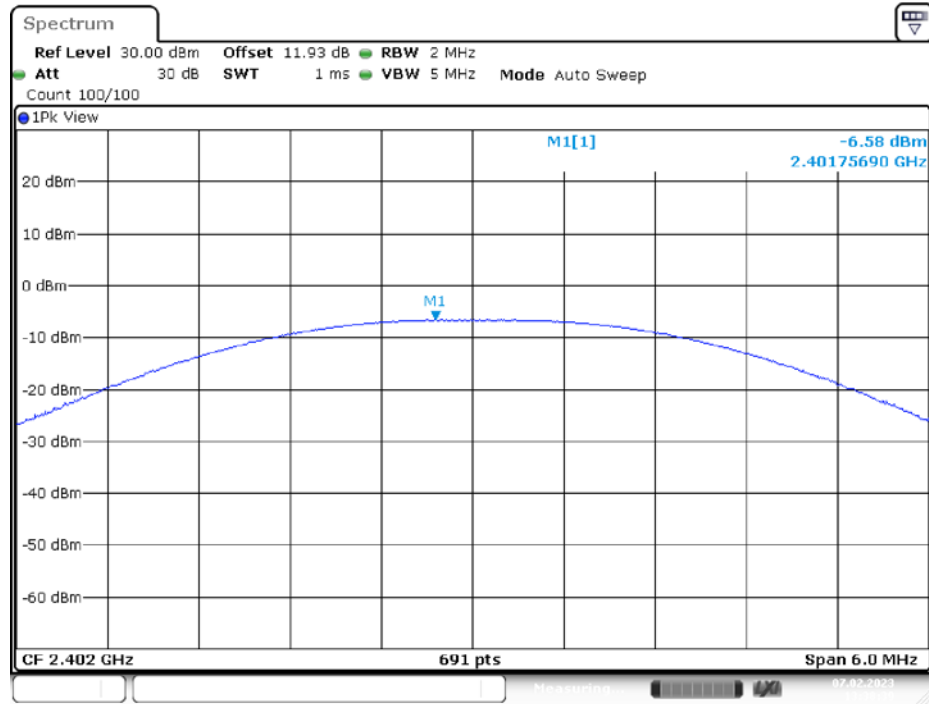
BLE_1M_Ant1_2402
