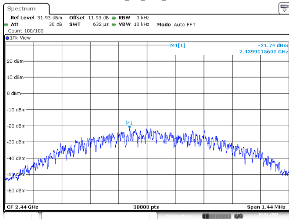
BLE_1M_Ant1_2440
