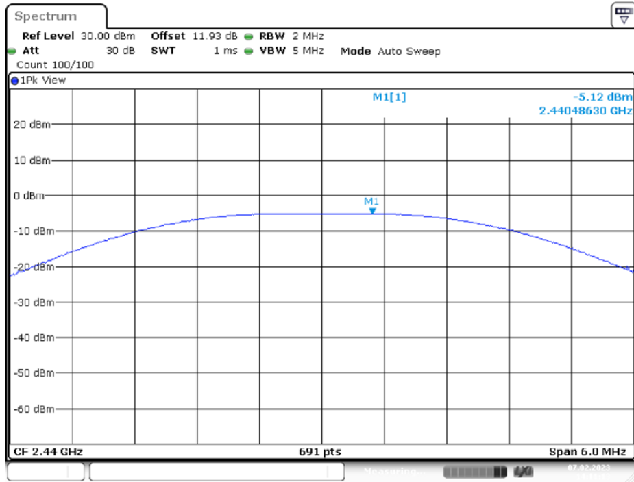
BLE_2M_Ant1_2440
