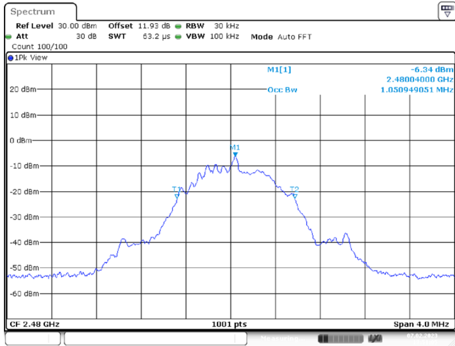
BLE_1M_Ant1_2480
