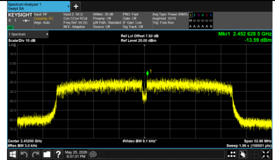
IEEE 802.11n_Channel 9_40MHz_Antenna 0
