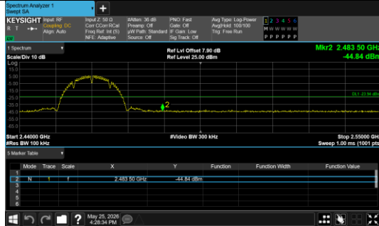
Out Of Band Emission IEEE 802.11b_Channel 11_20MHz_Antenna 0
