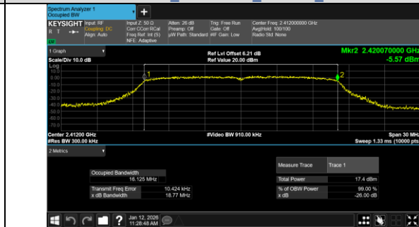
IEEE 802.11g_Channel 1_20MHz_Antenna 0
