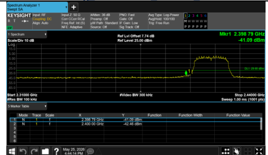
Out Of Band Emission IEEE 802.11n_Channel 1_20MHz_Antenna 0
