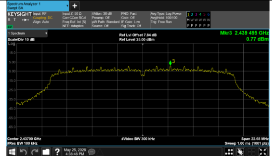
In-Band Reference Level IEEE 802.11g_Channel 6_20MHz_Antenna 0
