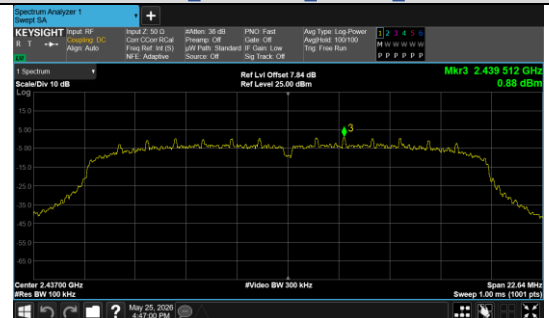
In-Band Reference Level IEEE 802.11n_Channel 6_20MHz_Antenna 0
