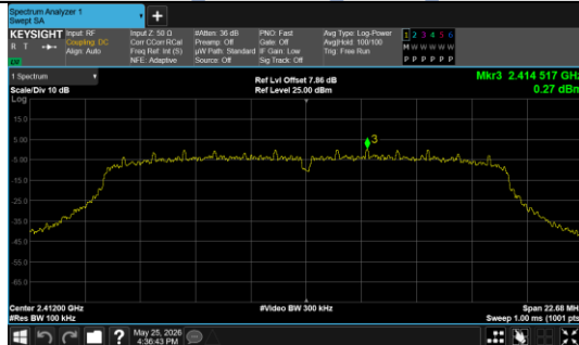
In-Band Reference Level IEEE 802.11g_Channel 1_20MHz_Antenna 0
