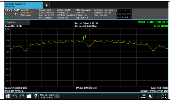
In-Band Reference Level IEEE 802.11b_Channel 11_20MHz_Antenna 0
