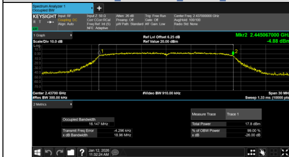
IEEE 802.11g_Channel 6_20MHz_Antenna 0
