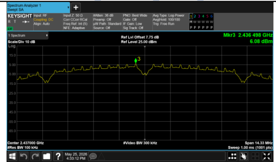
In-Band Reference Level IEEE 802.11b_Channel 6_20MHz_Antenna 0
