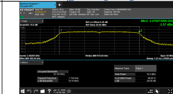
IEEE 802.11g_Channel 11_20MHz_Antenna 0
