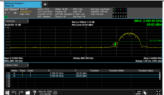
Out Of Band Emission IEEE 802.11b_Channel 1_20MHz_Antenna 0
