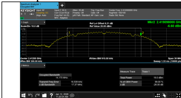
IEEE 802.11b_Channel 1_20MHz_Antenna 0
