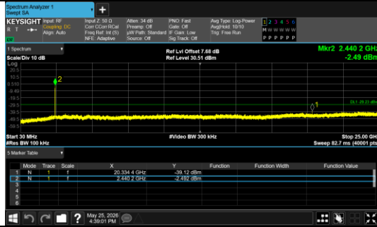
30.0 MHz - 25000.0 MHz IEEE 802.11g_Channel 6_20MHz_Antenna 0
