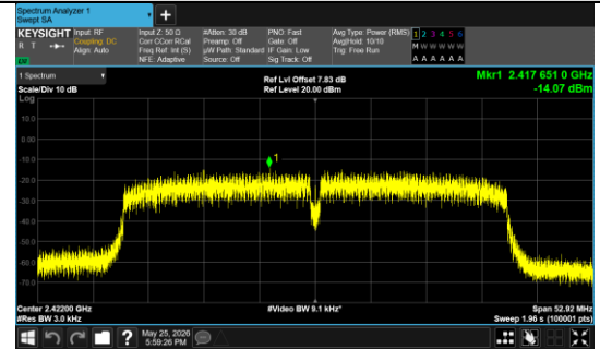
IEEE 802.11n_Channel 3_40MHz_Antenna 0
