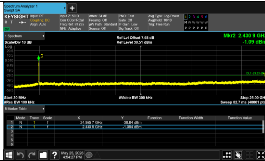
30.0 MHz - 25000.0 MHz IEEE 802.11n_Channel 6_40MHz_Antenna 0
