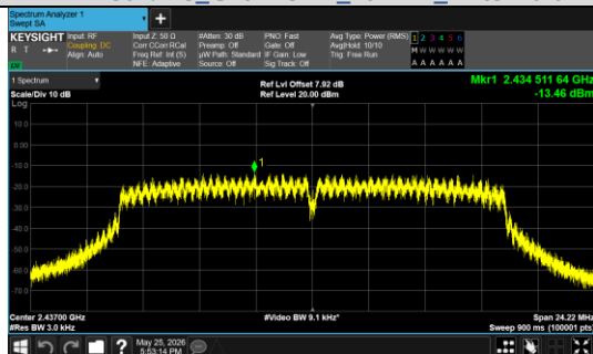
IEEE 802.11g_Channel 6_20MHz_Antenna 0
