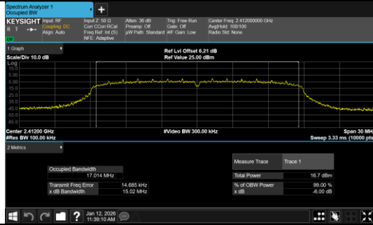
IEEE 802.11n_Channel 1_20MHz_Antenna 0
