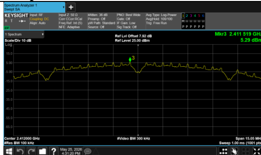
In-Band Reference Level IEEE 802.11b_Channel 1_20MHz_Antenna 0
