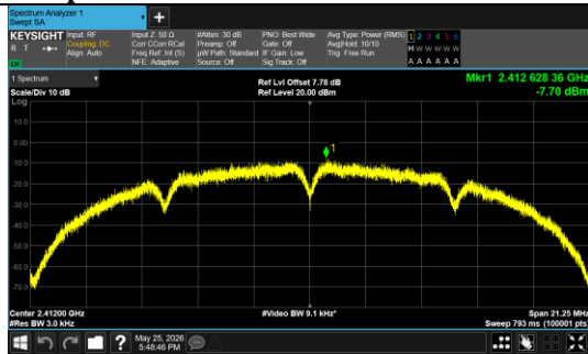
IEEE 802.11b_Channel 1_20MHz_Antenna 0
