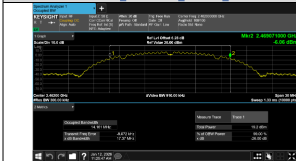
IEEE 802.11b_Channel 11_20MHz_Antenna 0
