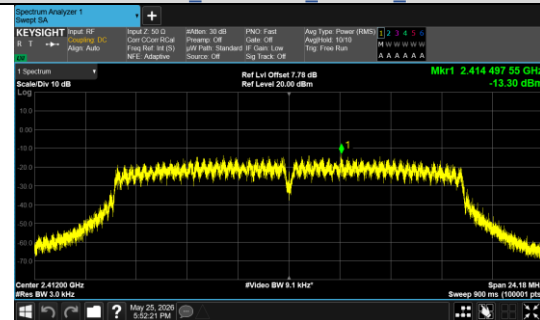
IEEE 802.11g_Channel 1_20MHz_Antenna 0
