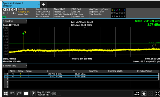
30.0 MHz - 25000.0 MHz IEEE 802.11b_Channel 1_20MHz_Antenna 0
