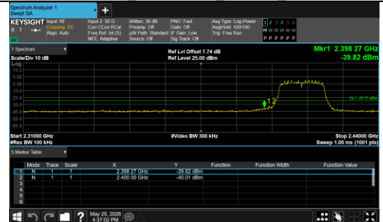
Out Of Band Emission IEEE 802.11g_Channel 1_20MHz_Antenna 0
