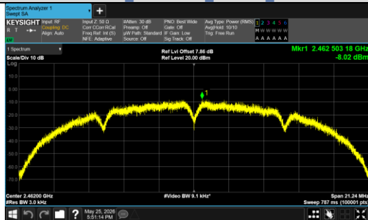
IEEE 802.11b_Channel 11_20MHz_Antenna 0
