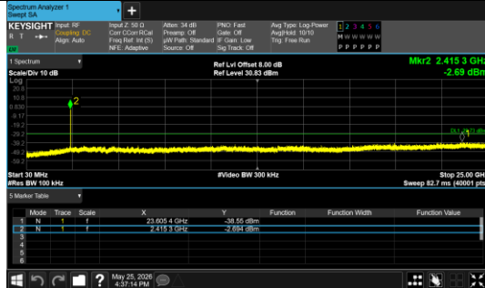
30.0 MHz - 25000.0 MHz IEEE 802.11g_Channel 1_20MHz_Antenna 0
