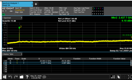
30.0 MHz - 25000.0 MHz IEEE 802.11b_Channel 6_20MHz_Antenna 0
