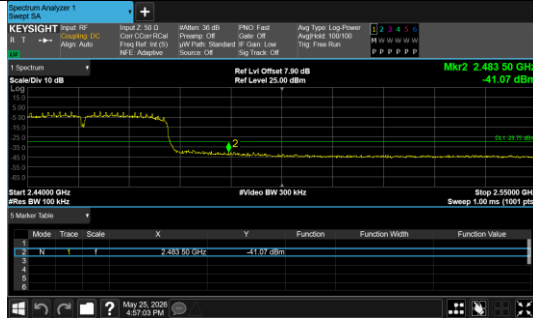
Out Of Band Emission IEEE 802.11n_Channel 9_40MHz_Antenna 0
