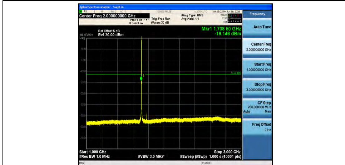
Band4-1.4MHz-16QAM-19957-1RB#0-1000~3000-PASS
