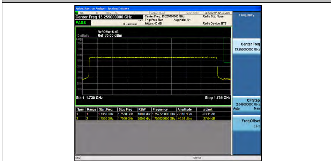
Band4-20MHz-16QAM-20300-100RB#0-PASS
