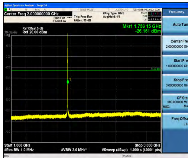
Band4-1.4MHz-16QAM-20393-1RB#0-1000~3000-PASS
