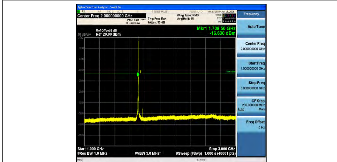
Band4-3MHz-QPSK-19965-1RB#0-1000~3000-PASS
