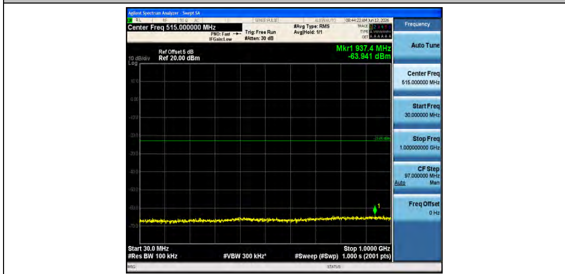
Band4-1.4MHz-16QAM-19957-1RB#0-30~1000-PASS
