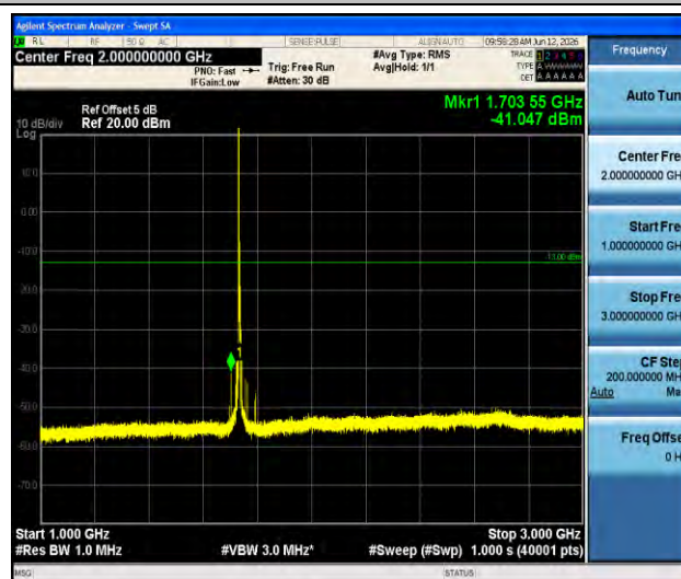
Band4-5MHz-16QAM-20175-1RB#0-1000~3000-PASS
