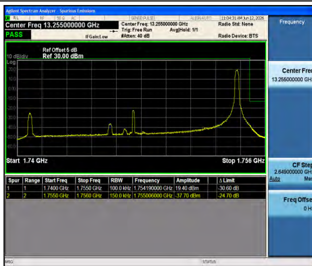
Band4-15MHz-QPSK-20325-1RB#74-PASS
