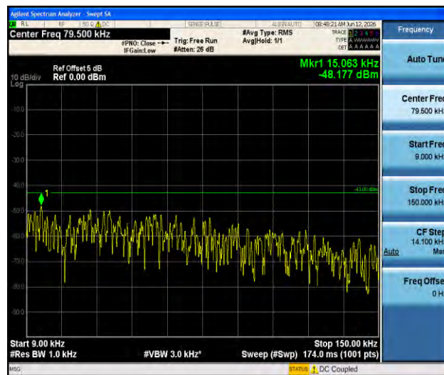
Band4-1.4MHz-16QAM-20393-1RB#0-0.009~0.15-PASS
