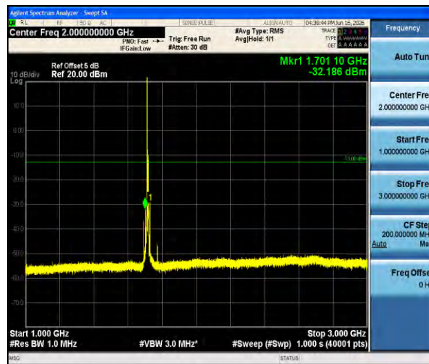
Band4-10MHz-QPSK-20000-1RB#0-1000~3000-PASS
