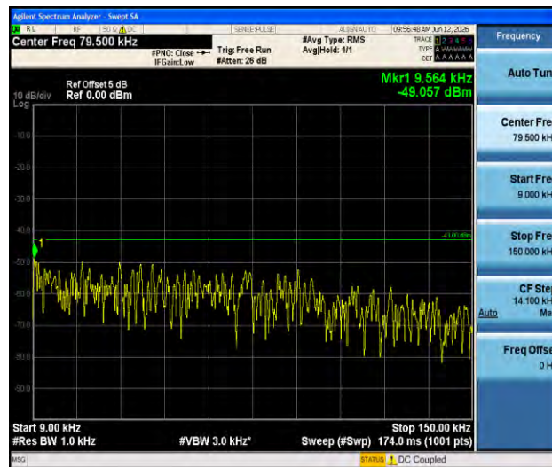
Band4-5MHz-QPSK-20175-1RB#0-0.009~0.15-PASS
