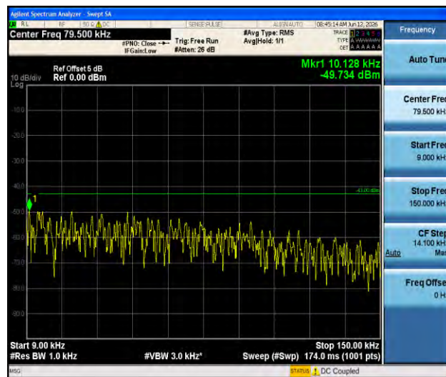
Band4-1.4MHz-QPSK-20175-1RB#0-0.009~0.15-PASS
