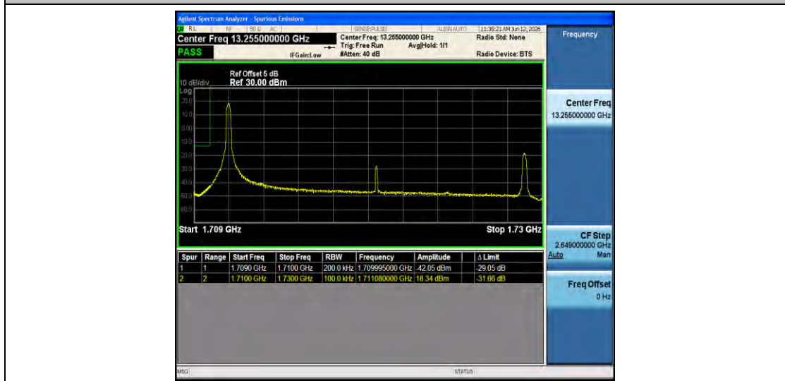
Band4-20MHz-16QAM-20050-1RB#0-PASS
