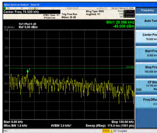
Band4-3MHz-QPSK-19965-1RB#0-0.009~0.15-PASS
