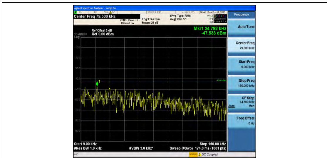
Band4-1.4MHz-16QAM-20175-1RB#0-0.009~0.15-PASS
