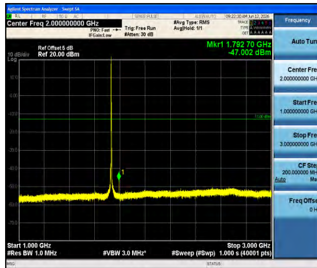
Band4-3MHz-16QAM-20175-1RB#0-1000~3000-PASS
