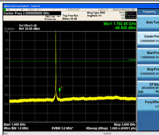
Band4-3MHz-QPSK-20175-1RB#0-1000~3000-PASS
