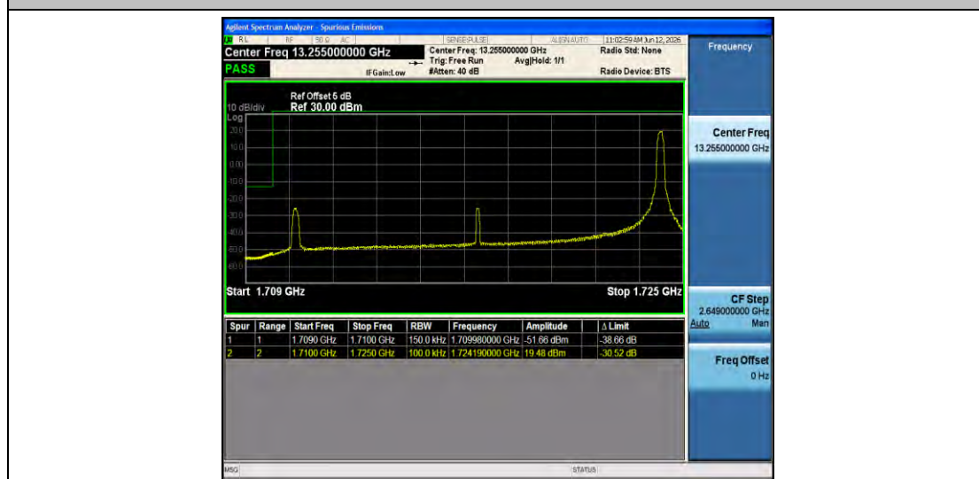
Band4-15MHz-QPSK-20025-1RB#74-PASS
