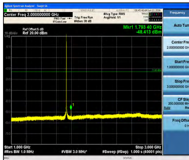
Band4-1.4MHz-QPSK-20175-1RB#0-1000~3000-PASS
