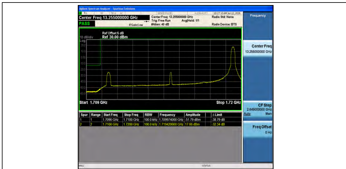
Band4-10MHz-16QAM-20000-1RB#49-PASS
