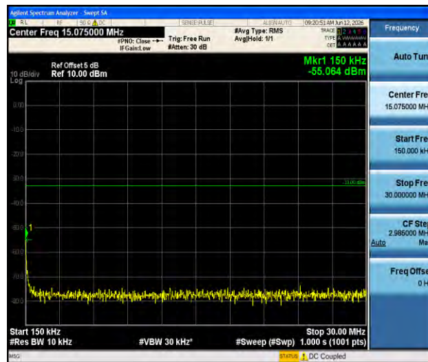
Band4-3MHz-QPSK-20175-1RB#0-0.15~30-PASS
