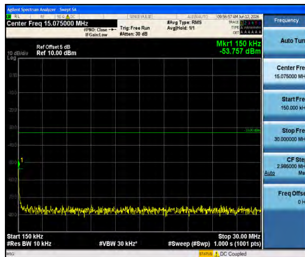
Band4-5MHz-QPSK-20175-1RB#0-0.15~30-PASS
