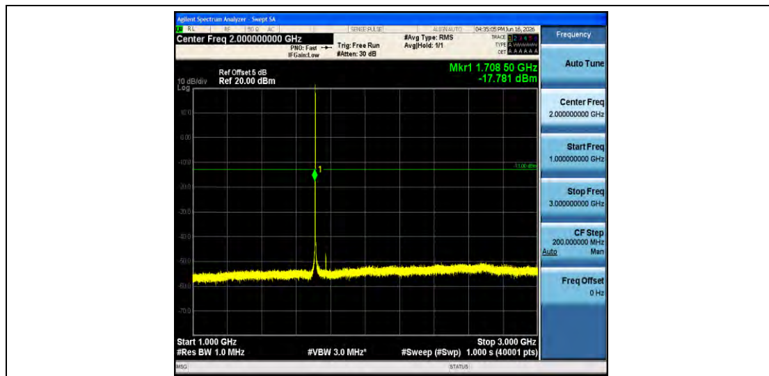
Band4-1.4MHz-QPSK-19957-1RB#0-1000~3000-PASS
