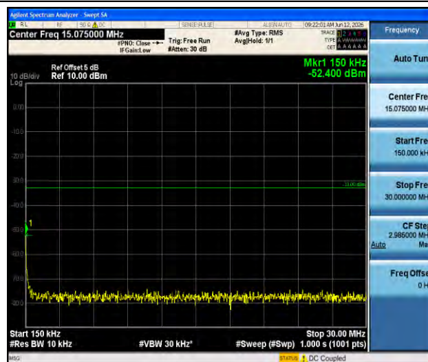
Band4-3MHz-16QAM-20175-1RB#0-0.15~30-PASS
