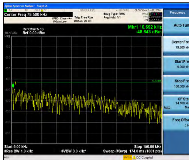
Band4-5MHz-QPSK-20375-1RB#0-0.009~0.15-PASS
