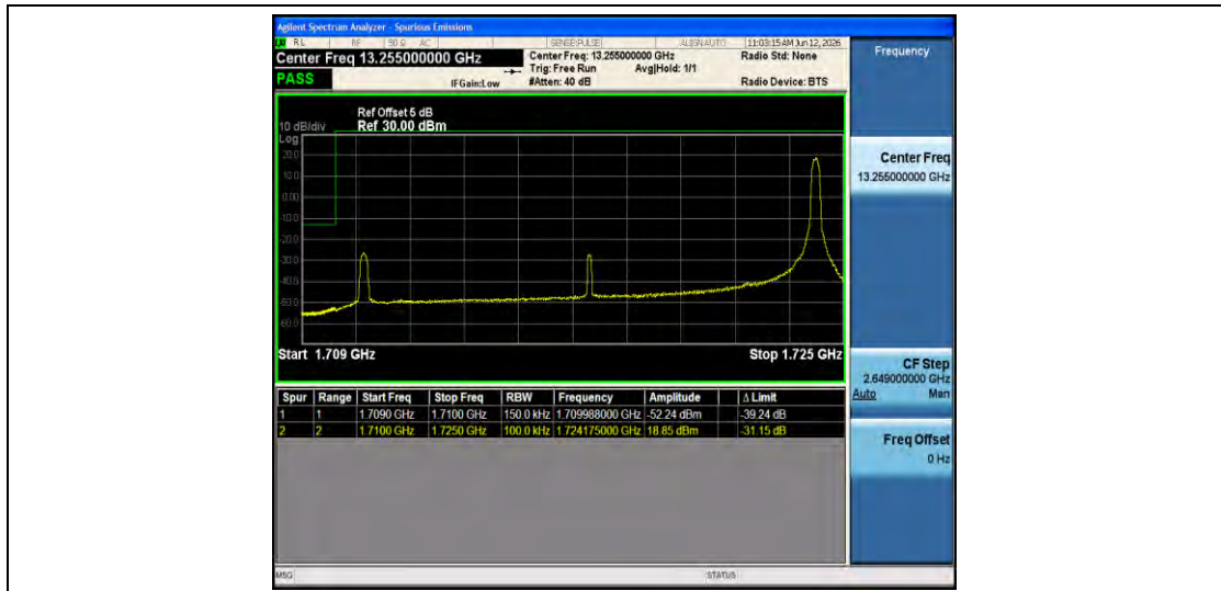
Band4-15MHz-16QAM-20025-1RB#74-PASS
