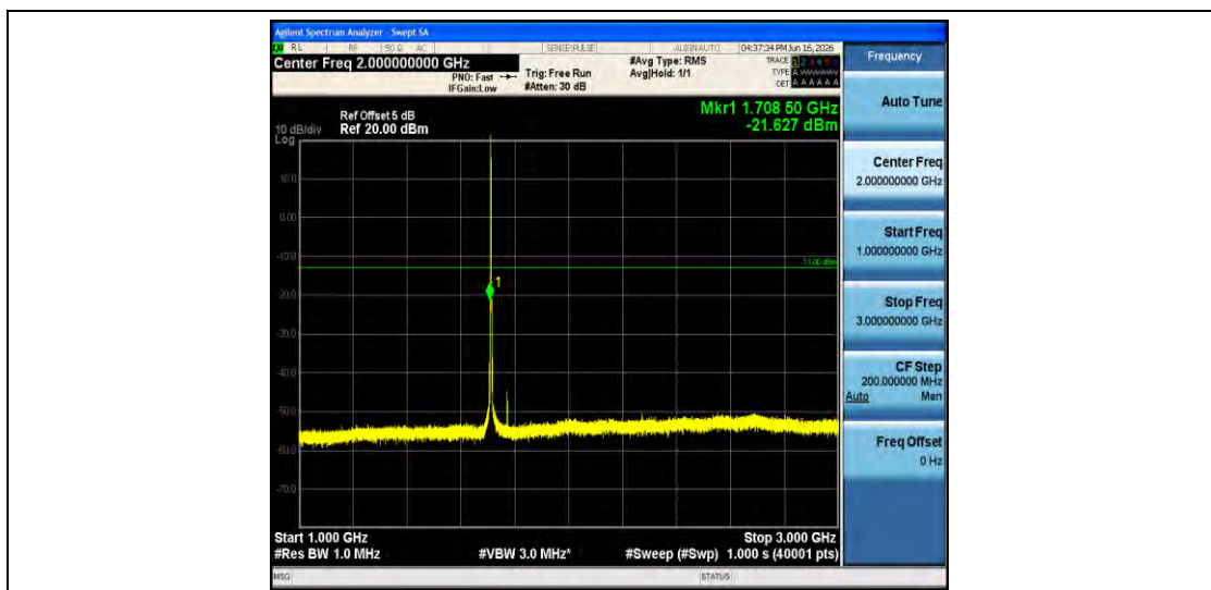
Band4-3MHz-16QAM-19965-1RB#0-1000~3000-PASS
