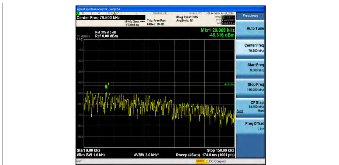
Band4-1.4MHz-16QAM-19957-1RB#0-0.009~0.15-PASS
