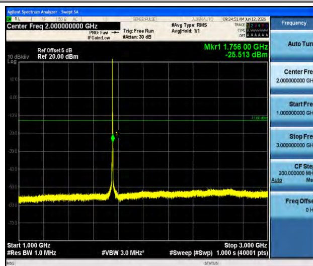
Band4-3MHz-16QAM-20385-1RB#0-1000~3000-PASS
