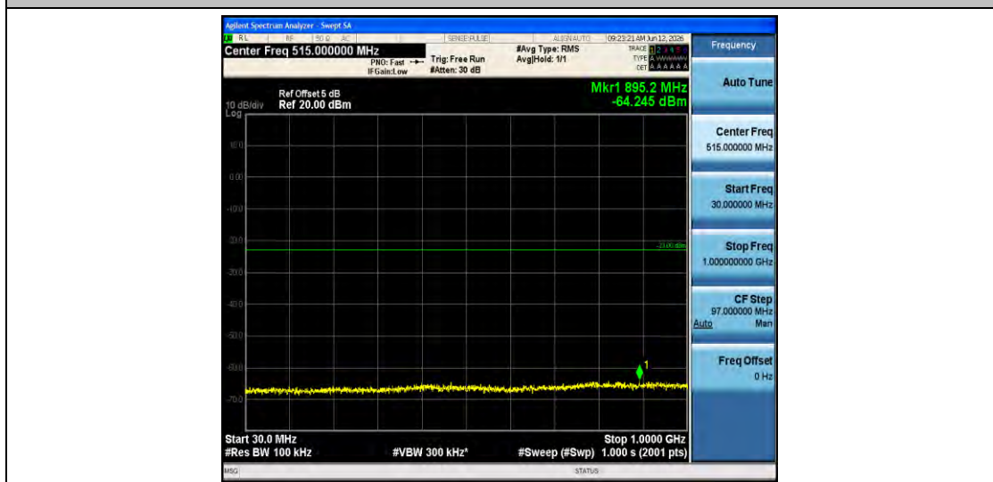
Band4-3MHz-QPSK-20385-1RB#0-30~1000-PASS
