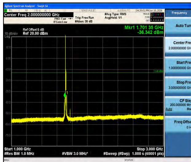
Band4-10MHz-16QAM-20000-1RB#0-1000~3000-PASS
