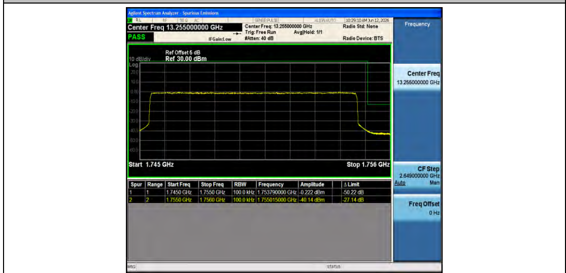
Band4-10MHz-16QAM-20350-50RB#0-PASS
