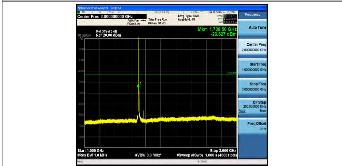
Band4-5MHz-16QAM-19975-1RB#0-1000~3000-PASS
