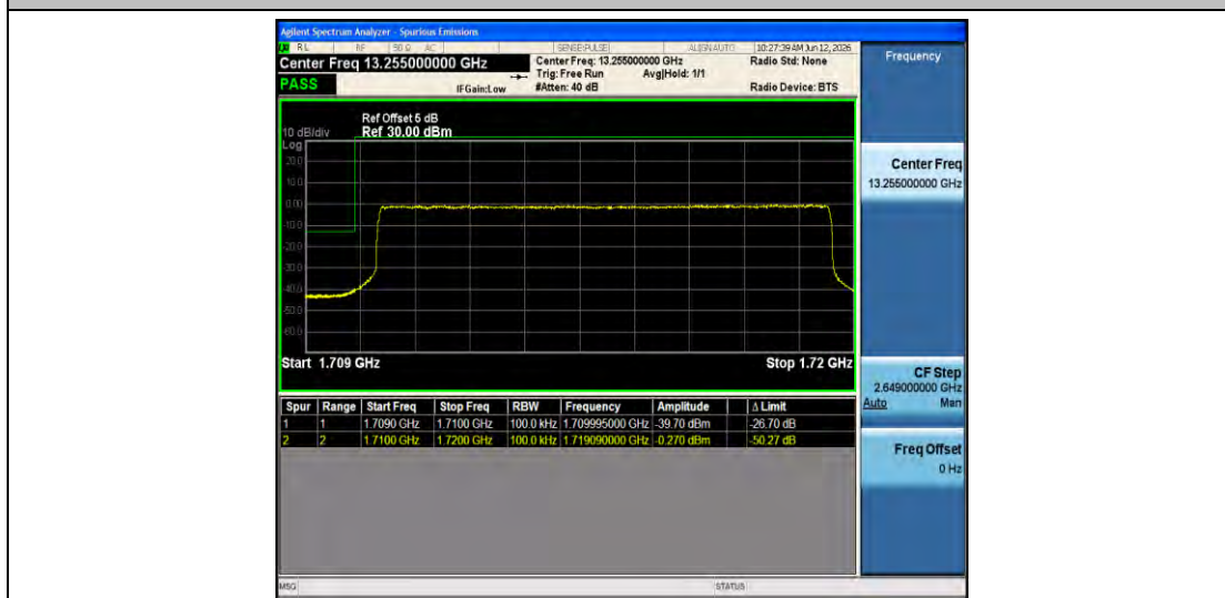
Band4-10MHz-16QAM-20000-50RB#0-PASS
