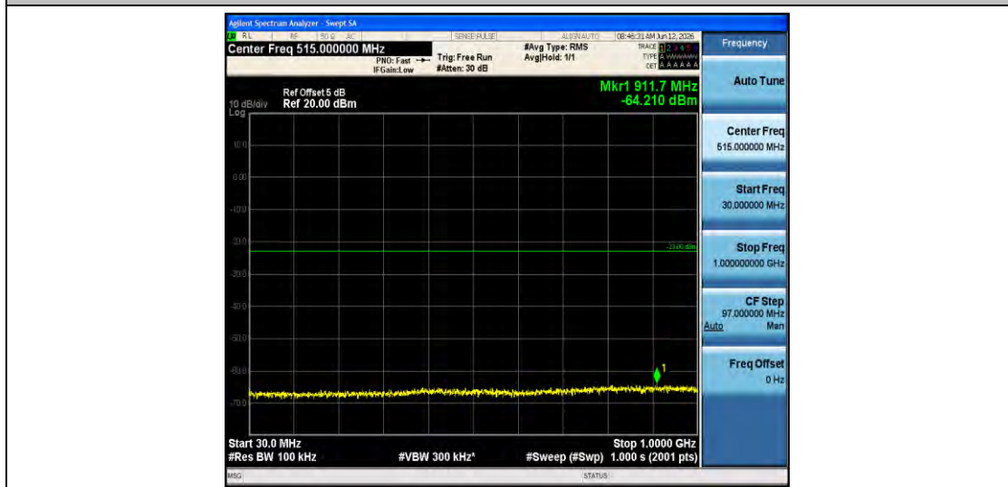
Band4-1.4MHz-16QAM-20175-1RB#0-30~1000-PASS
