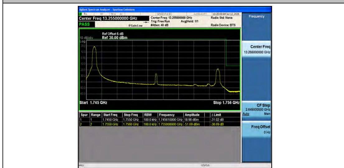
Band4-10MHz-16QAM-20350-1RB#0-PASS
