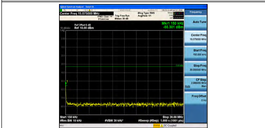
Band4-3MHz-QPSK-20385-1RB#0-0.15~30-PASS
