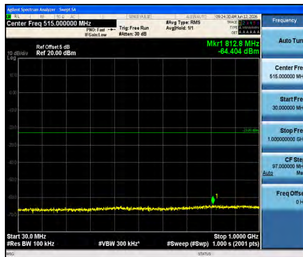
Band4-3MHz-16QAM-20385-1RB#0-30~1000-PASS
