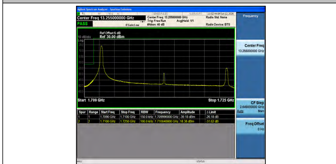
Band4-15MHz-16QAM-20025-1RB#0-PASS
