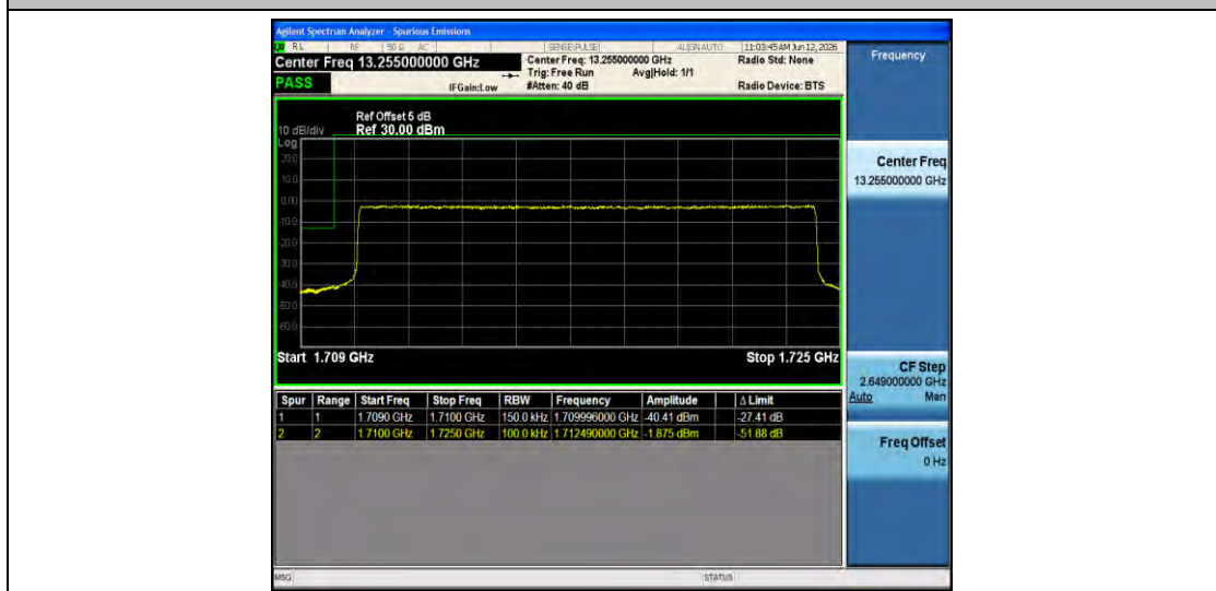
Band4-15MHz-16QAM-20025-75RB#0-PASS
