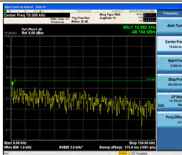
Band4-1.4MHz-QPSK-19957-1RB#0-0.009~0.15-PASS
