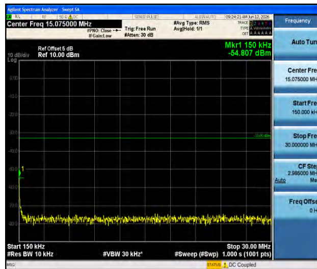
Band4-3MHz-16QAM-20385-1RB#0-0.15~30-PASS
