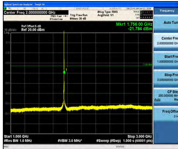
Band4-3MHz-QPSK-20385-1RB#0-1000~3000-PASS
