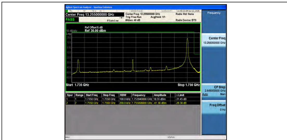
Band4-20MHz-16QAM-20300-1RB#99-PASS
