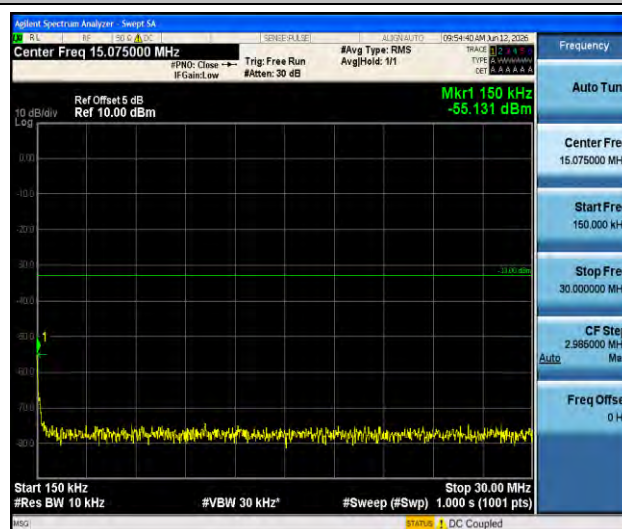
Band4-5MHz-QPSK-19975-1RB#0-0.15~30-PASS
