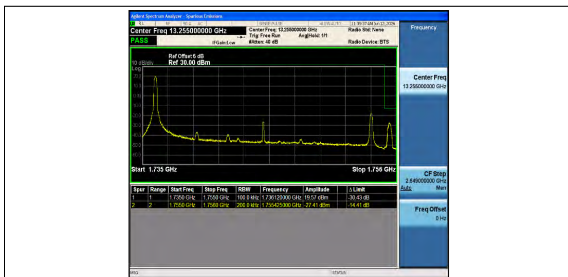
Band4-20MHz-QPSK-20300-1RB#0-PASS
