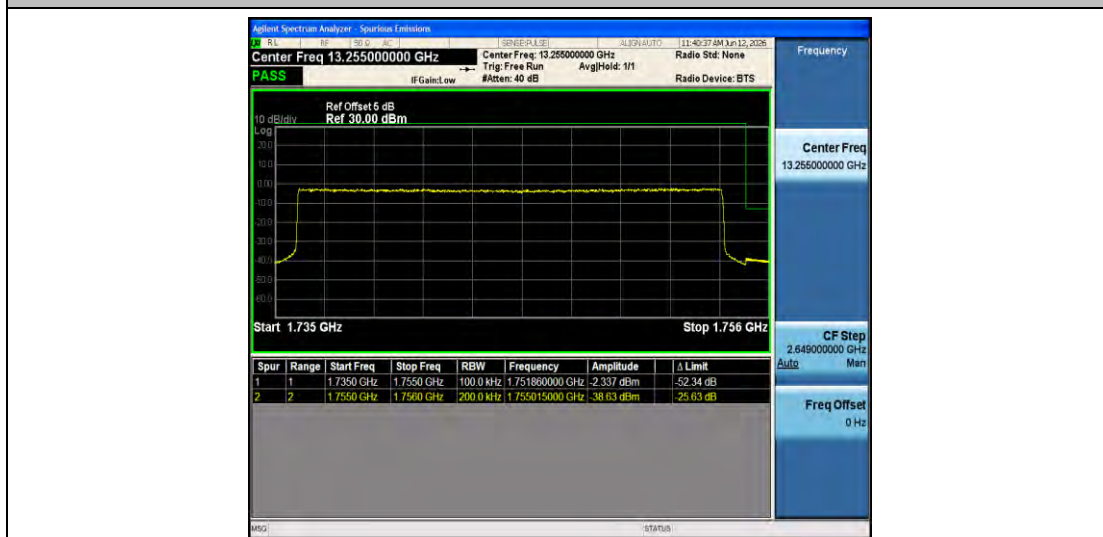
Band4-20MHz-QPSK-20300-100RB#0-PASS
