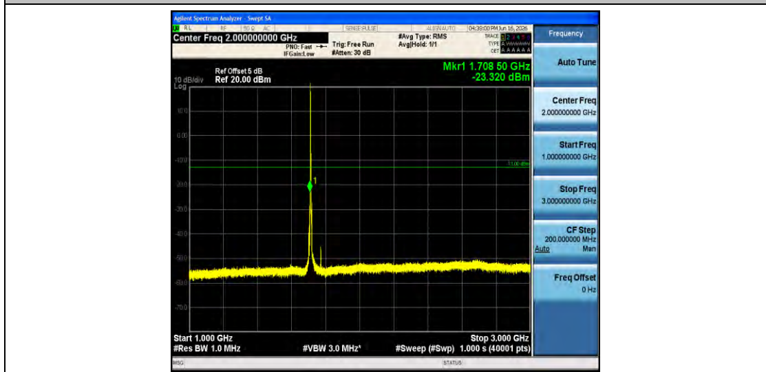
Band4-5MHz-QPSK-19975-1RB#0-1000~3000-PASS
