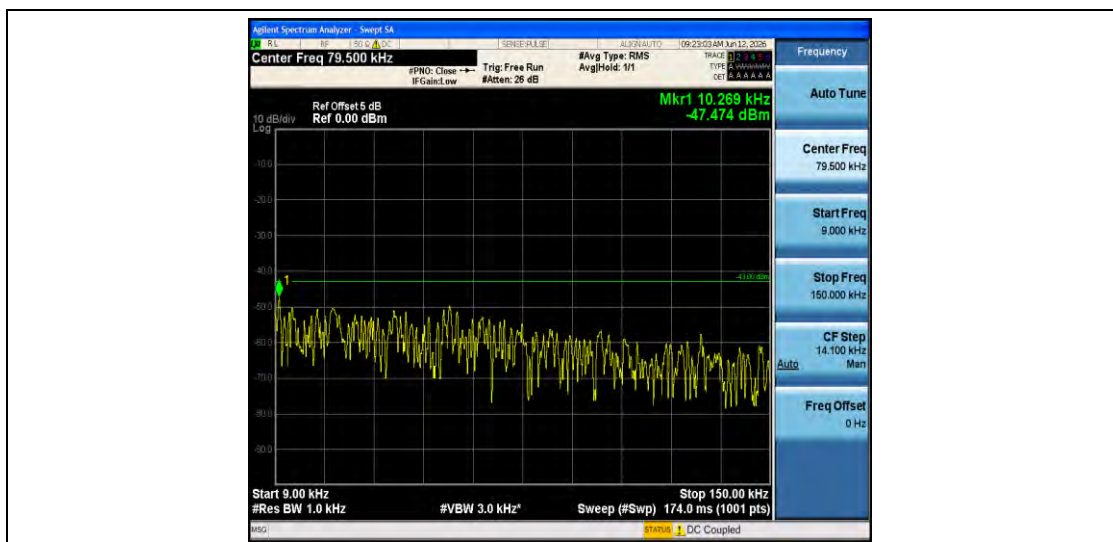
Band4-3MHz-QPSK-20385-1RB#0-0.009~0.15-PASS
