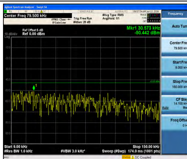
Band4-5MHz-16QAM-20175-1RB#0-0.009~0.15-PASS
