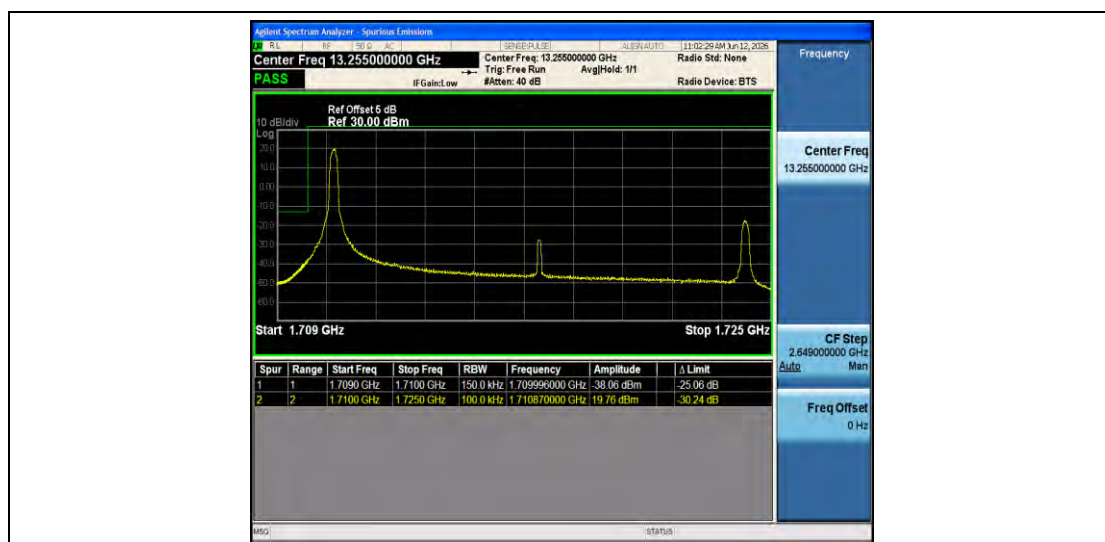
Band4-15MHz-QPSK-20025-1RB#0-PASS
