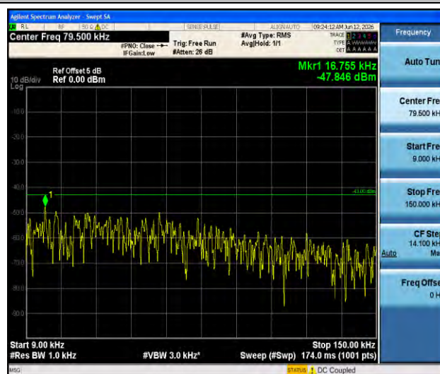
Band4-3MHz-16QAM-20385-1RB#0-0.009~0.15-PASS
