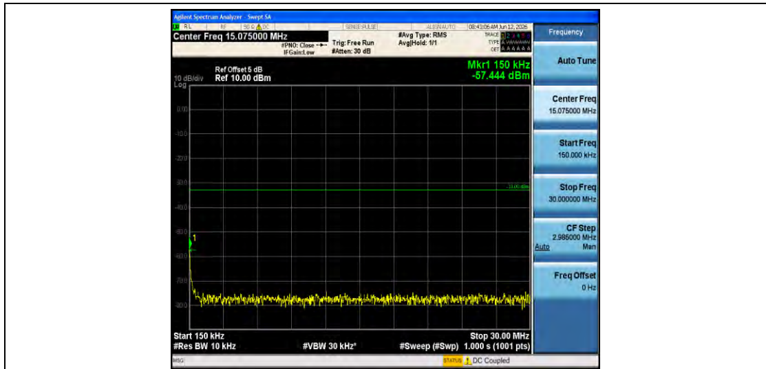
Band4-1.4MHz-QPSK-19957-1RB#0-0.15~30-PASS
