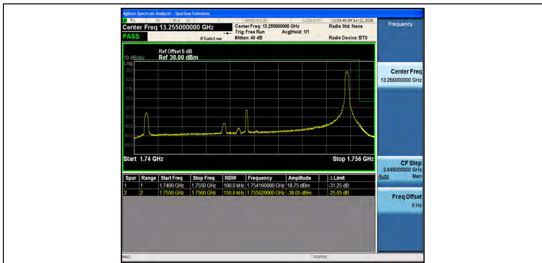
Band4-15MHz-16QAM-20325-1RB#74-PASS
