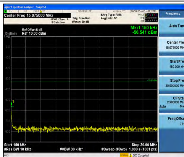
Band4-5MHz-QPSK-20375-1RB#0-0.15~30-PASS
