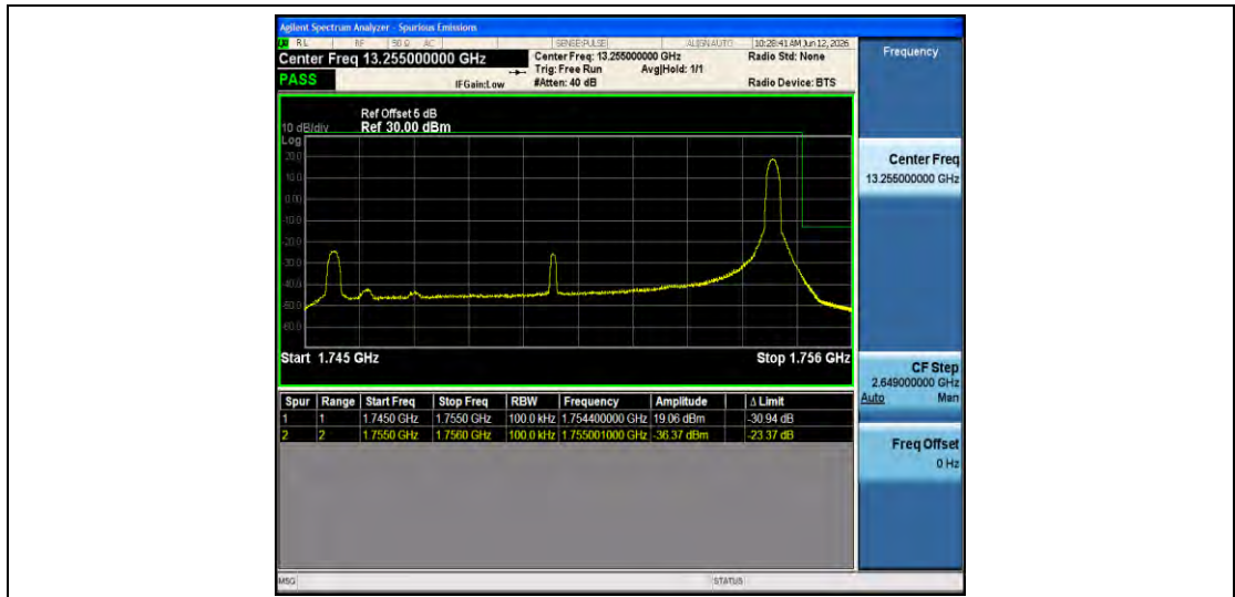
Band4-10MHz-16QAM-20350-1RB#49-PASS
