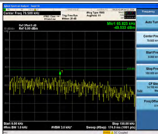
Band4-3MHz-QPSK-20175-1RB#0-0.009~0.15-PASS
