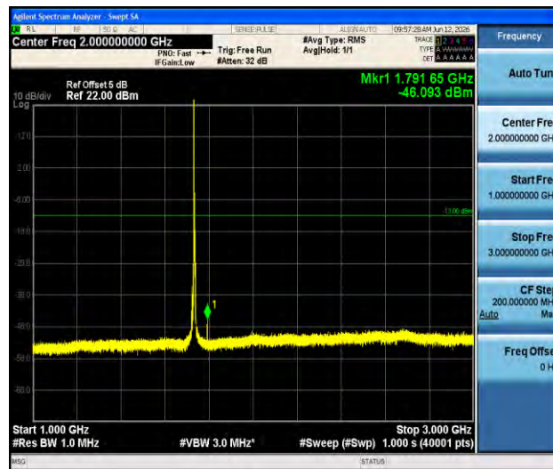
Band4-5MHz-QPSK-20175-1RB#0-1000~3000-PASS
