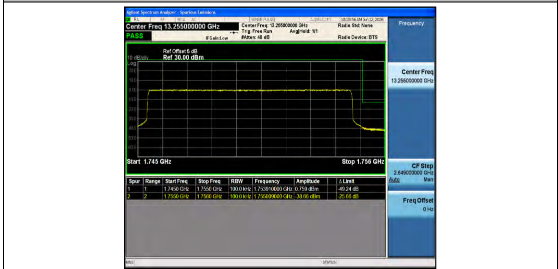
Band4-10MHz-QPSK-20350-50RB#0-PASS
