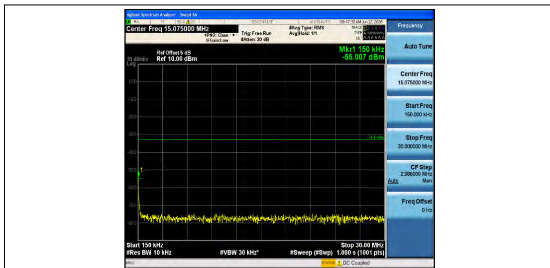
Band4-1.4MHz-QPSK-20393-1RB#0-0.15~30-PASS
