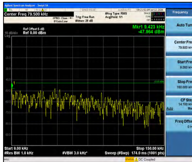
Band4-3MHz-16QAM-20175-1RB#0-0.009~0.15-PASS
