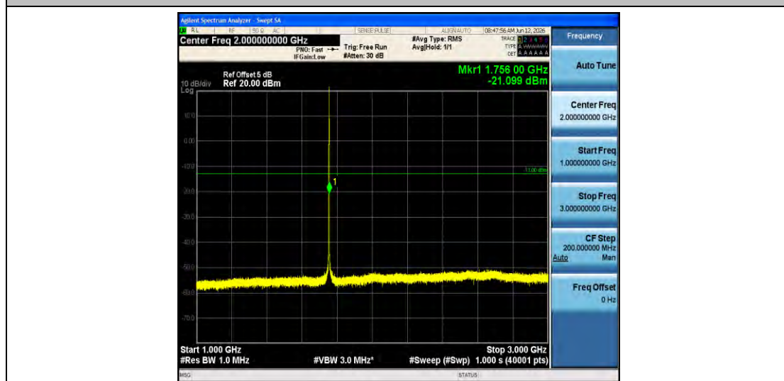
Band4-1.4MHz-QPSK-20393-1RB#0-1000~3000-PASS
