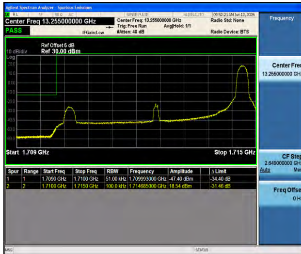
Band4-5MHz-16QAM-19975-1RB#24-PASS
