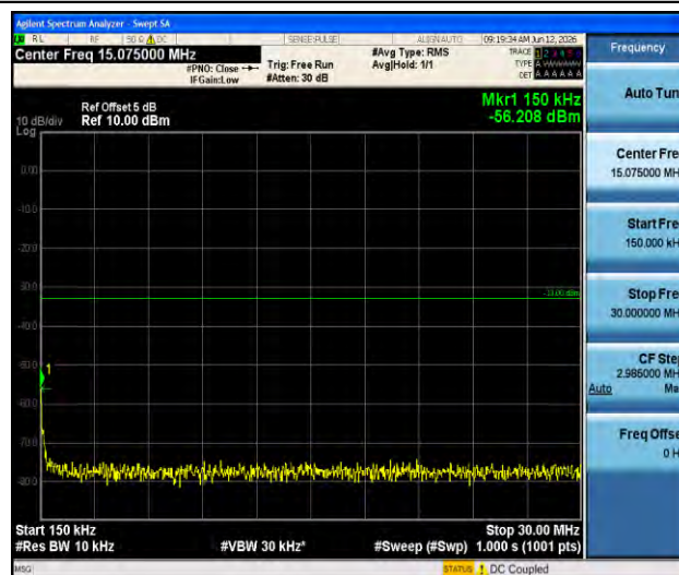
Band4-3MHz-16QAM-19965-1RB#0-0.15~30-PASS
