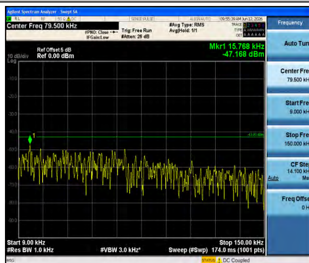
Band4-5MHz-16QAM-19975-1RB#0-0.009~0.15-PASS
