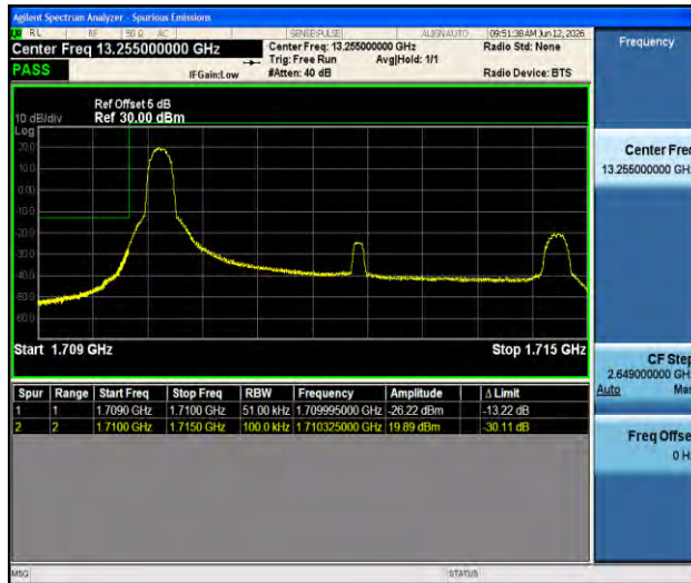
Band4-5MHz-QPSK-19975-1RB#0-PASS
