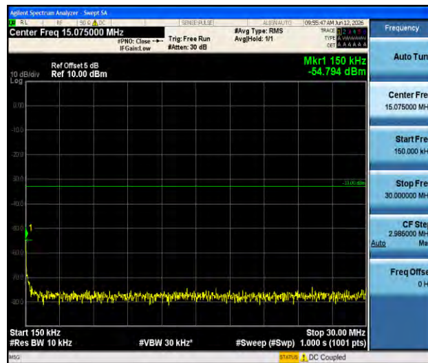
Band4-5MHz-16QAM-19975-1RB#0-0.15~30-PASS
