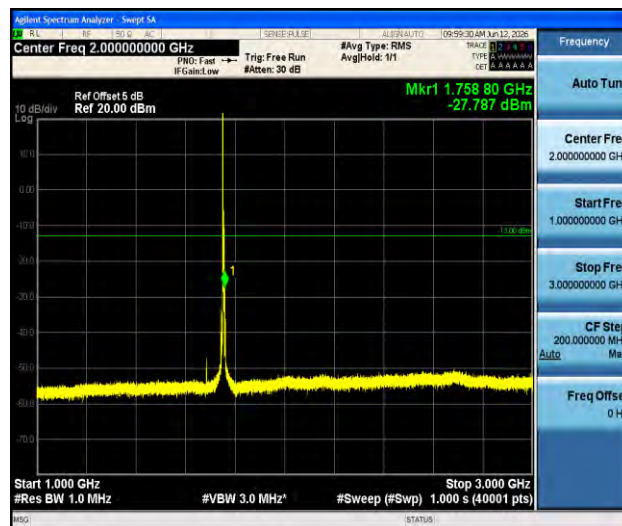
Band4-5MHz-QPSK-20375-1RB#0-1000~3000-PASS
