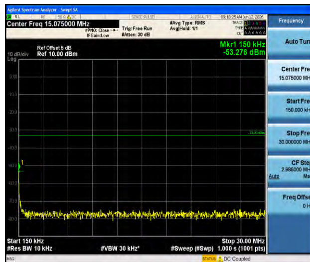
Band4-3MHz-QPSK-19965-1RB#0-0.15~30-PASS
