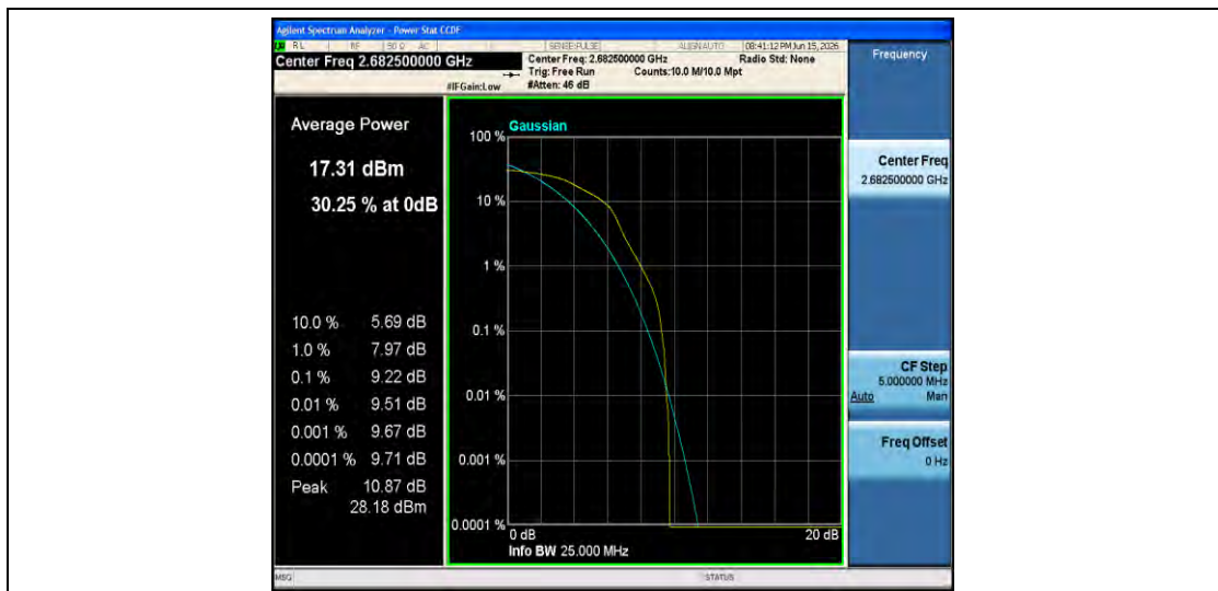
Band41-15MHz-16QAM-41515-1RB#0-PASS
