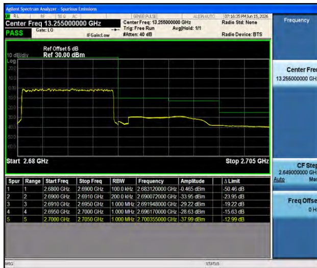
Band41-10MHz-QPSK-41540-50RB#0-PASS
