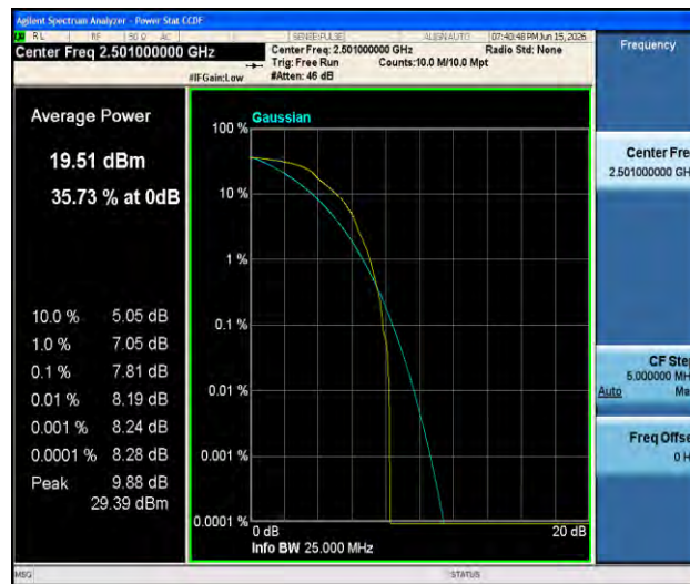
Band41-10MHz-QPSK-39700-1RB#0-PASS
