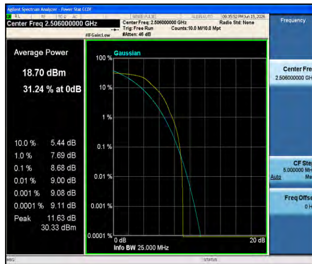
Band41-20MHz-QPSK-39750-1RB#0-PASS
