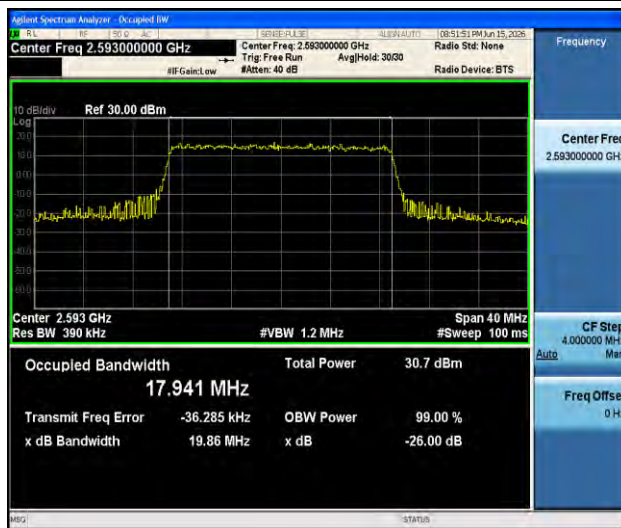
Band41-20MHz-QPSK-40620-100RB#0-PASS
