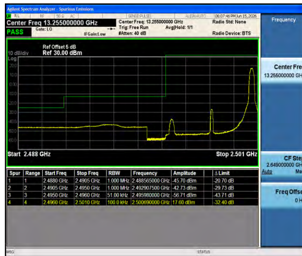
Band41-5MHz-16QAM-39675-1RB#24-PASS
