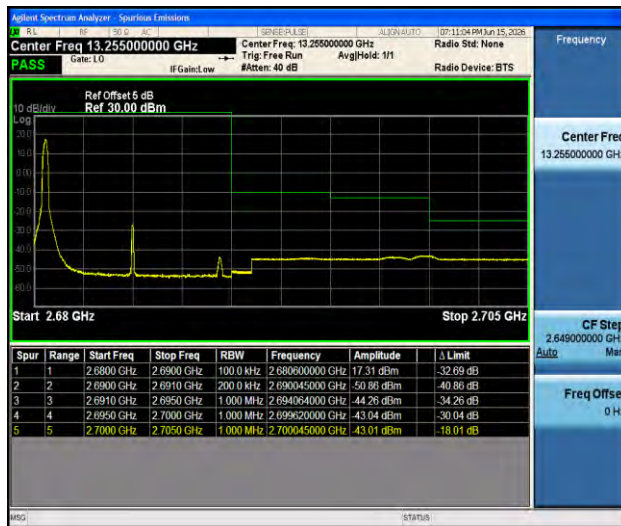
Band41-10MHz-16QAM-41540-1RB#0-PASS
