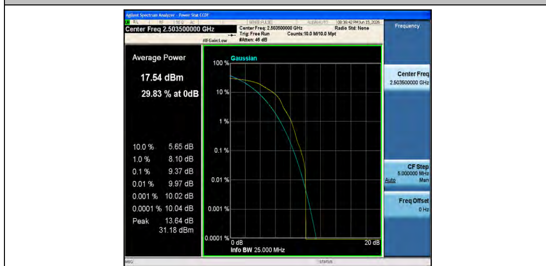
Band41-15MHz-16QAM-39725-1RB#0-PASS
