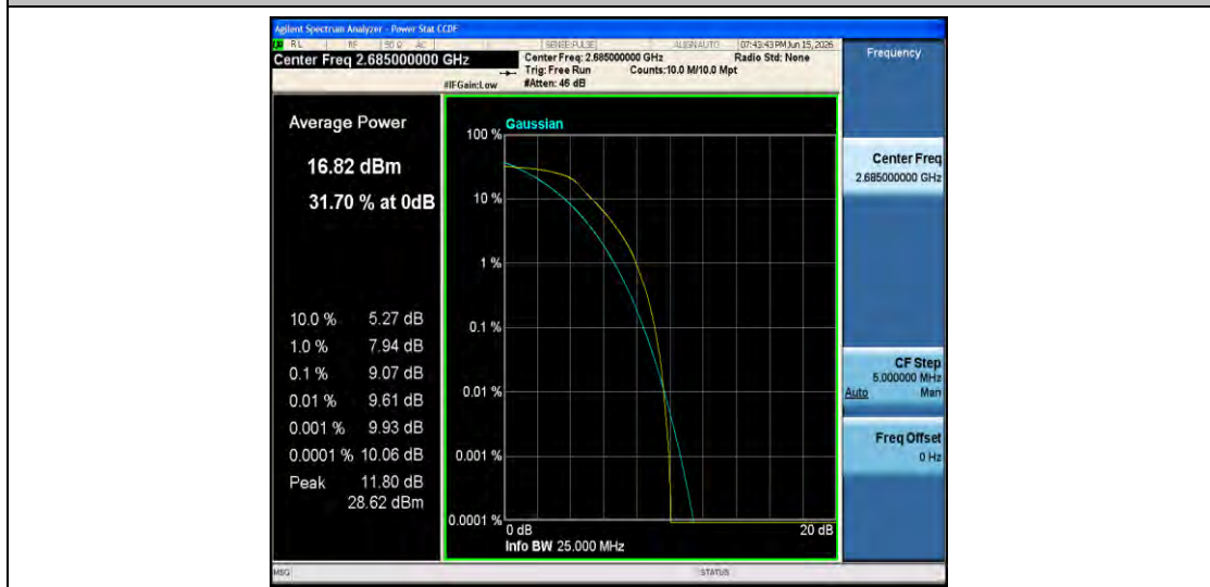
Band41-10MHz-QPSK-41540-50RB#0-PASS
