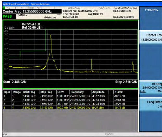
Band41-20MHz-QPSK-39750-1RB#0-PASS
