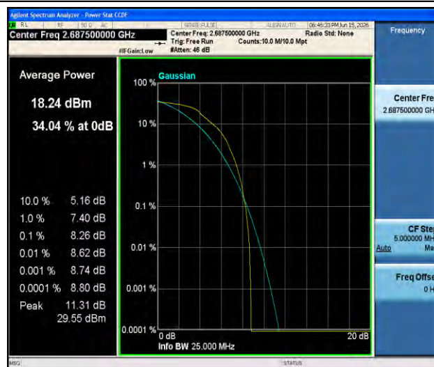
Band41-5MHz-QPSK-41565-1RB#0-PASS
