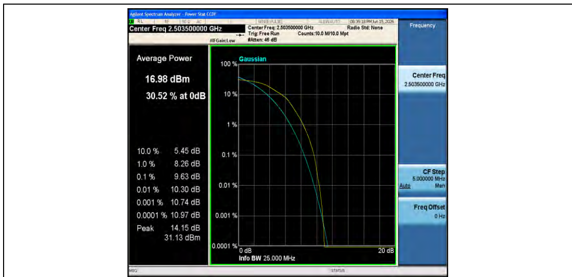
Band41-15MHz-16QAM-39725-75RB#0-PASS
