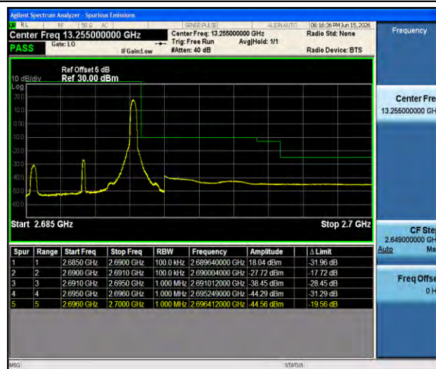
Band41-5MHz-QPSK-41565-1RB#24-PASS
