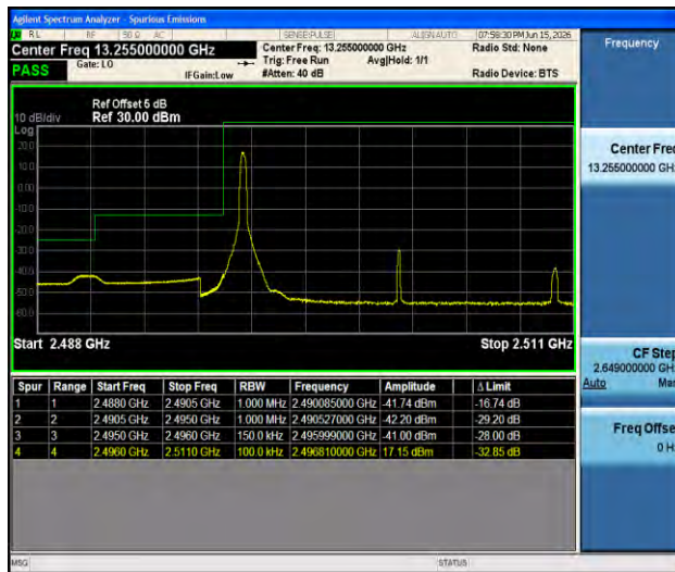
Band41-15MHz-16QAM-39725-1RB#0-PASS
