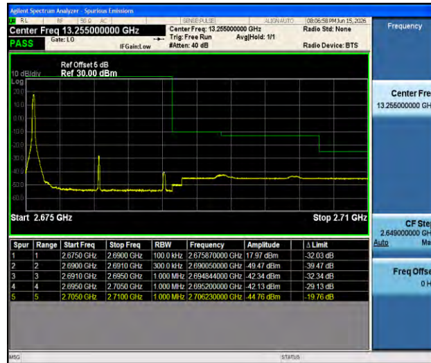
Band41-15MHz-QPSK-41515-1RB#0-PASS
