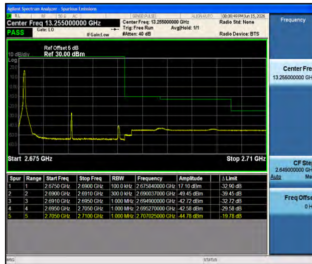
Band41-15MHz-16QAM-41515-1RB#0-PASS
