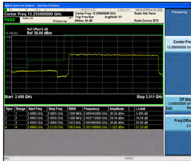
Band41-15MHz-QPSK-39725-75RB#0-PASS
