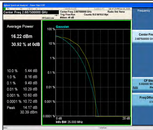
Band41-5MHz-16QAM-41565-25RB#0-PASS
