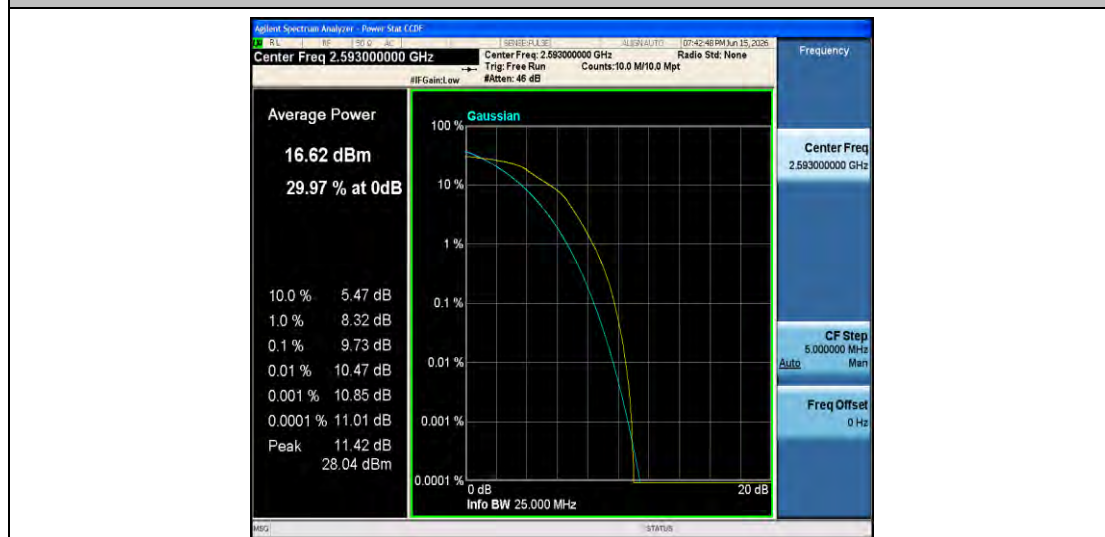
Band41-10MHz-16QAM-40620-50RB#0-PASS
