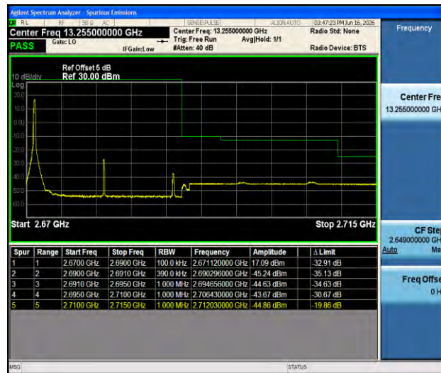
Band41-20MHz-16QAM-41490-1RB#0-PASS
