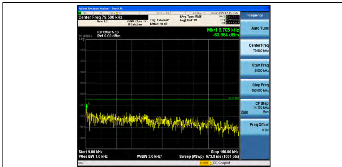
Band41-5MHz-QPSK-39675-1RB#0-0.009~0.15-PASS
