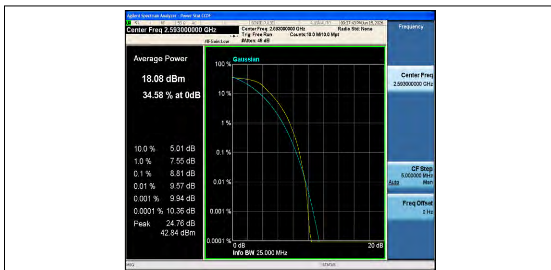
Band41-20MHz-QPSK-40620-100RB#0-PASS
