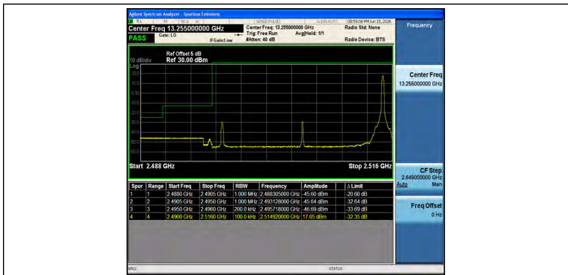
Band41-20MHz-16QAM-39750-1RB#99-PASS
