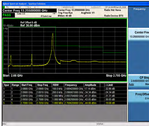
Band41-10MHz-16QAM-41540-1RB#49-PASS
