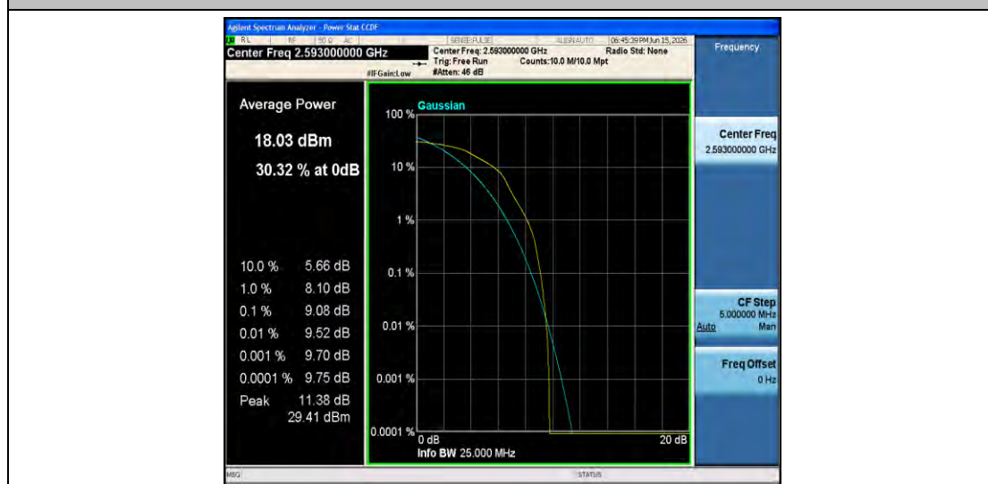
Band41-5MHz-16QAM-40620-1RB#0-PASS
