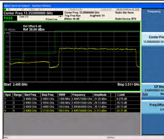
Band41-15MHz-16QAM-39725-75RB#0-PASS
