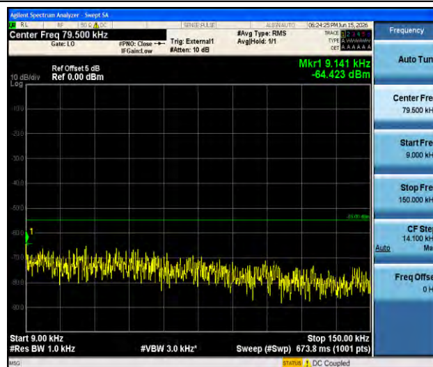
Band41-5MHz-16QAM-39675-1RB#0-0.009~0.15-PASS
