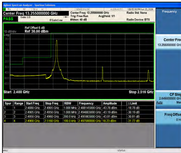
Band41-20MHz-16QAM-39750-1RB#0-PASS
