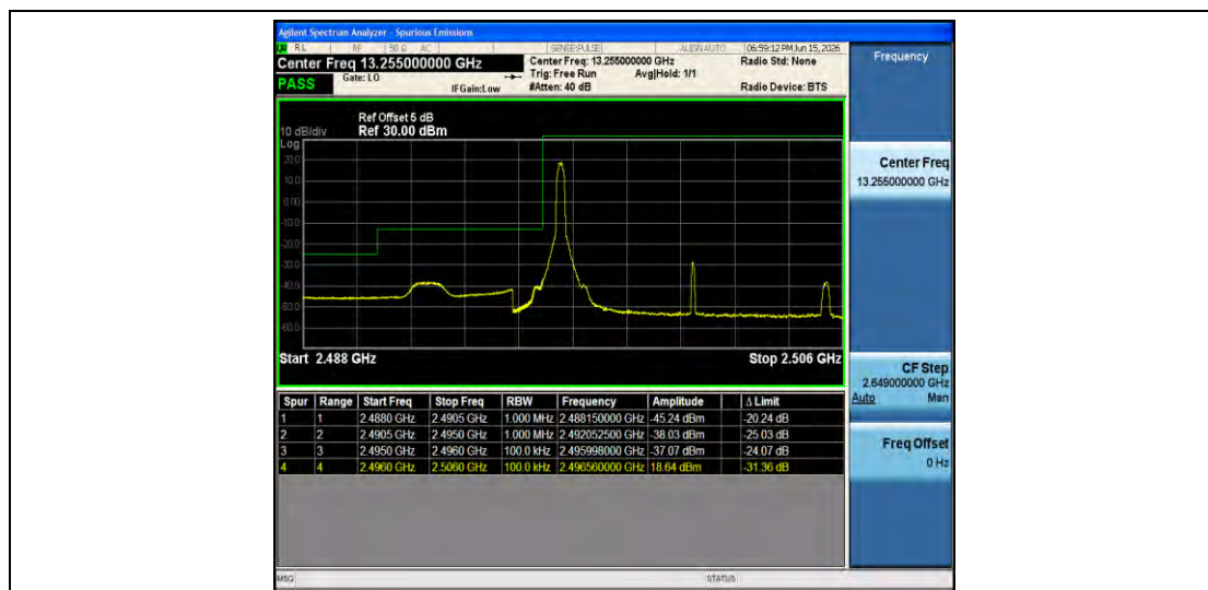
Band41-10MHz-QPSK-39700-1RB#0-PASS
