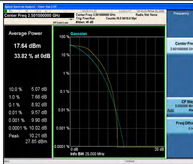
Band41-10MHz-QPSK-39700-50RB#0-PASS
