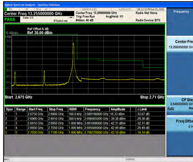
Band41-15MHz-16QAM-41515-1RB#74-PASS
