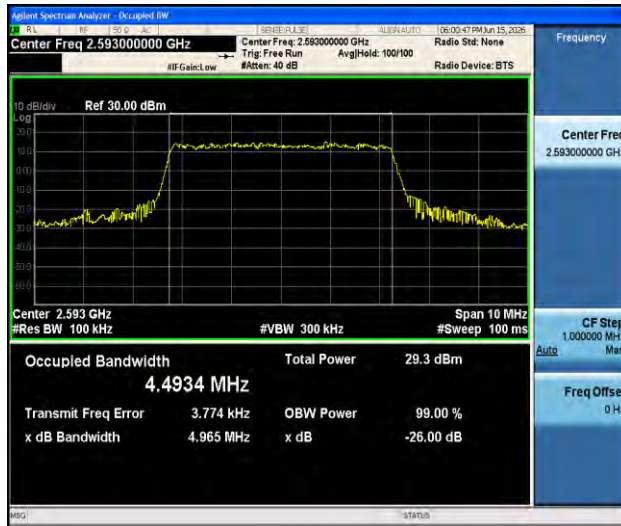
Band41-5MHz-16QAM-40620-25RB#0-PASS
