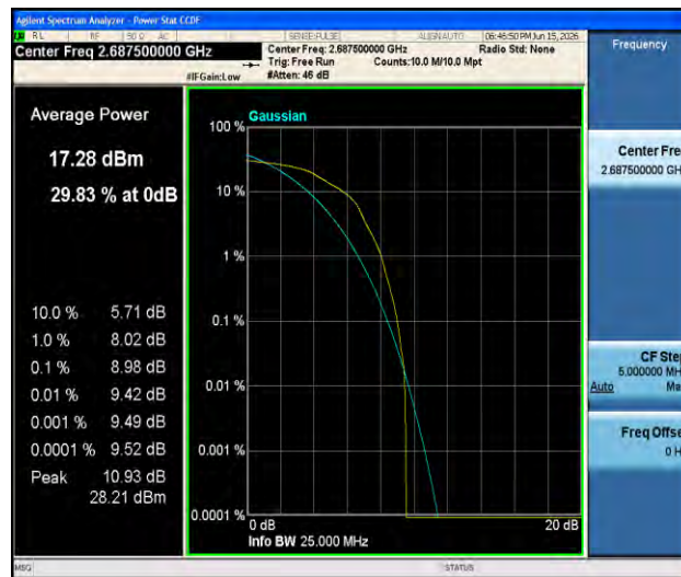
Band41-5MHz-16QAM-41565-1RB#0-PASS
