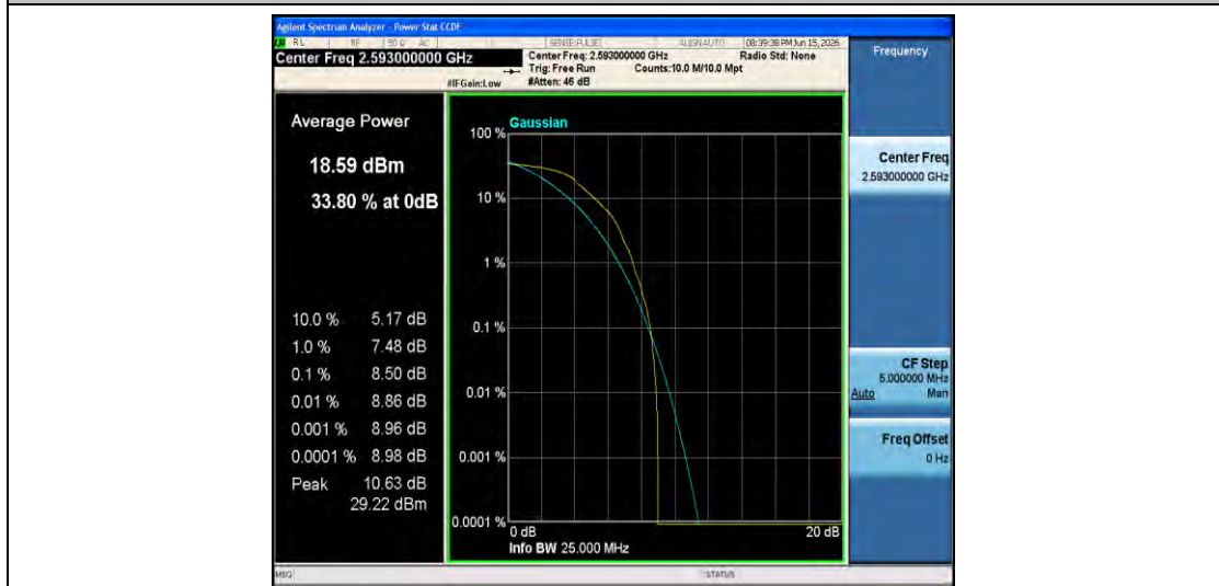
Band41-15MHz-QPSK-40620-1RB#0-PASS
