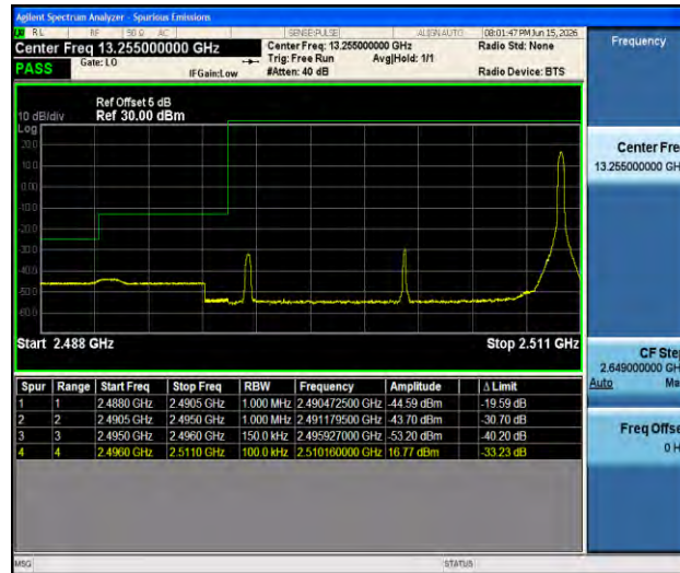
Band41-15MHz-16QAM-39725-1RB#74-PASS
