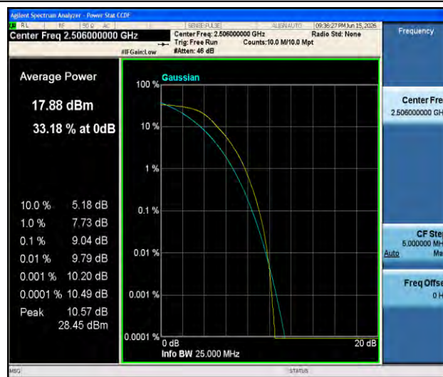
Band41-20MHz-QPSK-39750-100RB#0-PASS
