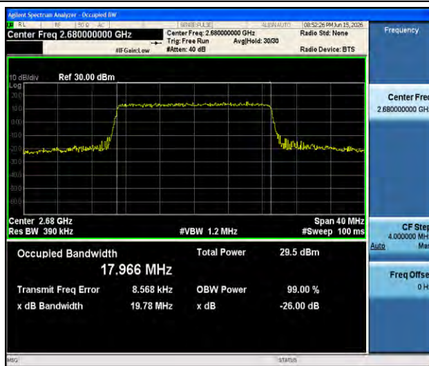
Band41-20MHz-16QAM-41490-100RB#0-PASS
