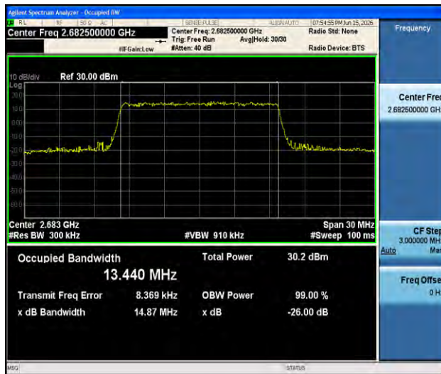
Band41-15MHz-QPSK-41515-75RB#0-PASS
