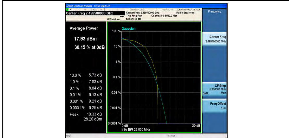
Band41-5MHz-16QAM-39675-1RB#0-PASS
