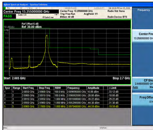
Band41-5MHz-16QAM-41565-1RB#24-PASS
