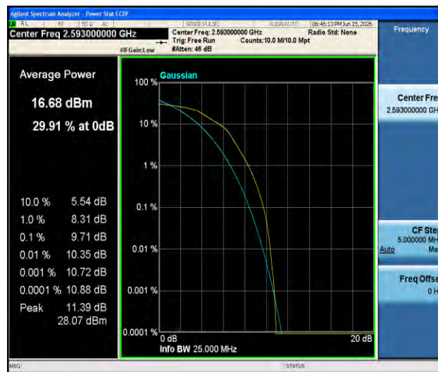
Band41-5MHz-16QAM-40620-25RB#0-PASS
