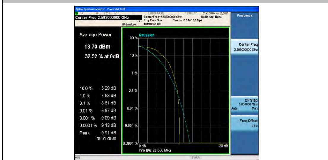
Band41-10MHz-QPSK-40620-1RB#0-PASS
