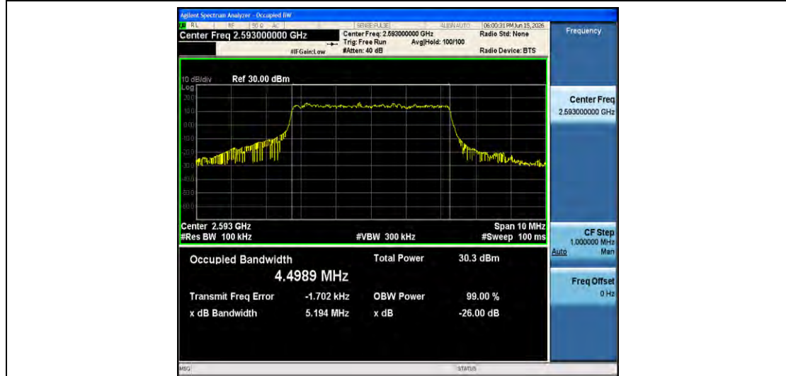
Band41-5MHz-QPSK-40620-25RB#0-PASS
