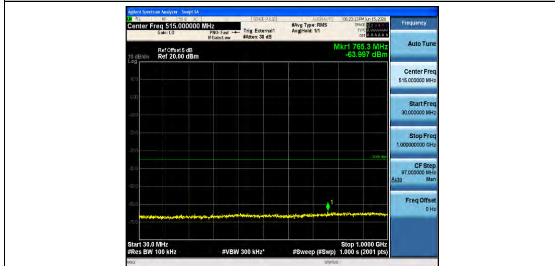
Band41-5MHz-QPSK-39675-1RB#0-30~1000-PASS
