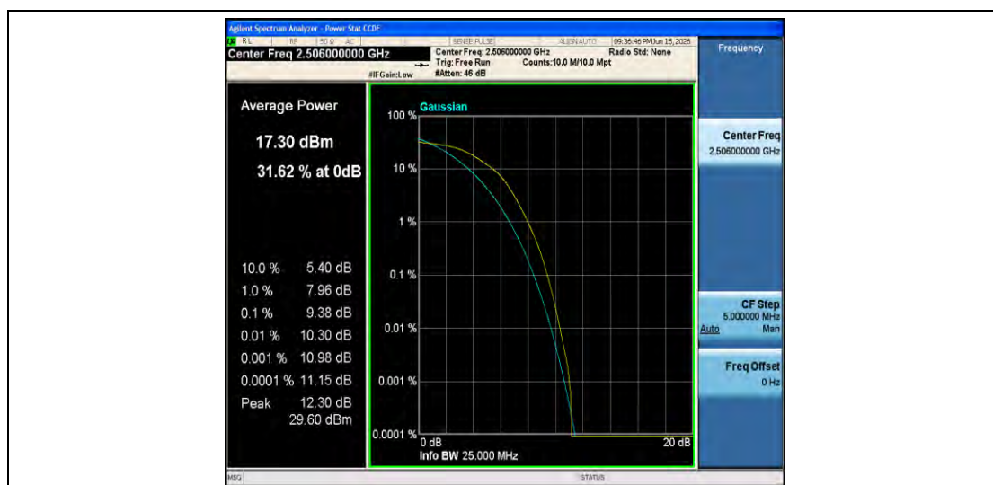
Band41-20MHz-16QAM-39750-100RB#0-PASS
