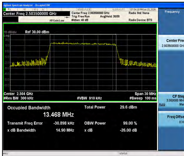
Band41-15MHz-16QAM-39725-75RB#0-PASS
