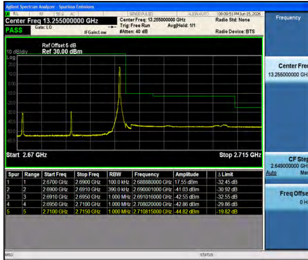
Band41-20MHz-16QAM-41490-1RB#99-PASS
