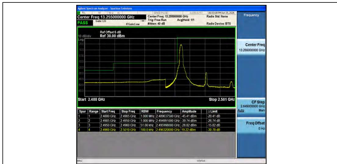
Band41-5MHz-QPSK-39675-1RB#0-PASS
