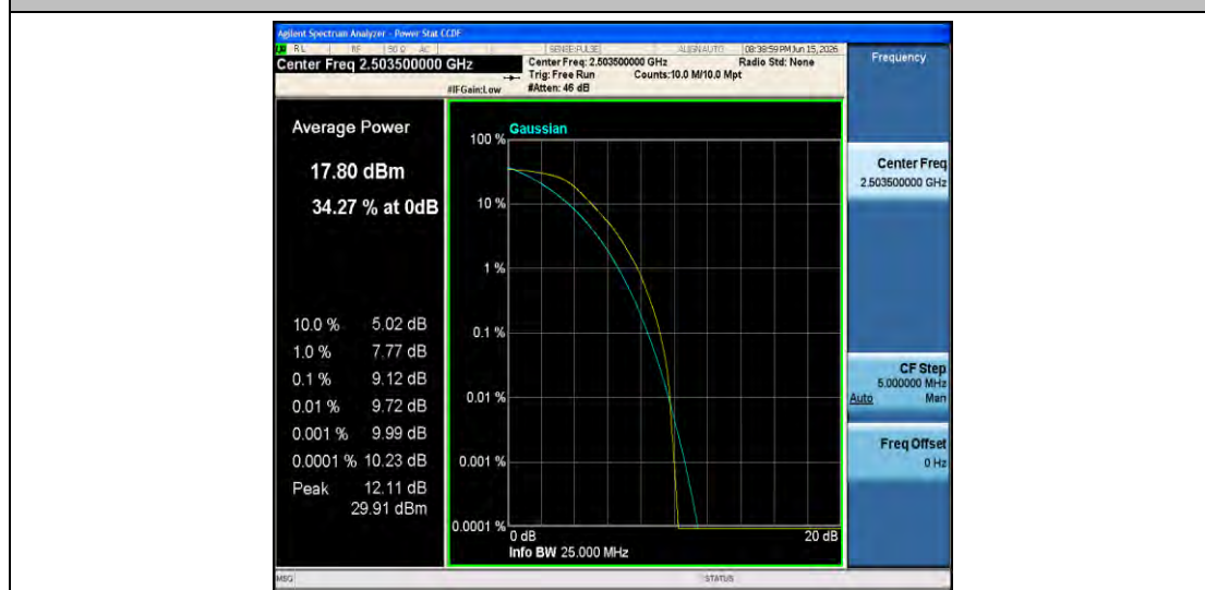
Band41-15MHz-QPSK-39725-75RB#0-PASS
