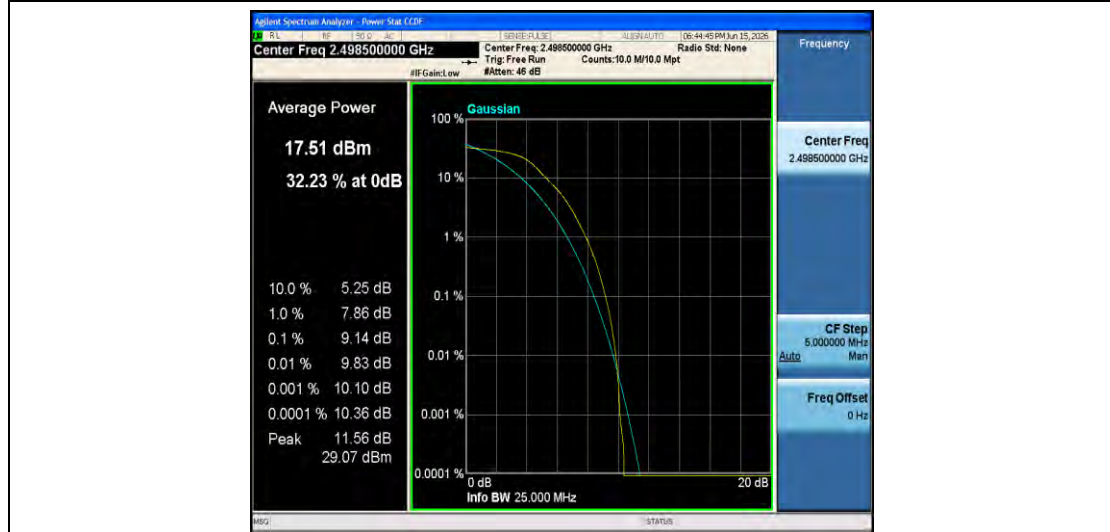
Band41-5MHz-QPSK-39675-25RB#0-PASS
