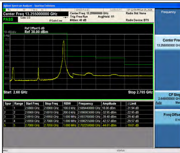
Band41-10MHz-QPSK-41540-1RB#49-PASS
