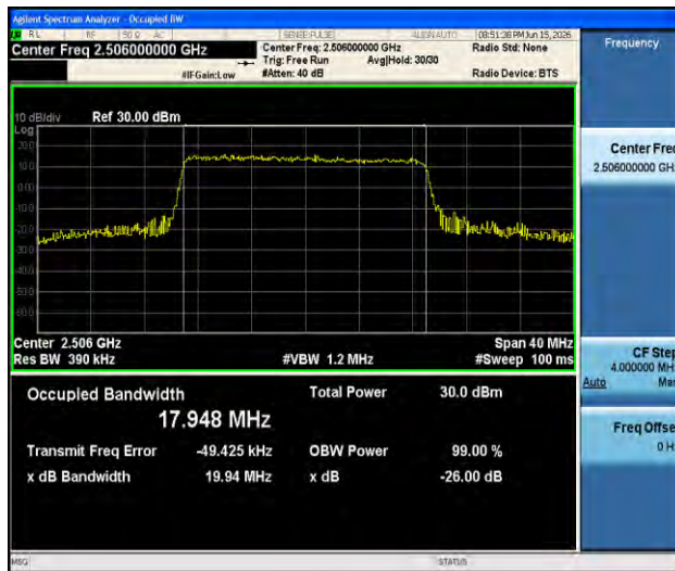
Band41-20MHz-16QAM-39750-100RB#0-PASS
