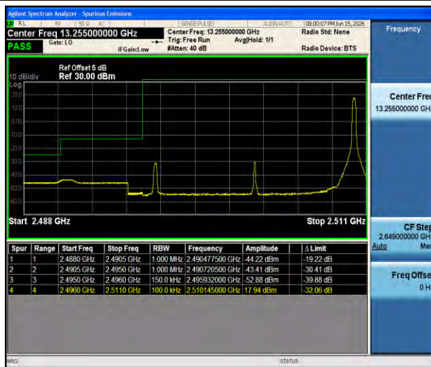
Band41-15MHz-QPSK-39725-1RB#74-PASS
