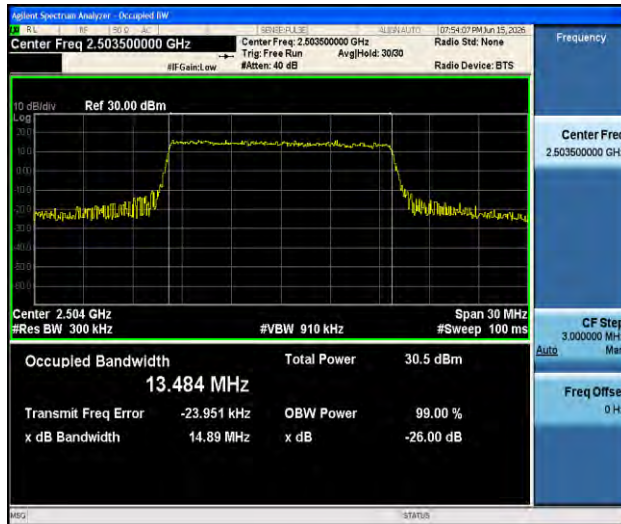
Band41-15MHz-QPSK-39725-75RB#0-PASS
