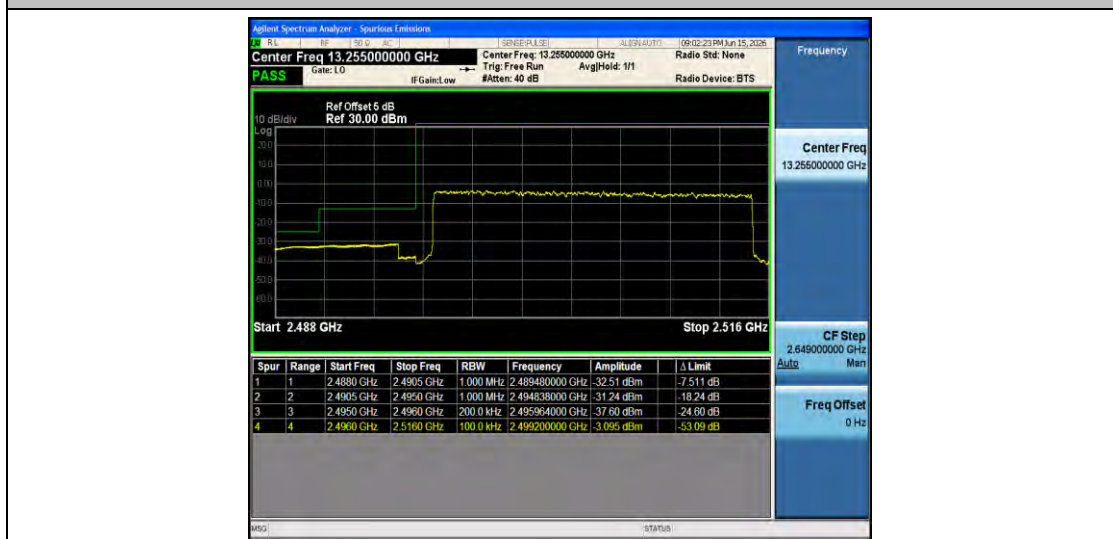
Band41-20MHz-16QAM-39750-100RB#0-PASS
