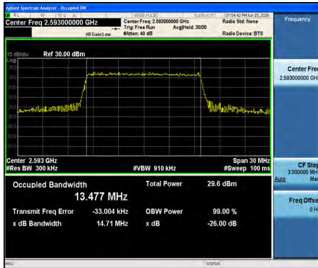
Band41-15MHz-16QAM-40620-75RB#0-PASS
