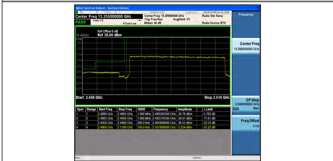
Band41-20MHz-QPSK-39750-100RB#0-PASS
