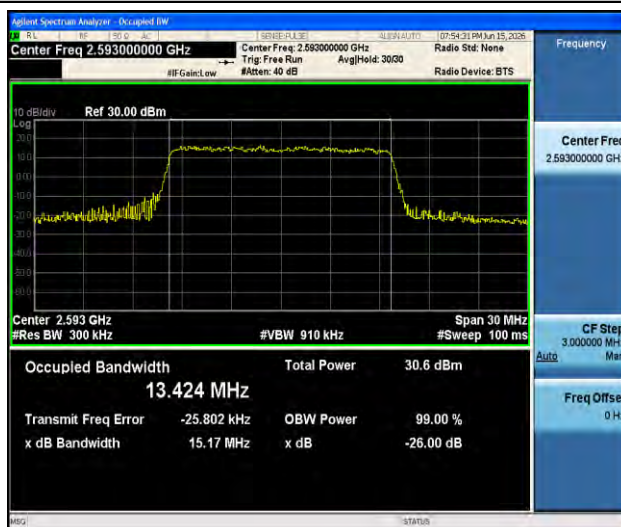
Band41-15MHz-QPSK-40620-75RB#0-PASS
