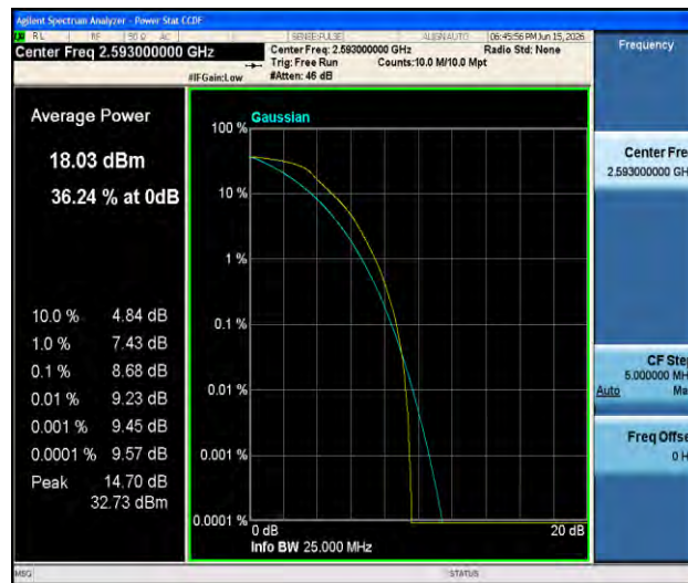
Band41-5MHz-QPSK-40620-25RB#0-PASS
