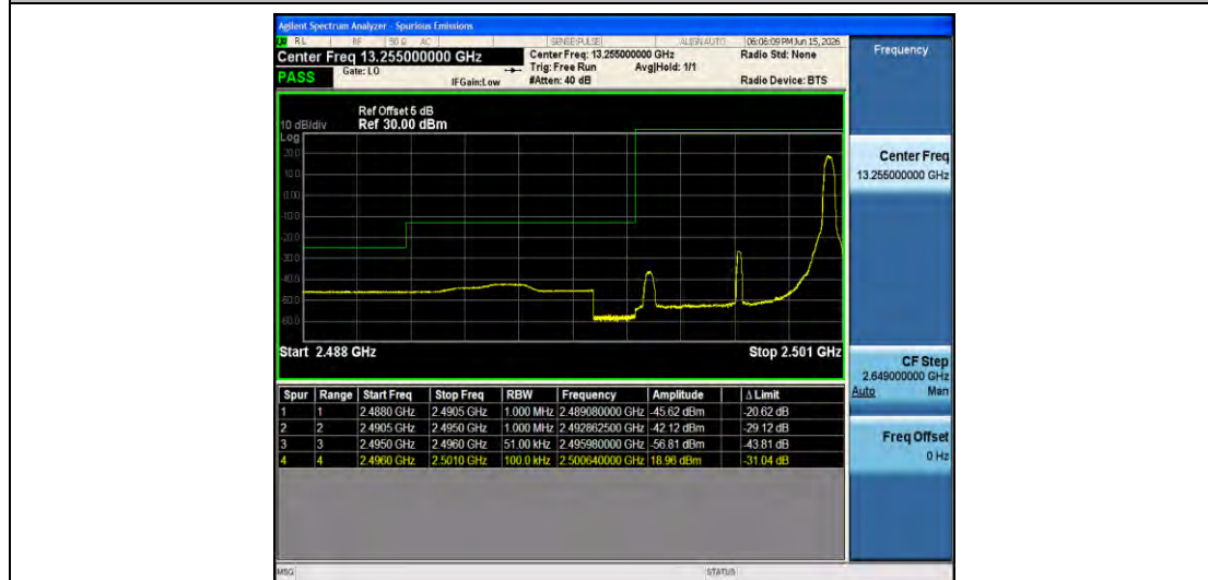
Band41-5MHz-QPSK-39675-1RB#24-PASS
