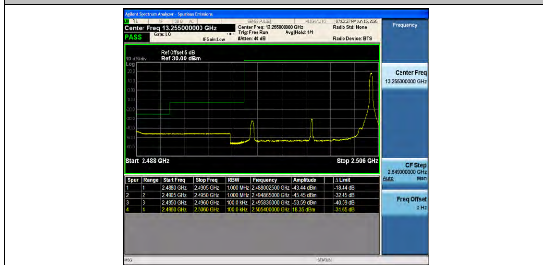
Band41-10MHz-QPSK-39700-1RB#49-PASS
