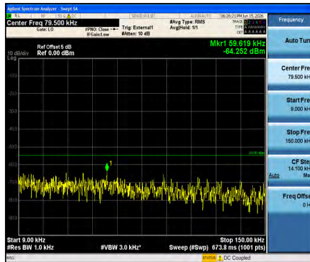
Band41-5MHz-QPSK-40620-1RB#0-0.009~0.15-PASS
