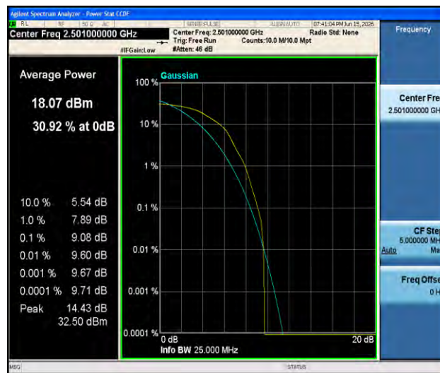
Band41-10MHz-16QAM-39700-1RB#0-PASS
