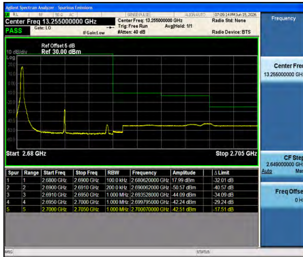
Band41-10MHz-QPSK-41540-1RB#0-PASS
