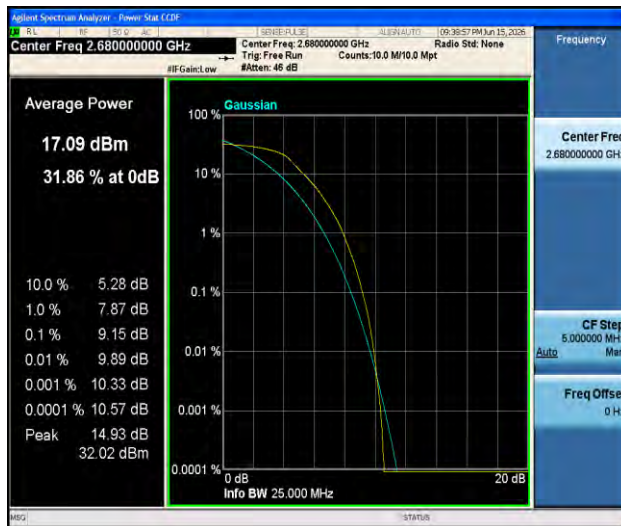
Band41-20MHz-QPSK-41490-100RB#0-PASS
