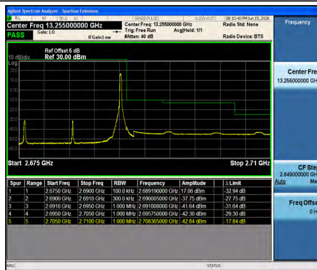
Band41-15MHz-QPSK-41515-1RB#74-PASS
