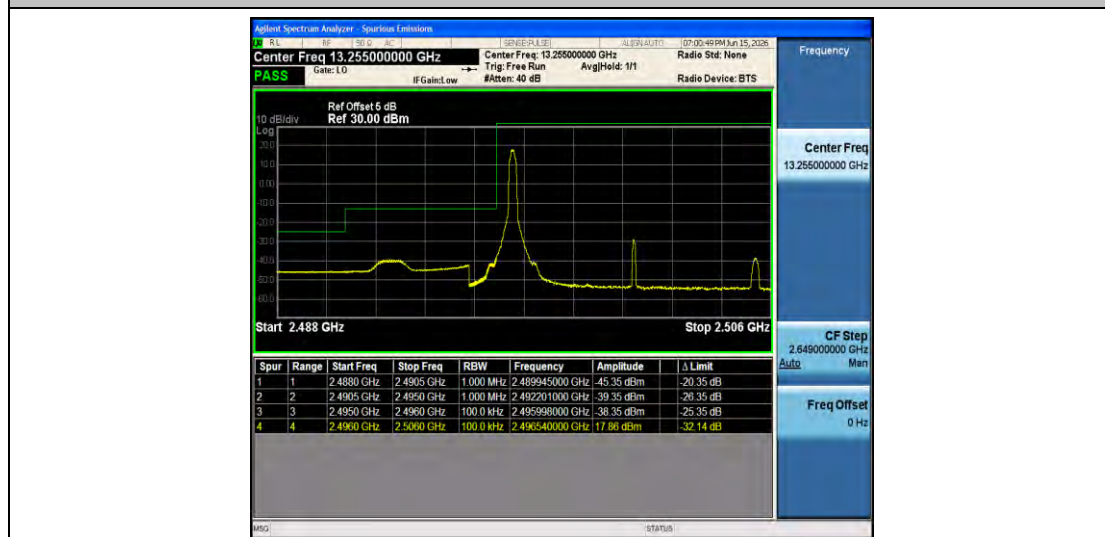
Band41-10MHz-16QAM-39700-1RB#0-PASS
