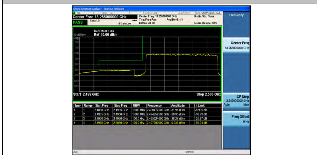
Band41-10MHz-16QAM-39700-50RB#0-PASS
