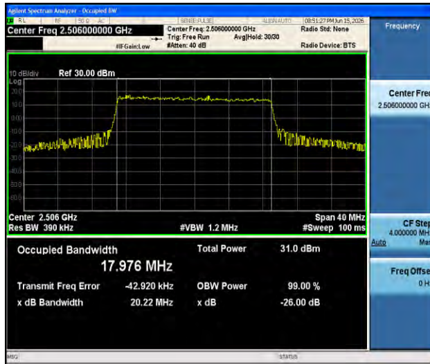
Band41-20MHz-QPSK-39750-100RB#0-PASS
