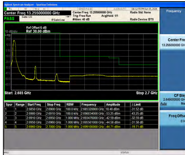
Band41-5MHz-QPSK-41565-1RB#0-PASS
