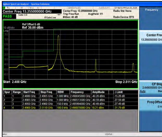
Band41-15MHz-QPSK-39725-1RB#0-PASS
