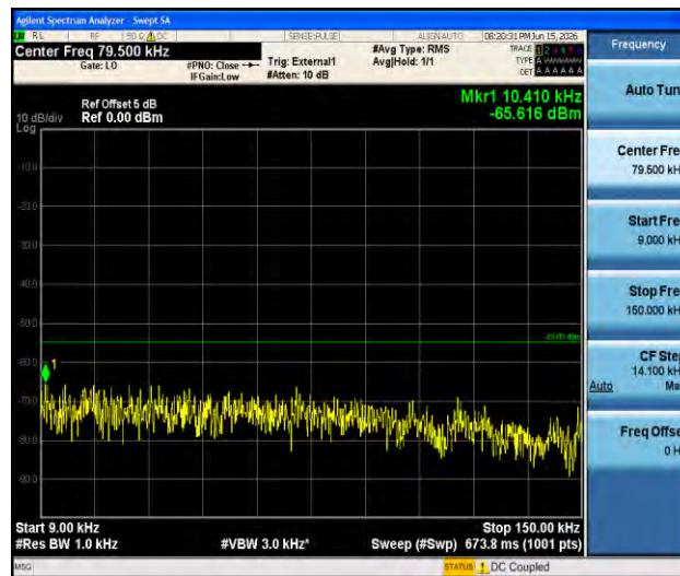
Band41-15MHz-QPSK-40620-1RB#0-0.009~0.15-PASS
