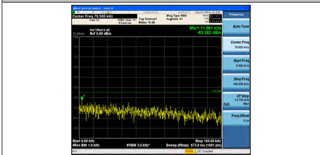
Band41-15MHz-QPSK-41515-1RB#0-0.009~0.15-PASS
