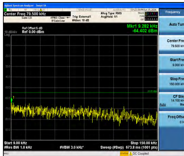
Band41-10MHz-QPSK-40620-1RB#0-0.009~0.15-PASS
