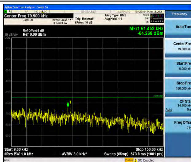
Band41-10MHz-16QAM-41540-1RB#0-0.009~0.15-PASS
