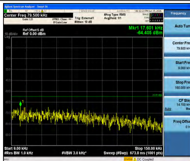
Band41-5MHz-16QAM-41565-1RB#0-0.009~0.15-PASS
