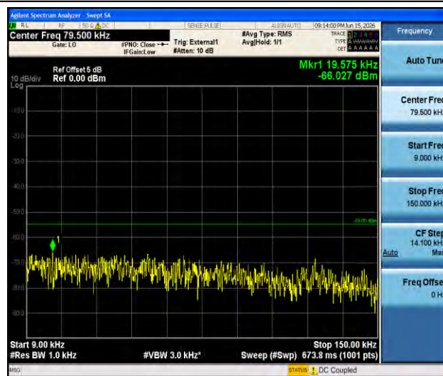
Band41-20MHz-QPSK-39750-1RB#0-0.009~0.15-PASS
