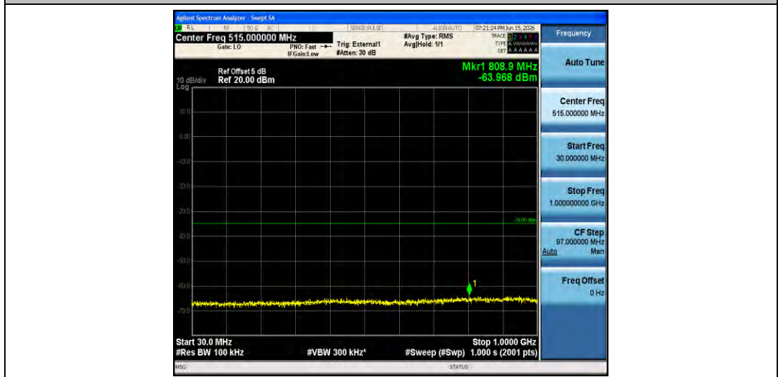
Band41-10MHz-16QAM-39700-1RB#0-30~1000-PASS
