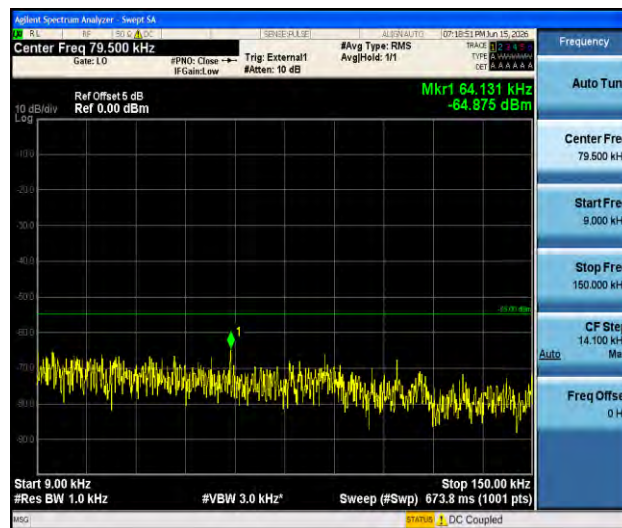
Band41-10MHz-QPSK-39700-1RB#0-0.009~0.15-PASS
