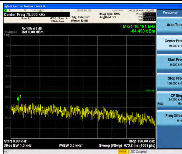
Band41-15MHz-16QAM-40620-1RB#0-0.009~0.15-PASS
