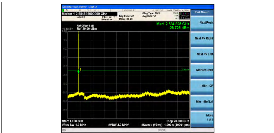
Band41-10MHz-16QAM-41540-1RB#0-1000~20000-PASS
