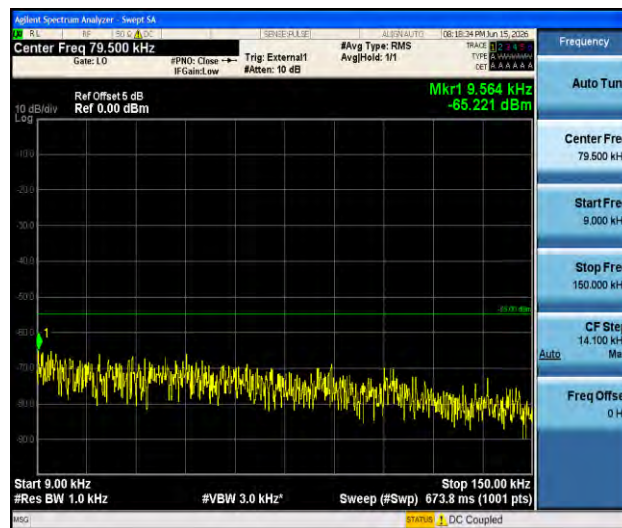
Band41-15MHz-16QAM-39725-1RB#0-0.009~0.15-PASS
