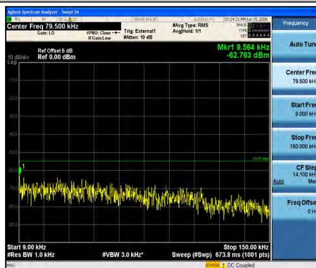
Band41-10MHz-16QAM-40620-1RB#0-0.009~0.15-PASS
