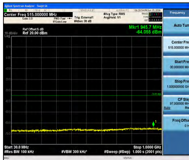
Band41-5MHz-16QAM-40620-1RB#0-30~1000-PASS
