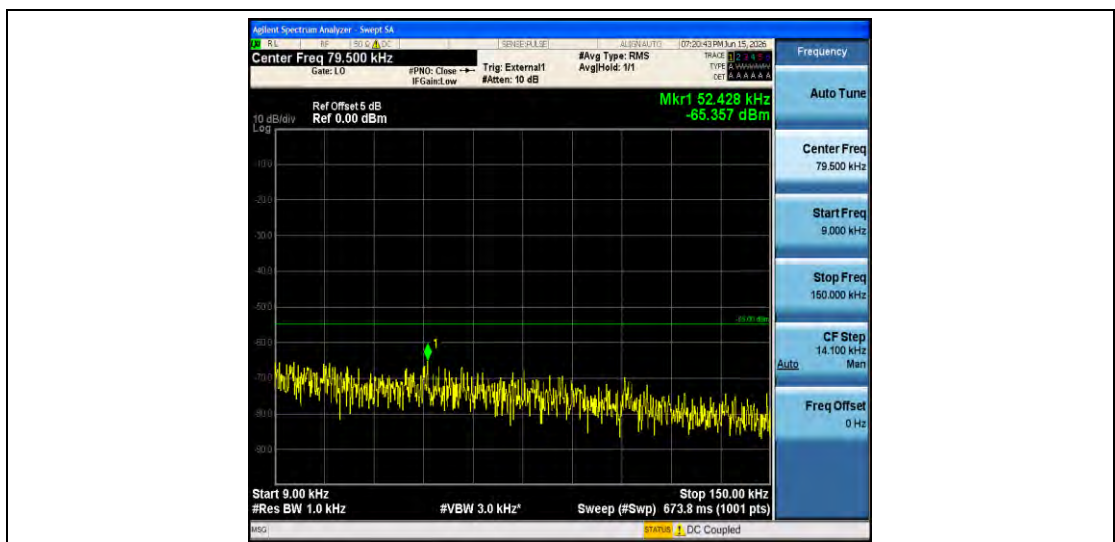
Band41-10MHz-16QAM-39700-1RB#0-0.009~0.15-PASS
