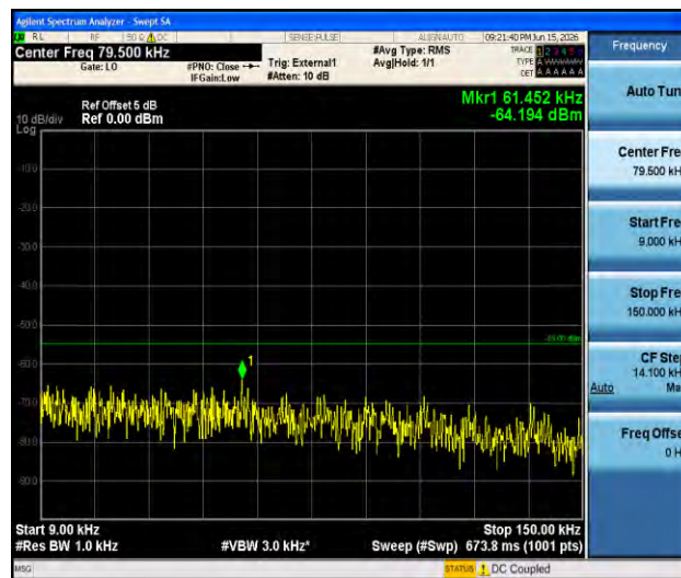
Band41-20MHz-QPSK-41490-1RB#0-0.009~0.15-PASS
