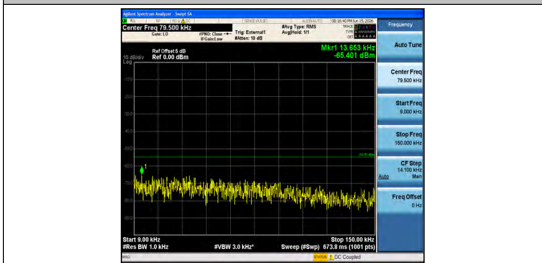
Band41-15MHz-QPSK-39725-1RB#0-0.009~0.15-PASS
