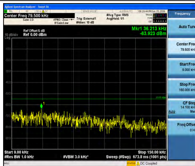
Band41-20MHz-16QAM-40620-1RB#0-0.009~0.15-PASS
