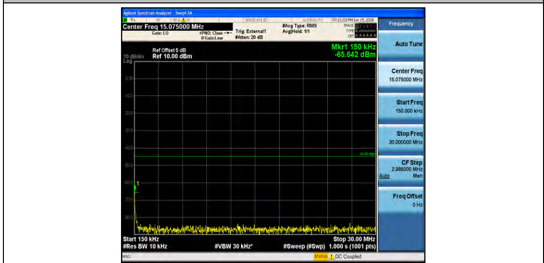
Band41-10MHz-16QAM-39700-1RB#0-0.15~30-PASS
