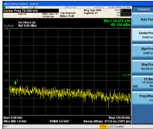
Band41-10MHz-QPSK-41540-1RB#0-0.009~0.15-PASS
