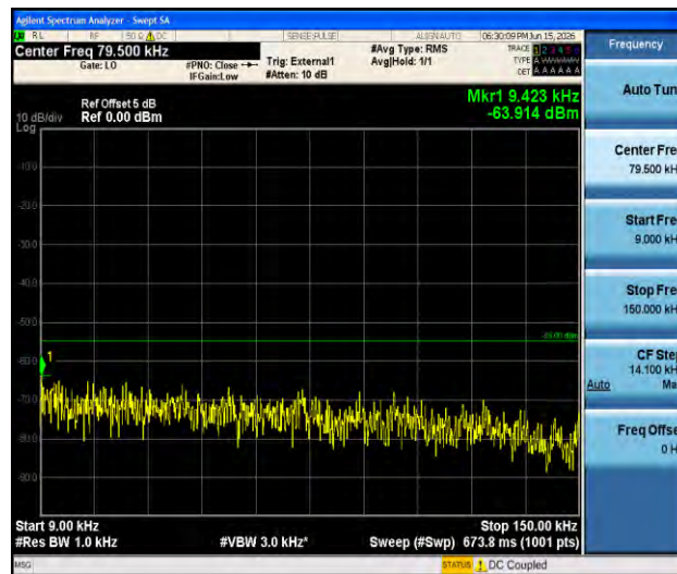
Band41-5MHz-QPSK-41565-1RB#0-0.009~0.15-PASS
