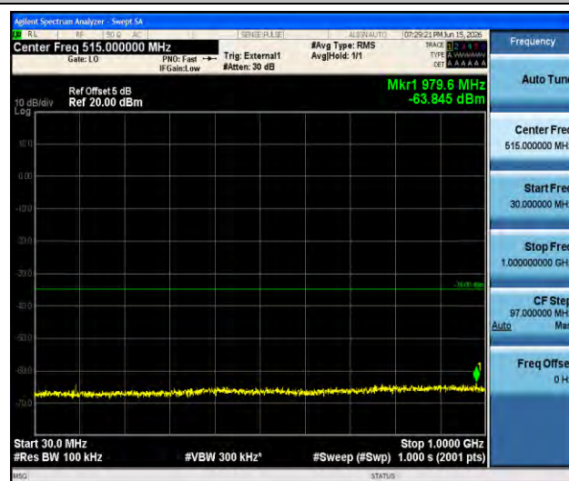
Band41-10MHz-16QAM-41540-1RB#0-30~1000-PASS
