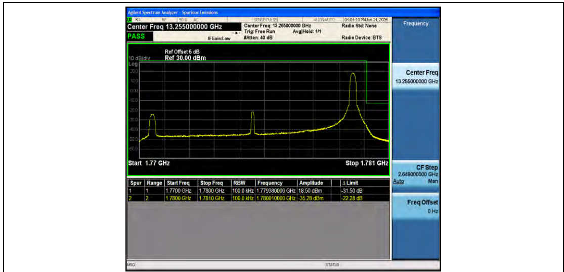
Band66-10MHz-16QAM-132622-1RB#49-PASS
