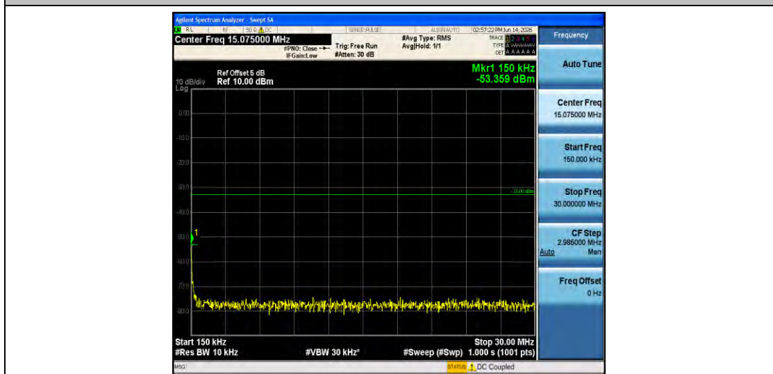
Band66-3MHz-QPSK-132322-1RB#0-0.15~30-PASS
