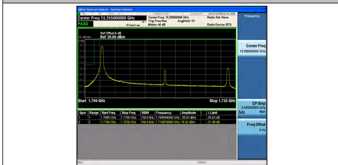
Band66-15MHz-16QAM-132047-1RB#0-PASS
