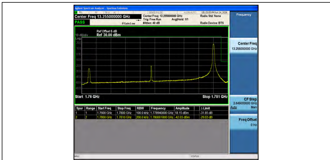
Band66-20MHz-16QAM-132572-1RB#99-PASS
