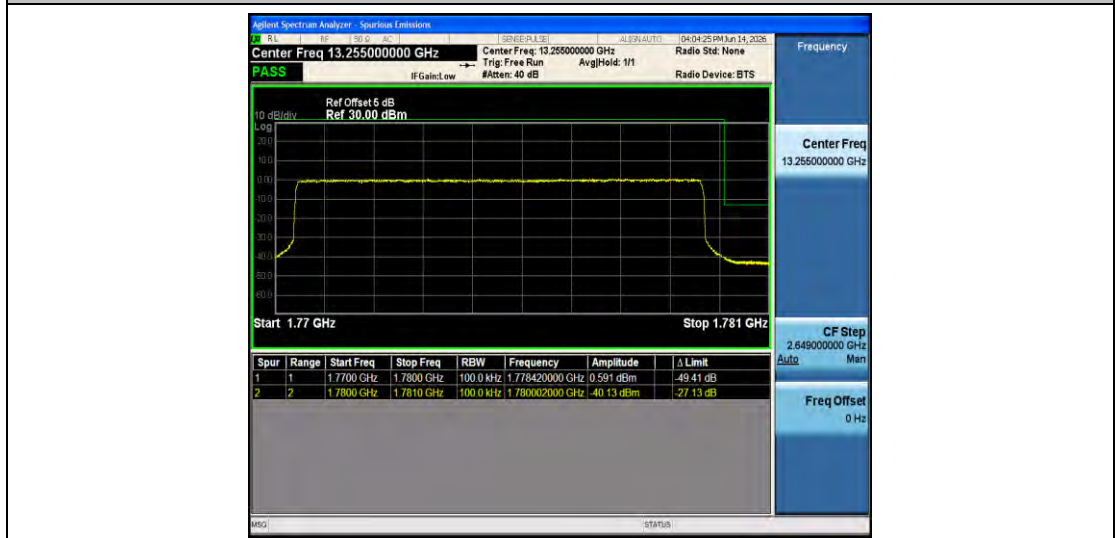
Band66-10MHz-QPSK-132622-50RB#0-PASS
