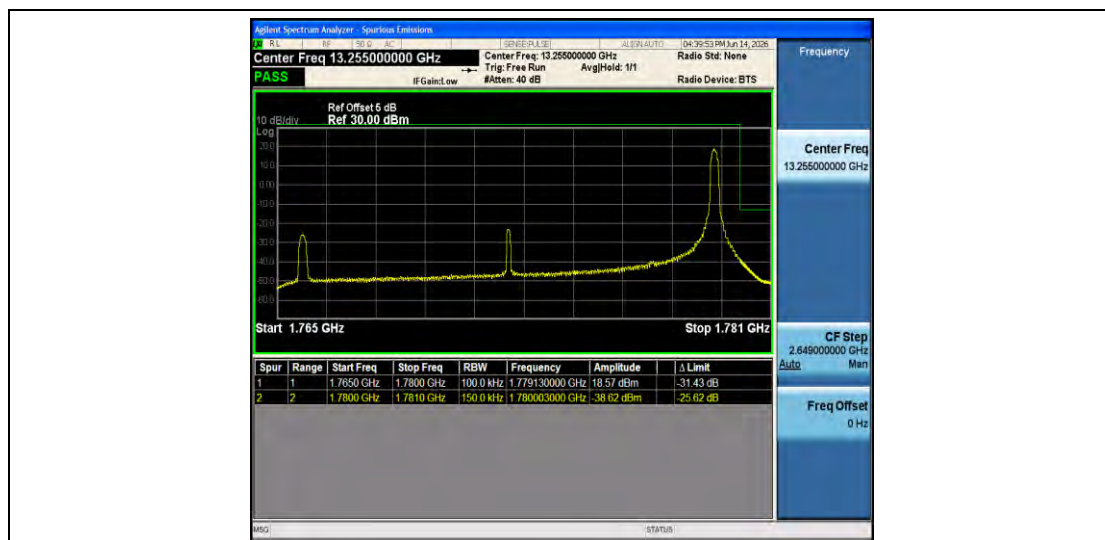
Band66-15MHz-16QAM-132597-1RB#74-PASS
