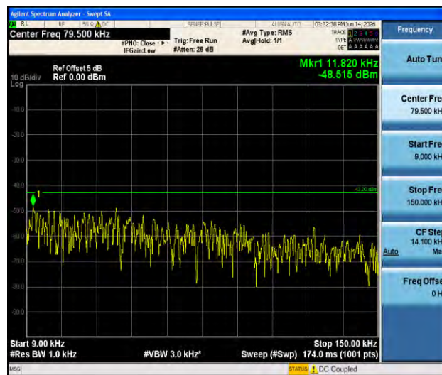
Band66-5MHz-QPSK-132322-1RB#0-0.009~0.15-PASS
