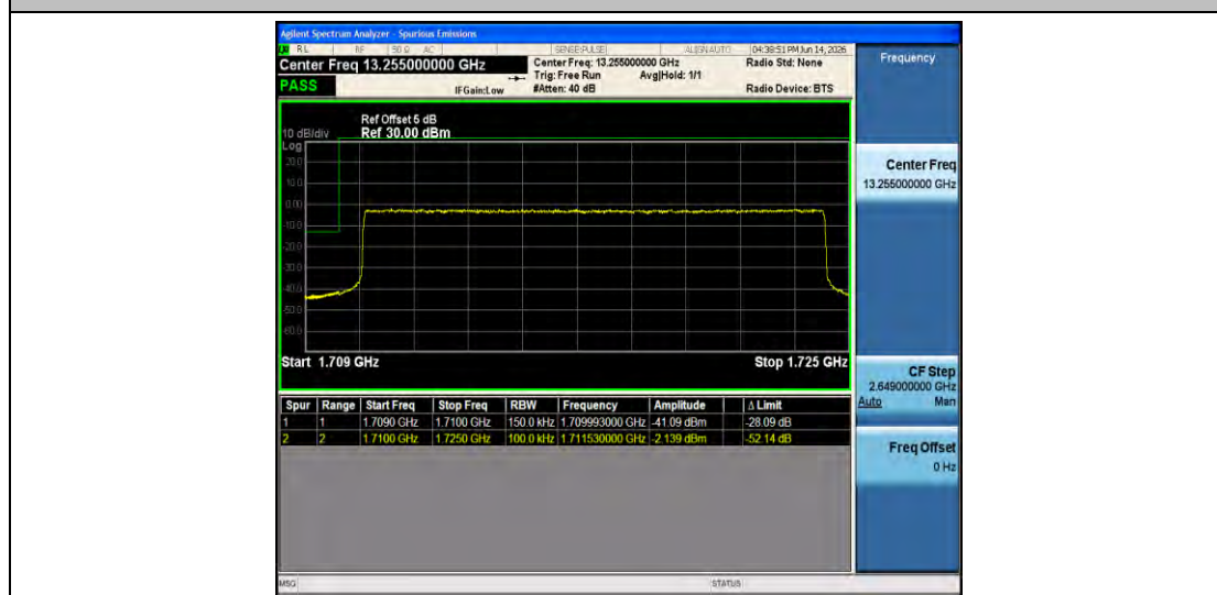
Band66-15MHz-16QAM-132047-75RB#0-PASS
