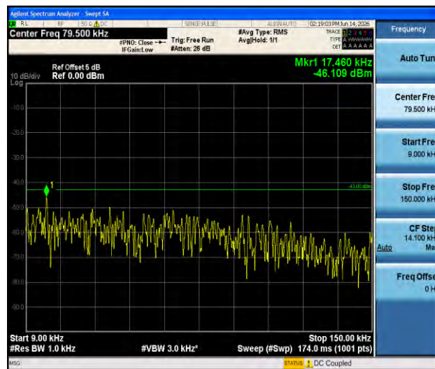
Band66-1.4MHz-16QAM-132322-1RB#0-0.009~0.15-PASS
