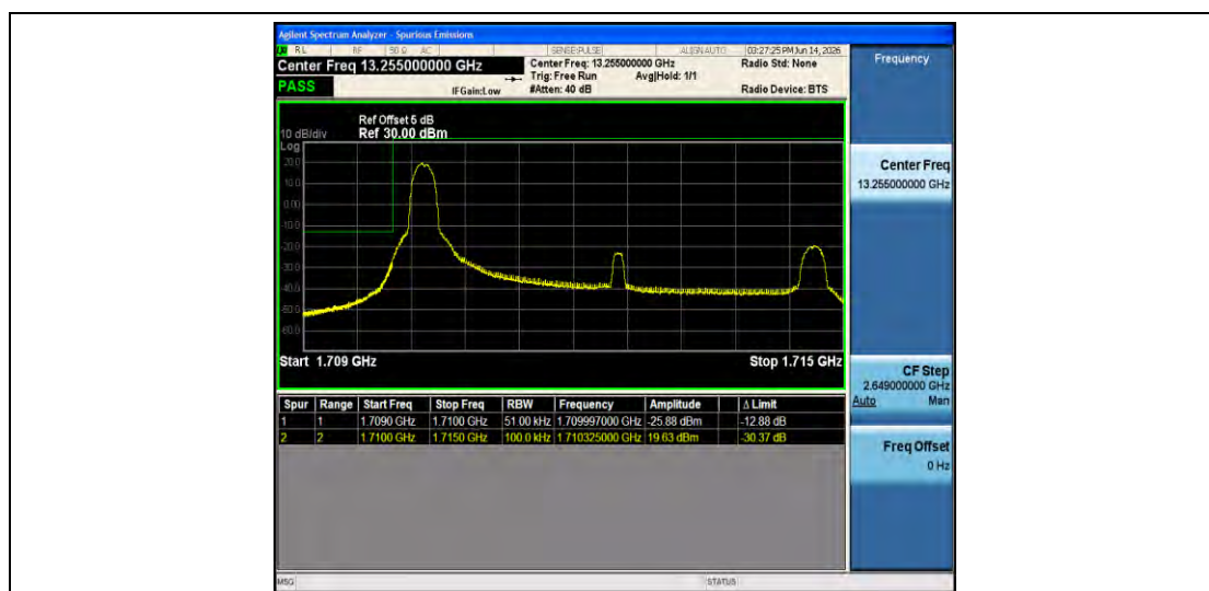
Band66-5MHz-QPSK-131997-1RB#0-PASS
