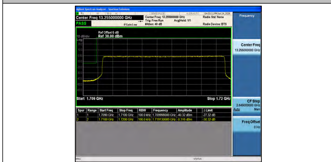
Band66-10MHz-16QAM-132022-50RB#0-PASS
