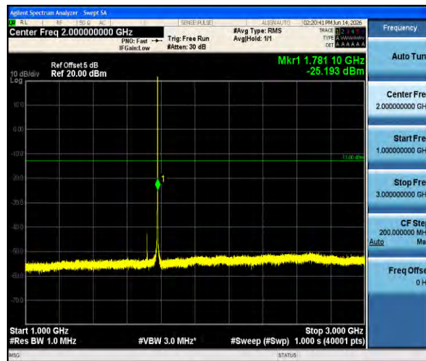
Band66-1.4MHz-QPSK-132665-1RB#0-1000~3000-PASS
