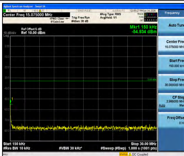
Band66-3MHz-QPSK-132657-1RB#0-0.15~30-PASS
