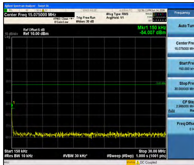
Band66-3MHz-16QAM-131987-1RB#0-0.15~30-PASS
