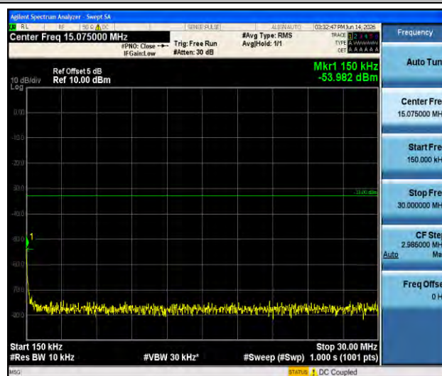
Band66-5MHz-QPSK-132322-1RB#0-0.15~30-PASS
