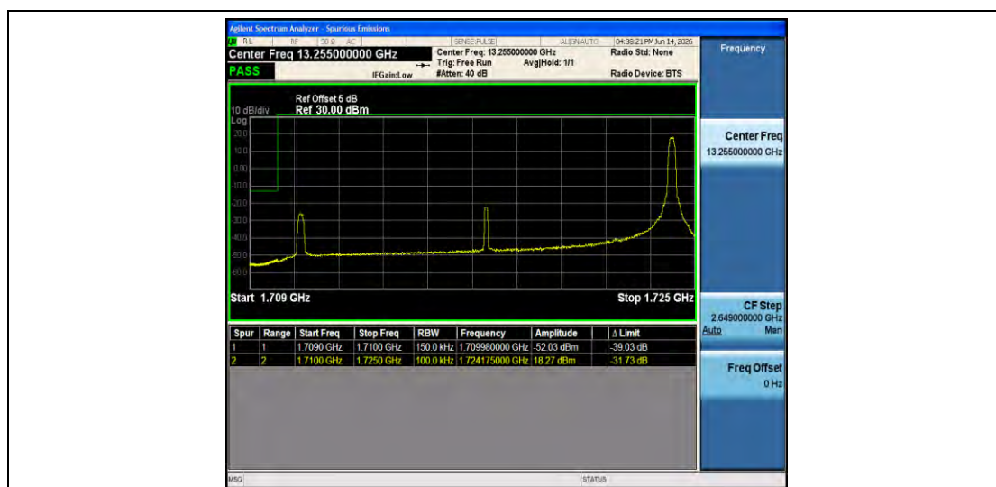
Band66-15MHz-16QAM-132047-1RB#74-PASS
