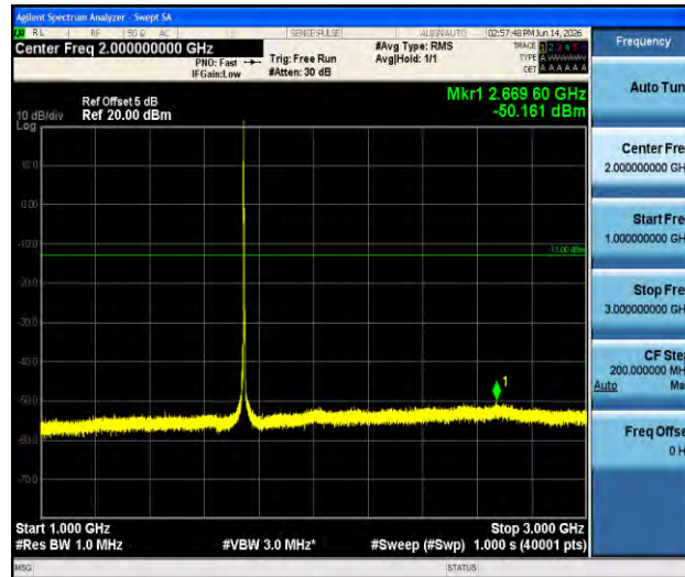
Band66-3MHz-QPSK-132322-1RB#0-1000~3000-PASS
