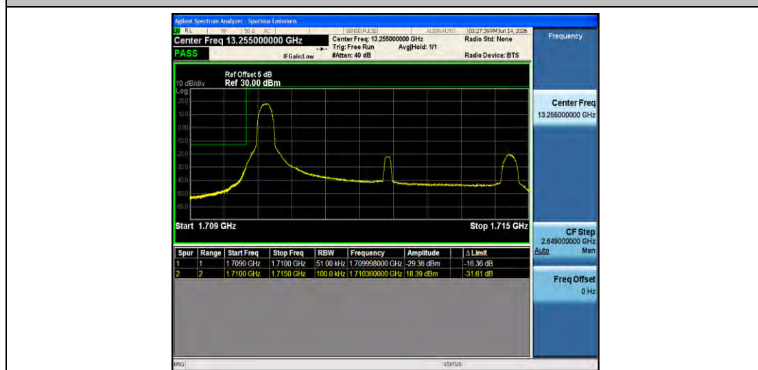
Band66-5MHz-16QAM-131997-1RB#0-PASS
