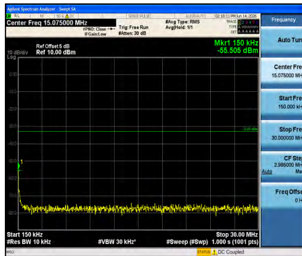
Band66-1.4MHz-QPSK-132322-1RB#0-0.15~30-PASS
