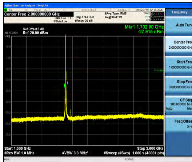
Band66-10MHz-QPSK-132022-1RB#0-1000~3000-PASS
