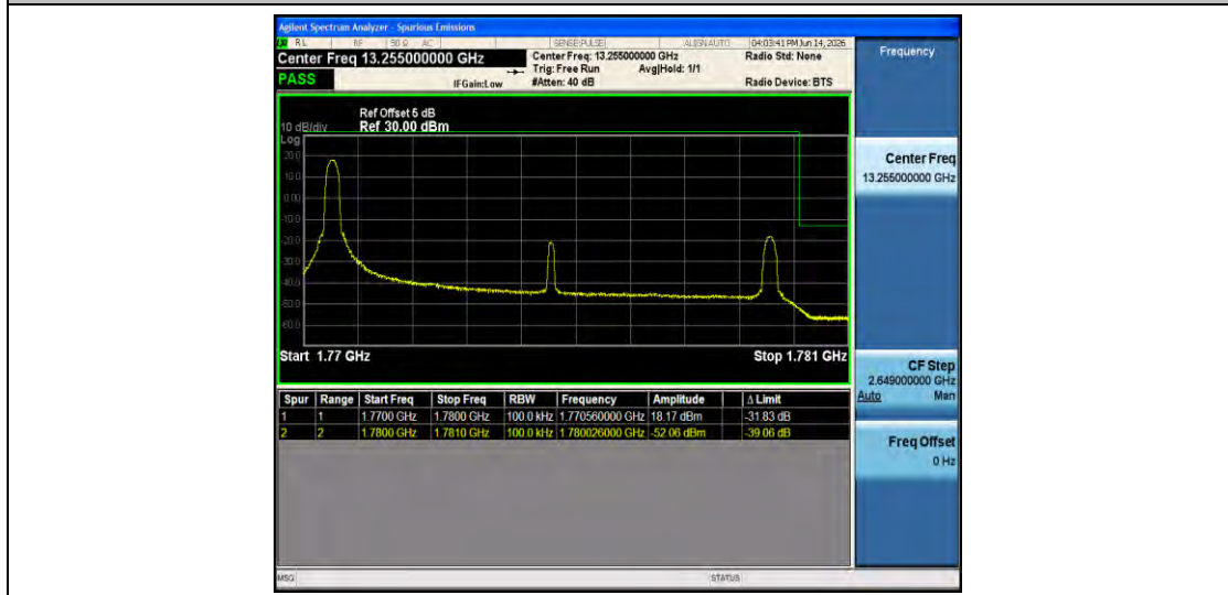
Band66-10MHz-16QAM-132622-1RB#0-PASS
