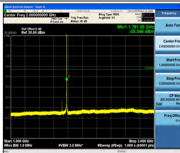
Band66-1.4MHz-16QAM-132665-1RB#0-1000~3000-PASS
