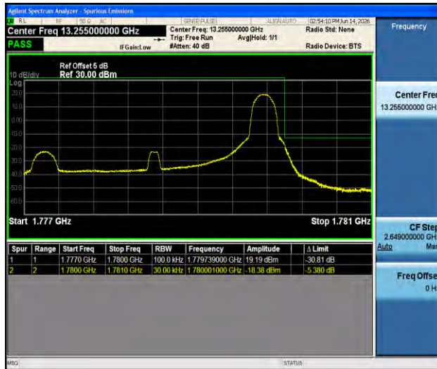
Band66-3MHz-16QAM-132657-1RB#14-PASS
