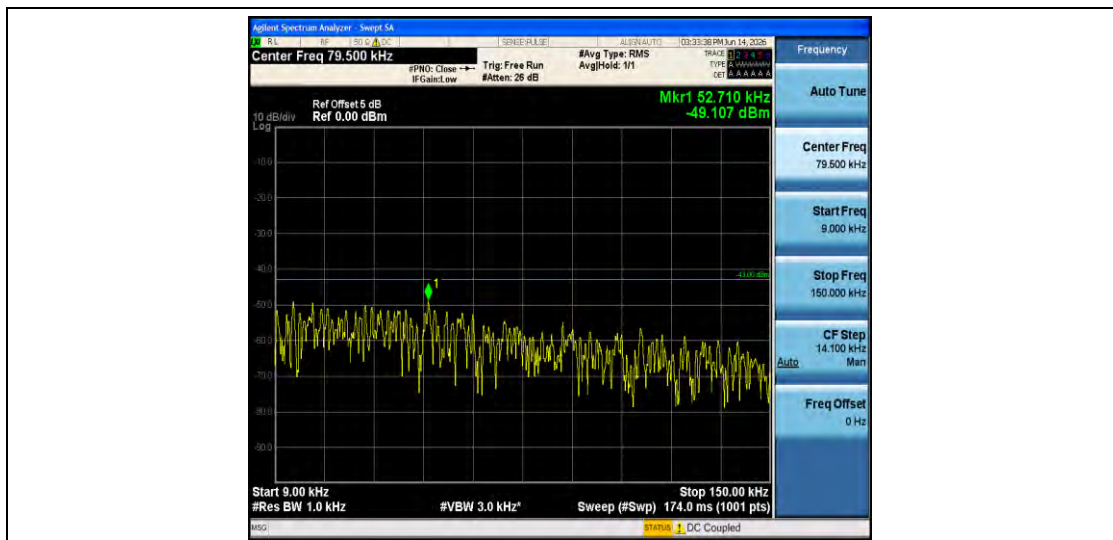
Band66-5MHz-16QAM-132322-1RB#0-0.009~0.15-PASS
