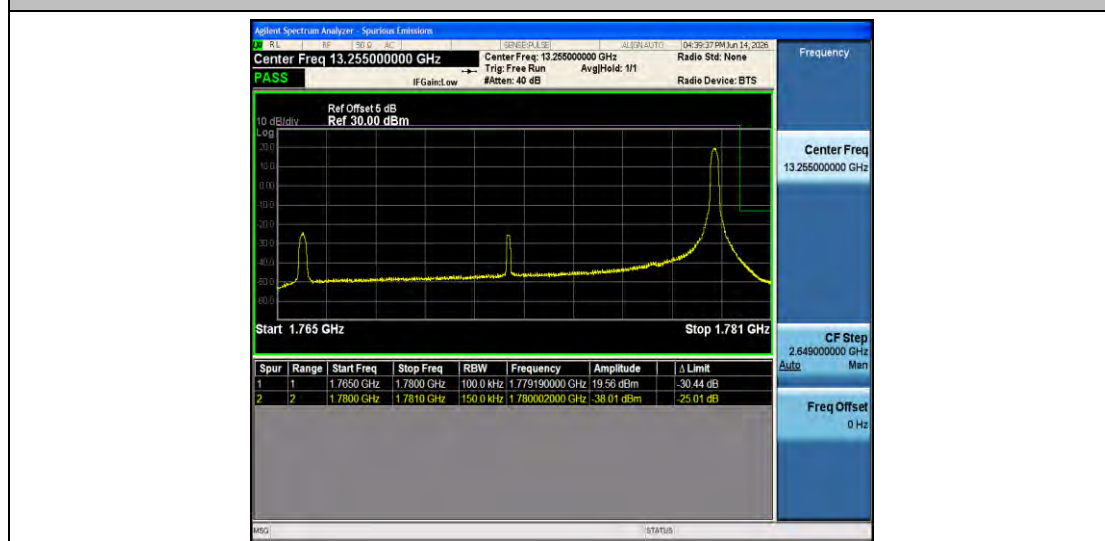
Band66-15MHz-QPSK-132597-1RB#74-PASS
