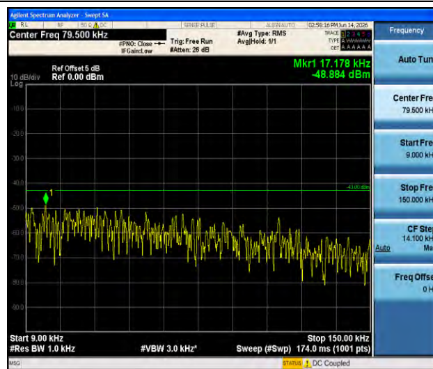
Band66-3MHz-16QAM-132322-1RB#0-0.009~0.15-PASS
