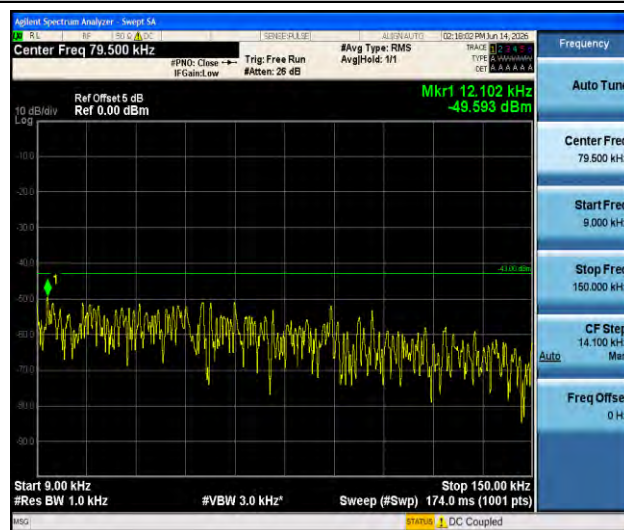
Band66-1.4MHz-QPSK-132322-1RB#0-0.009~0.15-PASS
