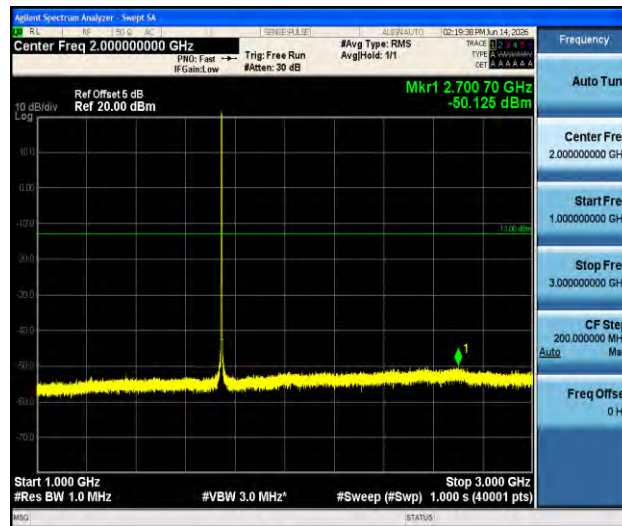
Band66-1.4MHz-16QAM-132322-1RB#0-1000~3000-PASS
