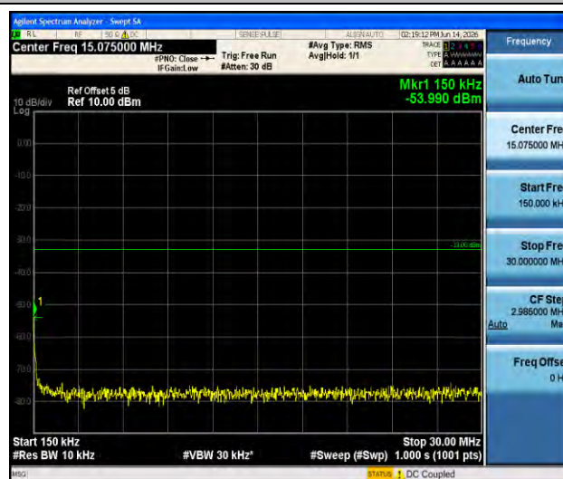
Band66-1.4MHz-16QAM-132322-1RB#0-0.15~30-PASS
