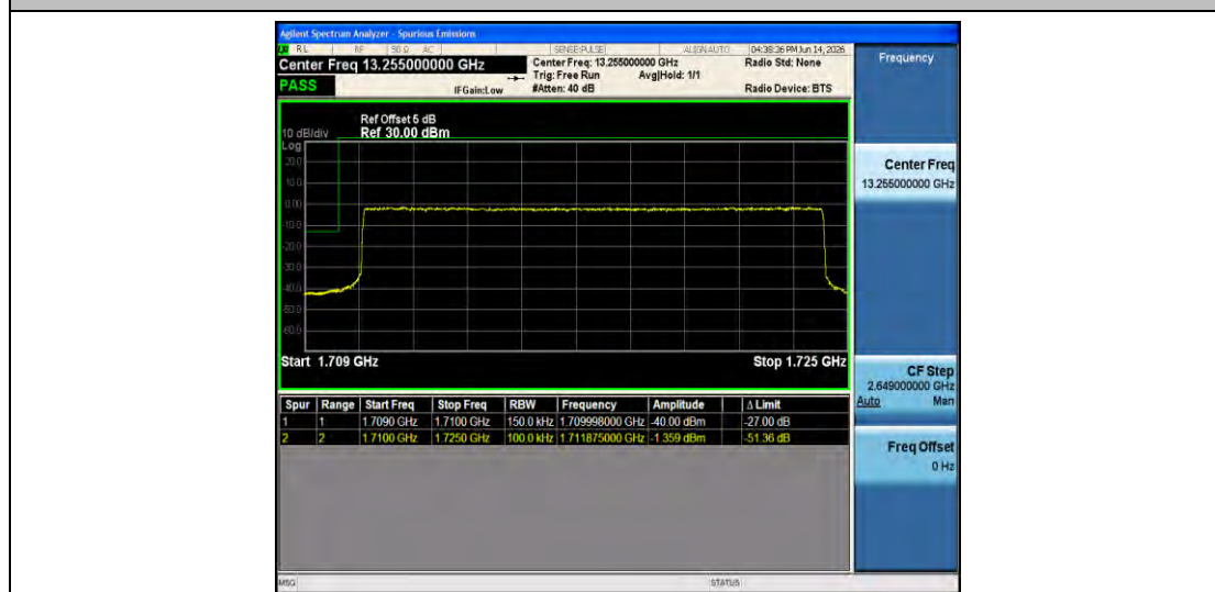
Band66-15MHz-QPSK-132047-75RB#0-PASS
