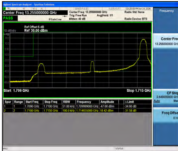
Band66-5MHz-16QAM-131997-1RB#24-PASS
