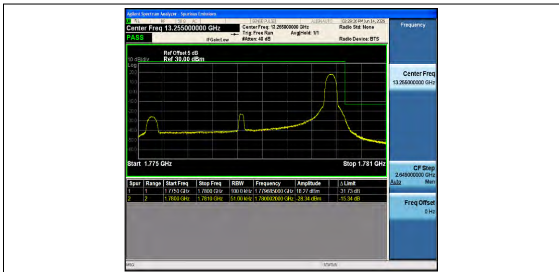
Band66-5MHz-16QAM-132647-1RB#24-PASS
