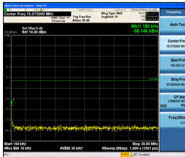
Band66-5MHz-QPSK-131997-1RB#0-0.15~30-PASS
