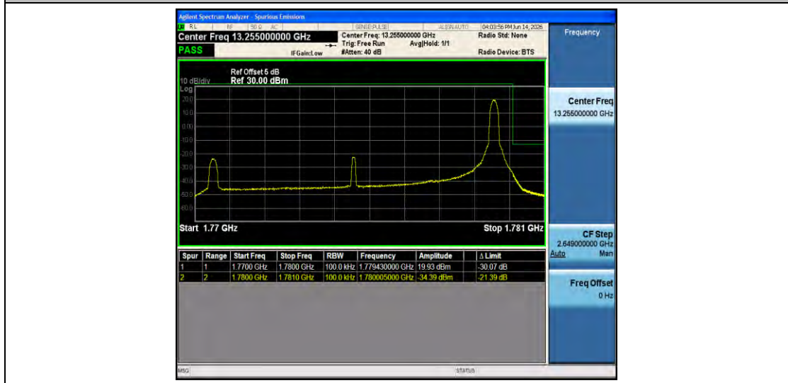
Band66-10MHz-QPSK-132622-1RB#49-PASS
