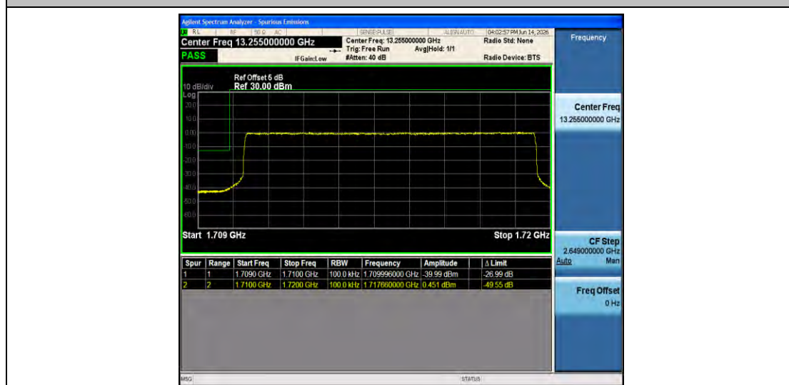
Band66-10MHz-QPSK-132022-50RB#0-PASS
