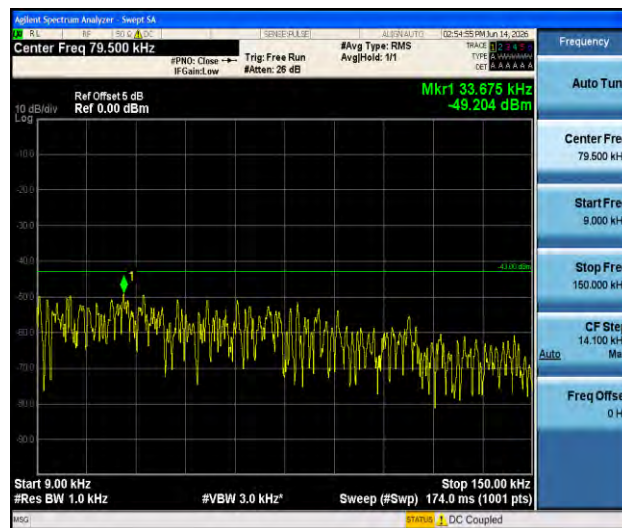
Band66-3MHz-QPSK-131987-1RB#0-0.009~0.15-PASS
