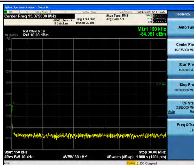
Band66-1.4MHz-16QAM-131979-1RB#0-0.15~30-PASS
