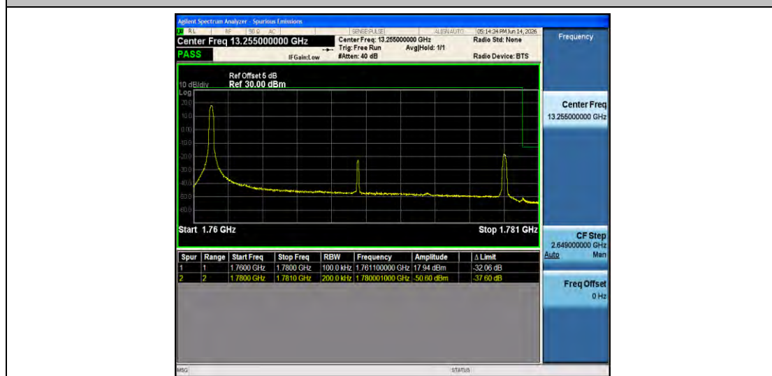
Band66-20MHz-16QAM-132572-1RB#0-PASS
