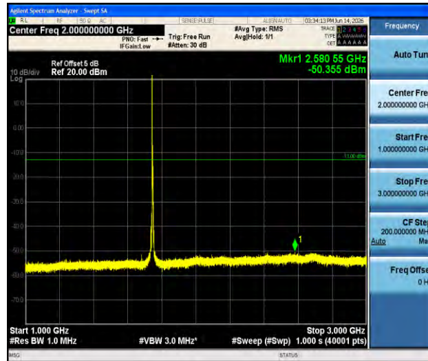
Band66-5MHz-16QAM-132322-1RB#0-1000~3000-PASS
