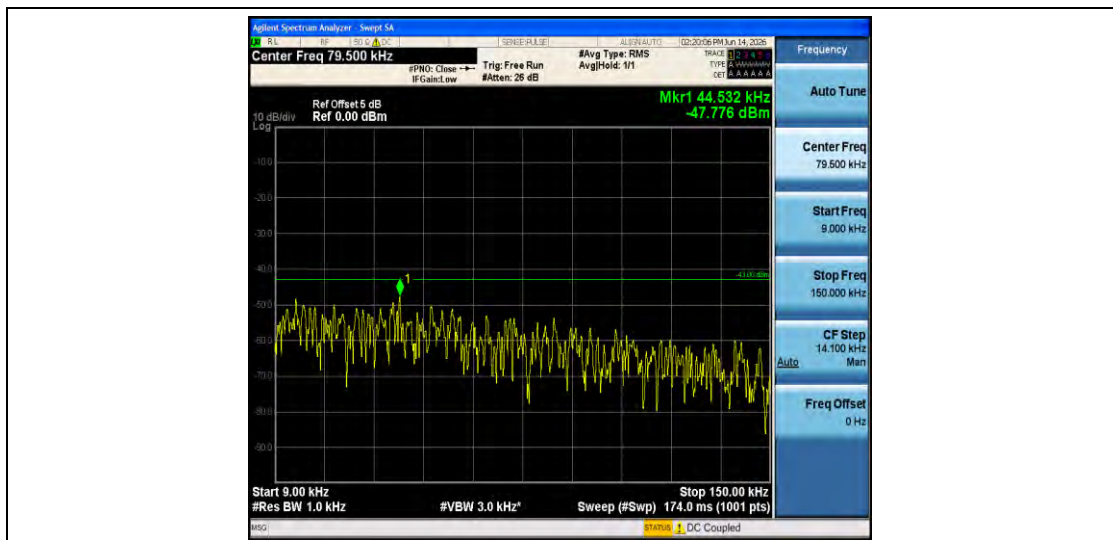
Band66-1.4MHz-QPSK-132665-1RB#0-0.009~0.15-PASS
