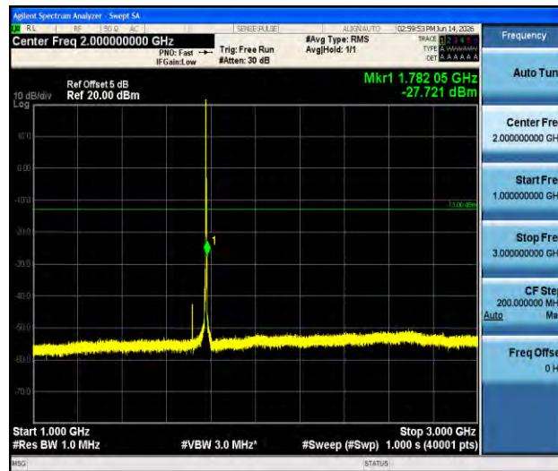
Band66-3MHz-QPSK-132657-1RB#0-1000~3000-PASS
