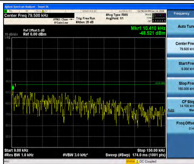
Band66-3MHz-16QAM-131987-1RB#0-0.009~0.15-PASS
