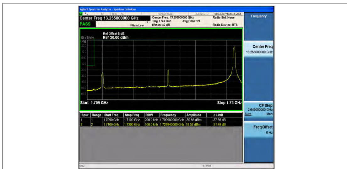
Band66-20MHz-16QAM-132072-1RB#99-PASS
