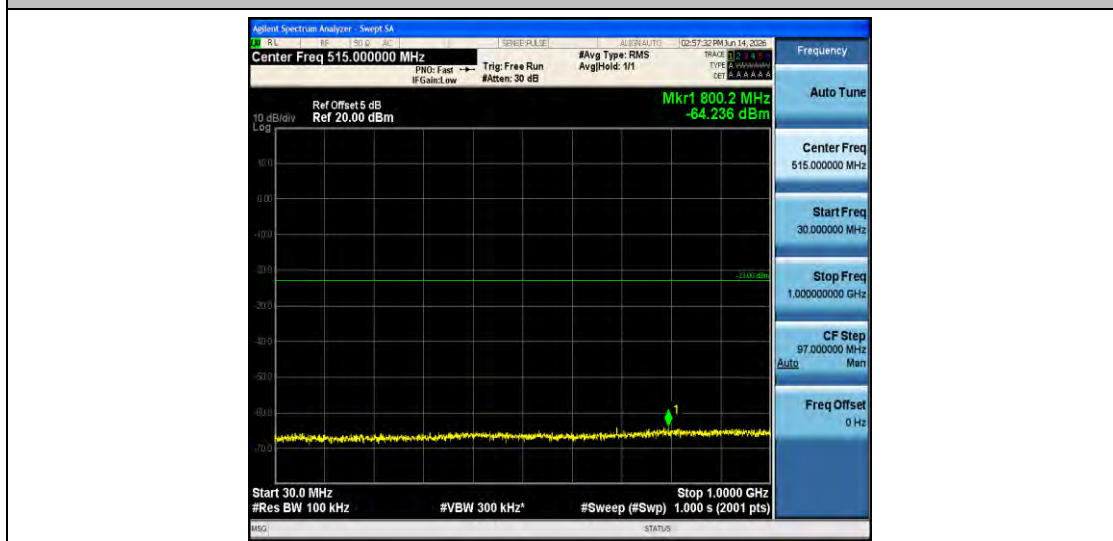
Band66-3MHz-QPSK-132322-1RB#0-30~1000-PASS
