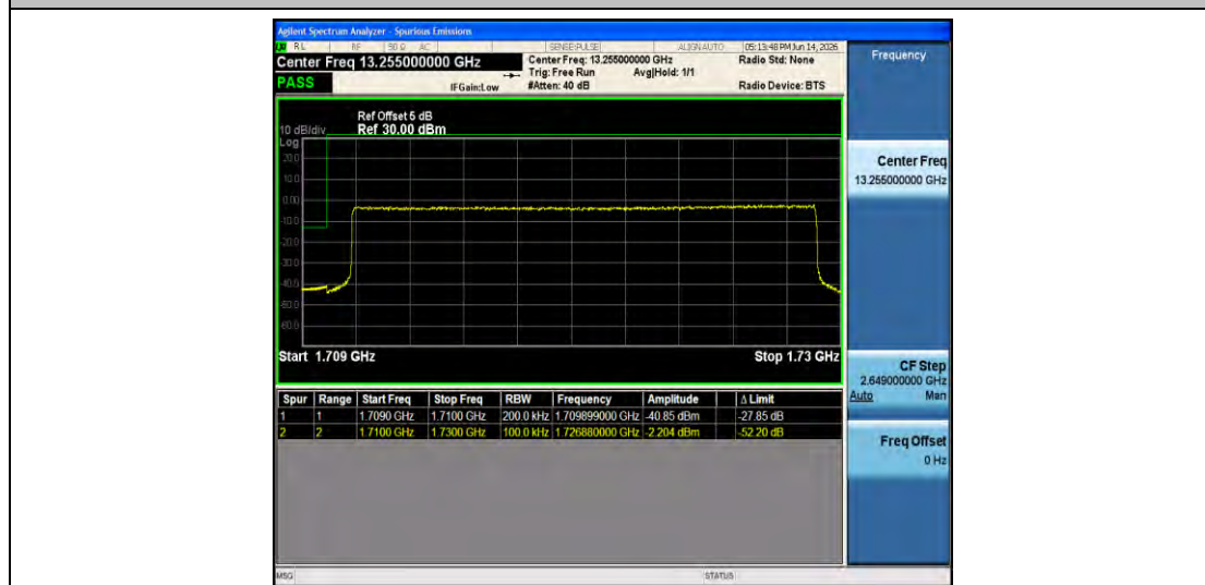
Band66-20MHz-QPSK-132072-100RB#0-PASS
