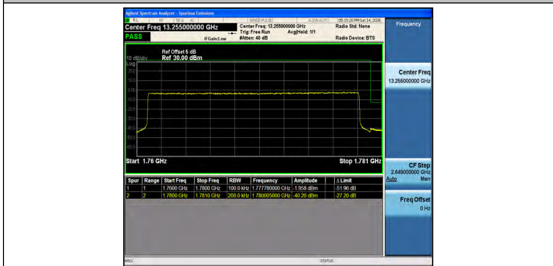
Band66-20MHz-QPSK-132572-100RB#0-PASS
