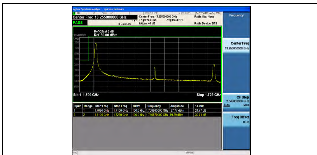
Band66-15MHz-QPSK-132047-1RB#0-PASS
