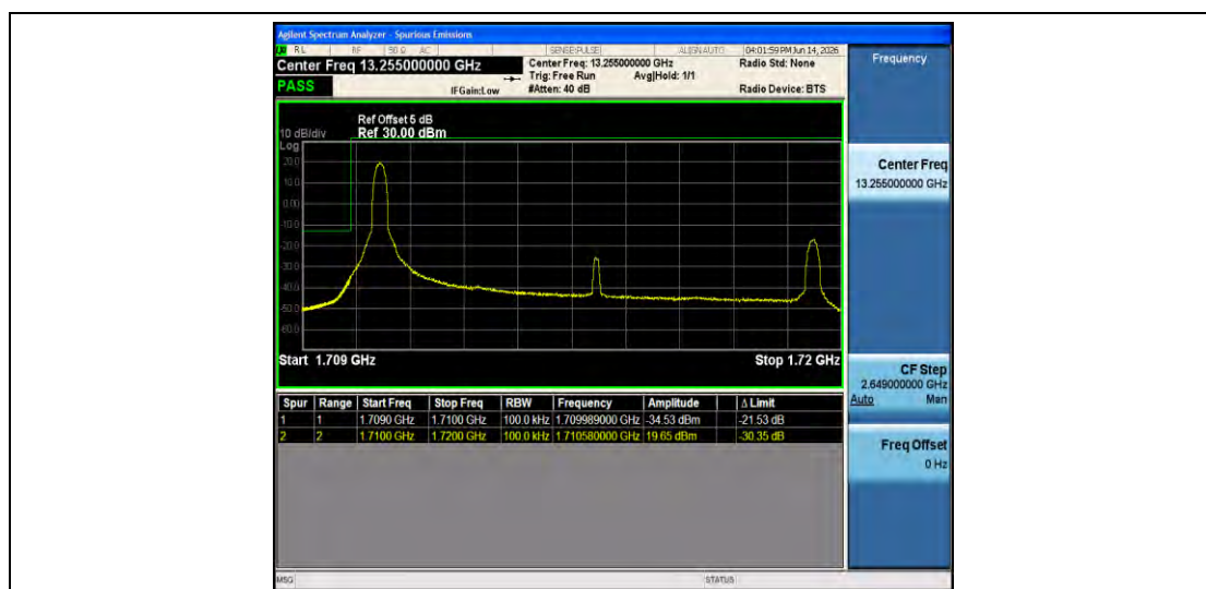
Band66-10MHz-QPSK-132022-1RB#0-PASS
