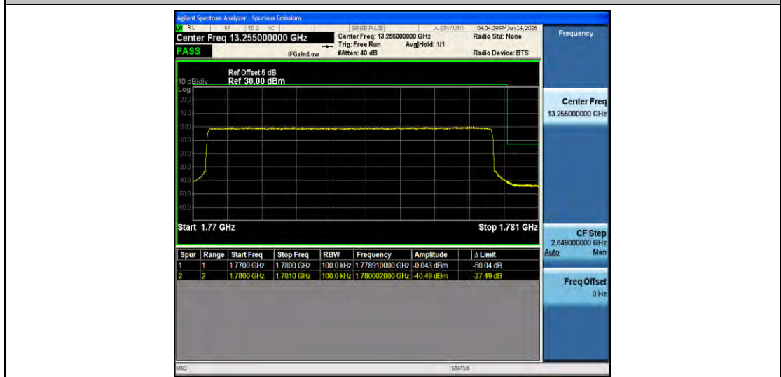
Band66-10MHz-16QAM-132622-50RB#0-PASS
