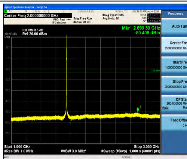
Band66-3MHz-16QAM-132322-1RB#0-1000~3000-PASS
