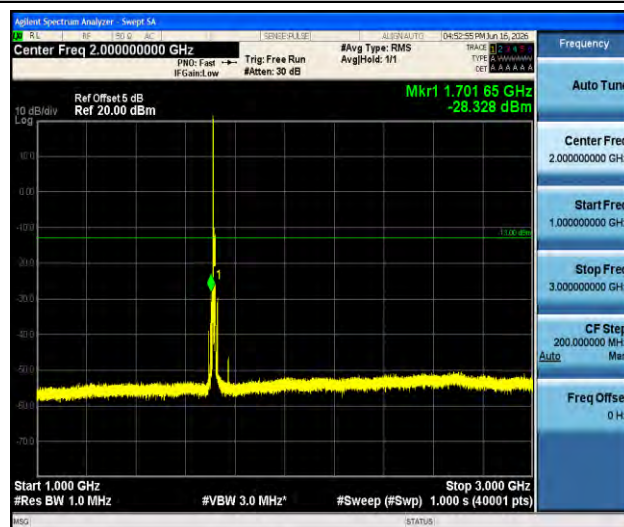
Band66-10MHz-16QAM-132022-1RB#0-1000~3000-PASS
