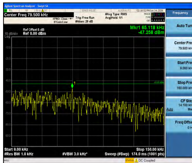
Band66-1.4MHz-16QAM-131979-1RB#0-0.009~0.15-PASS
