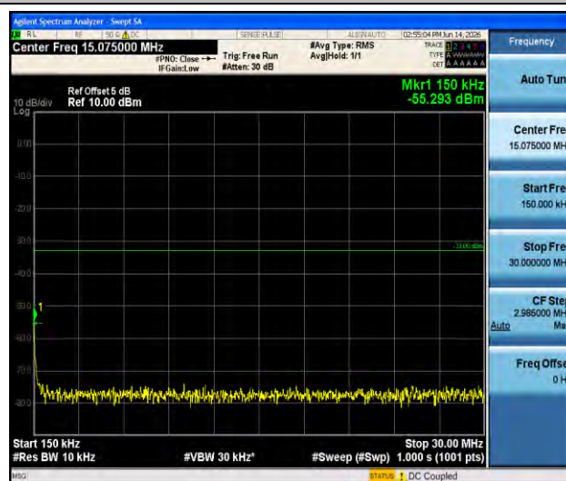
Band66-3MHz-QPSK-131987-1RB#0-0.15~30-PASS
