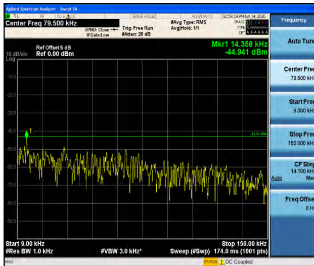
Band66-3MHz-QPSK-132657-1RB#0-0.009~0.15-PASS
