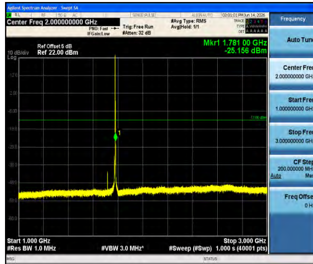
Band66-3MHz-16QAM-132657-1RB#0-1000~3000-PASS
