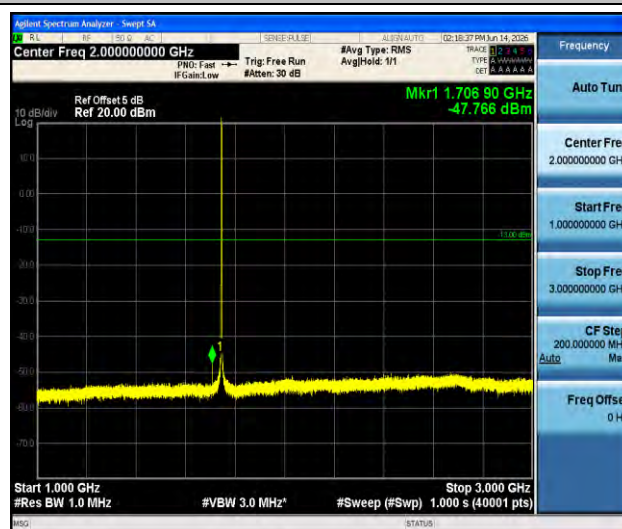
Band66-1.4MHz-QPSK-132322-1RB#0-1000~3000-PASS
