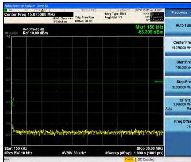
Band66-3MHz-16QAM-132322-1RB#0-0.15~30-PASS
