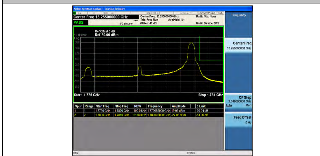
Band66-5MHz-QPSK-132647-1RB#24-PASS
