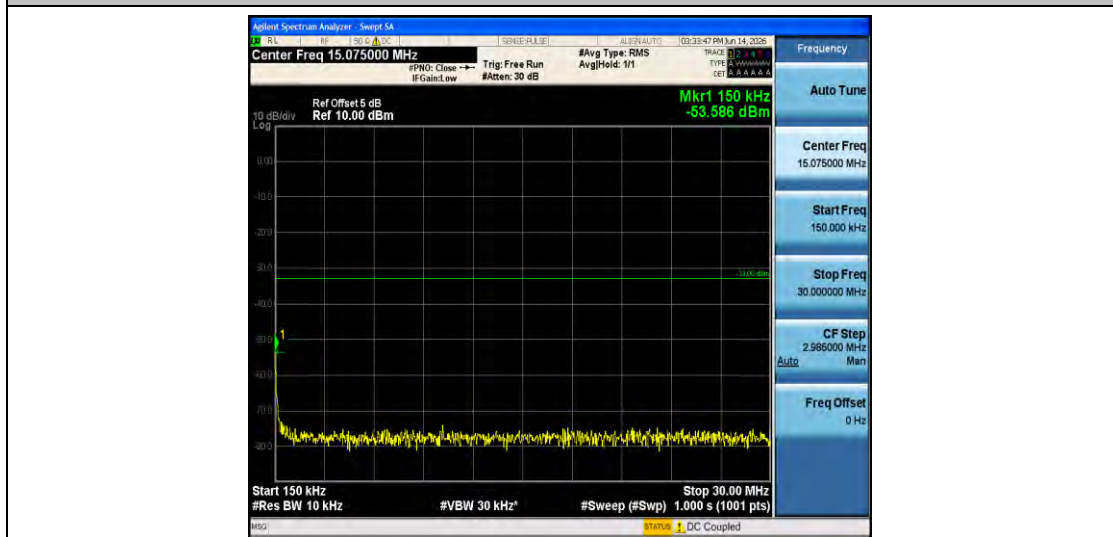
Band66-5MHz-16QAM-132322-1RB#0-0.15~30-PASS
