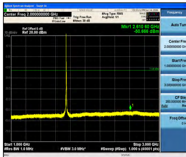
Band66-5MHz-QPSK-132322-1RB#0-1000~3000-PASS
