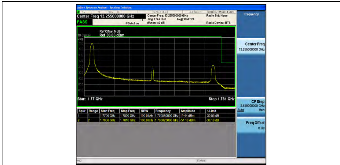
Band66-10MHz-QPSK-132622-1RB#0-PASS
