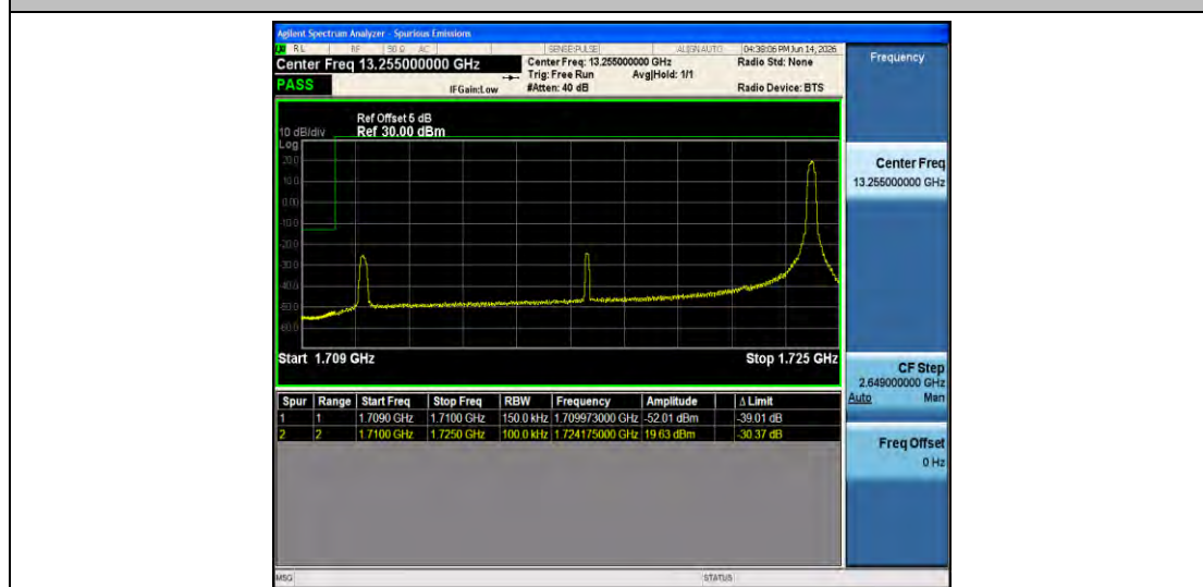
Band66-15MHz-QPSK-132047-1RB#74-PASS
