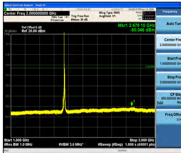
Band66-10MHz-16QAM-132322-1RB#0-1000~3000-PASS
