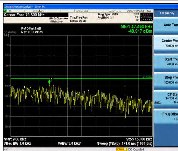
Band66-15MHz-16QAM-132597-1RB#0-0.009~0.15-PASS
