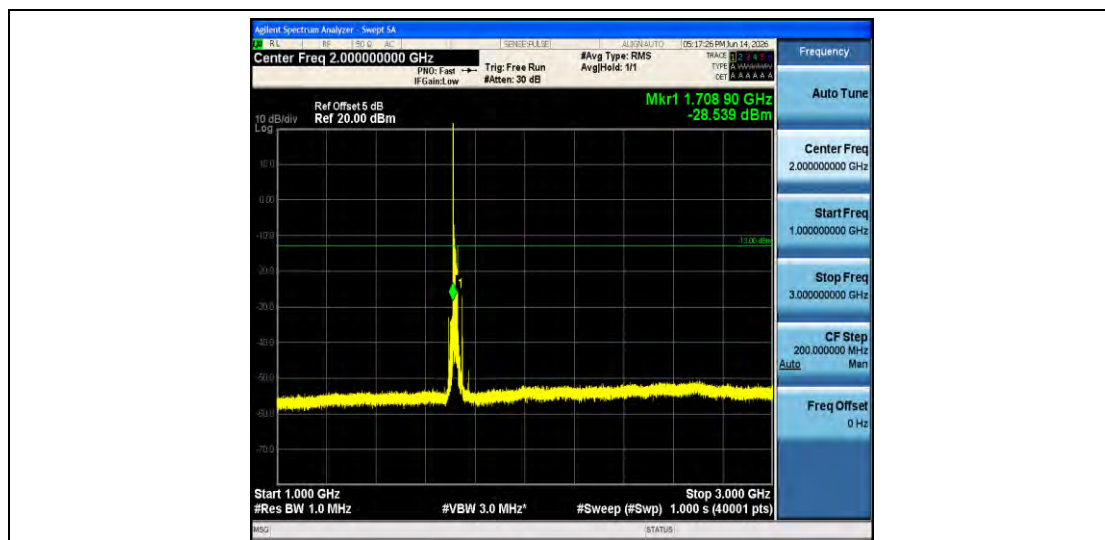
Band66-20MHz-16QAM-132072-1RB#0-1000~3000-PASS
