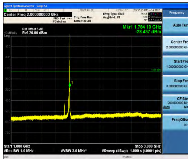
Band66-5MHz-16QAM-132647-1RB#0-1000~3000-PASS
