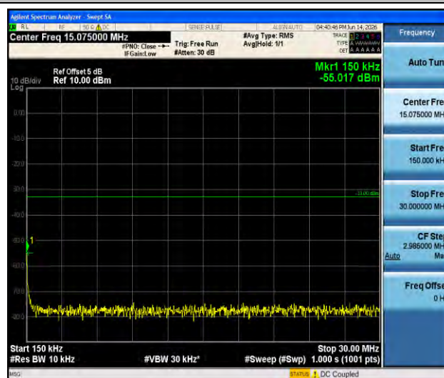
Band66-15MHz-QPSK-132047-1RB#0-0.15~30-PASS
