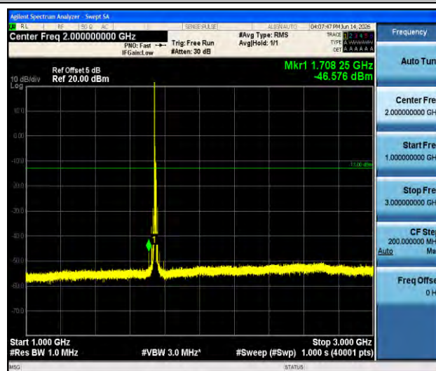
Band66-10MHz-QPSK-132322-1RB#0-1000~3000-PASS
