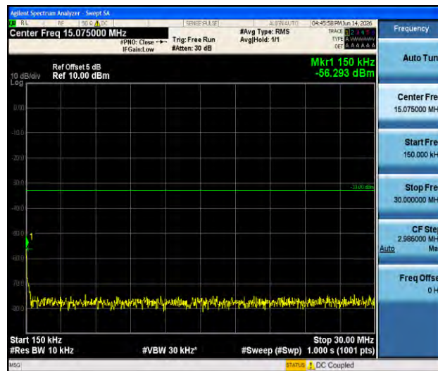
Band66-15MHz-16QAM-132597-1RB#0-0.15~30-PASS
