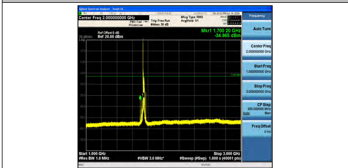
Band66-20MHz-16QAM-132322-1RB#0-1000~3000-PASS
