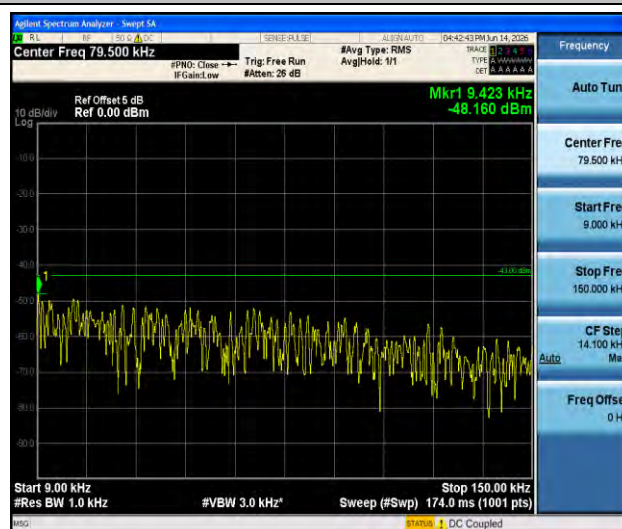
Band66-15MHz-QPSK-132322-1RB#0-0.009~0.15-PASS
