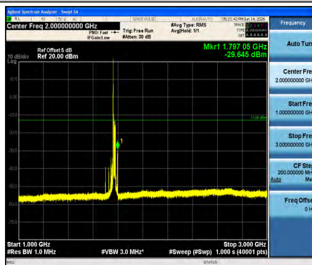
Band66-20MHz-16QAM-132572-1RB#0-1000~3000-PASS
