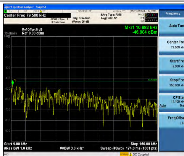
Band66-20MHz-16QAM-132572-1RB#0-0.009~0.15-PASS
