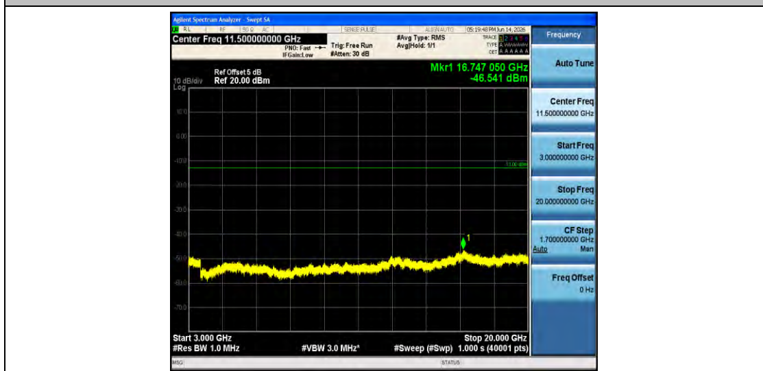
Band66-20MHz-16QAM-132322-1RB#0-3000~20000-PASS
