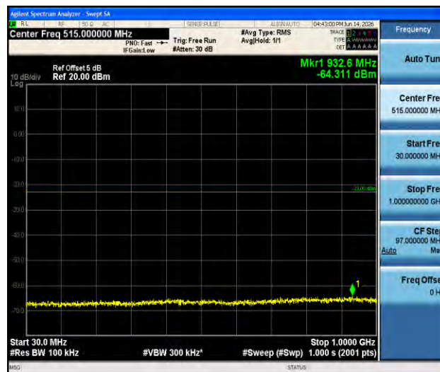
Band66-15MHz-QPSK-132322-1RB#0-30~1000-PASS
