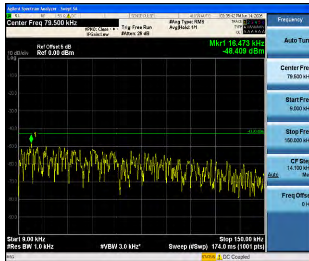
Band66-5MHz-16QAM-132647-1RB#0-0.009~0.15-PASS
