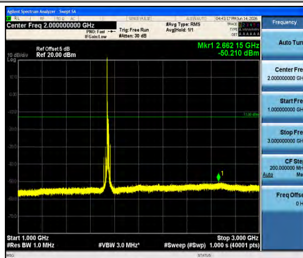
Band66-15MHz-QPSK-132322-1RB#0-1000~3000-PASS
