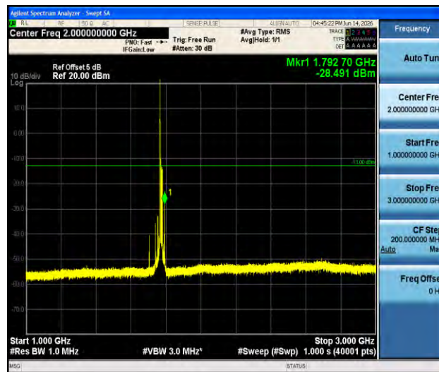
Band66-15MHz-QPSK-132597-1RB#0-1000~3000-PASS
