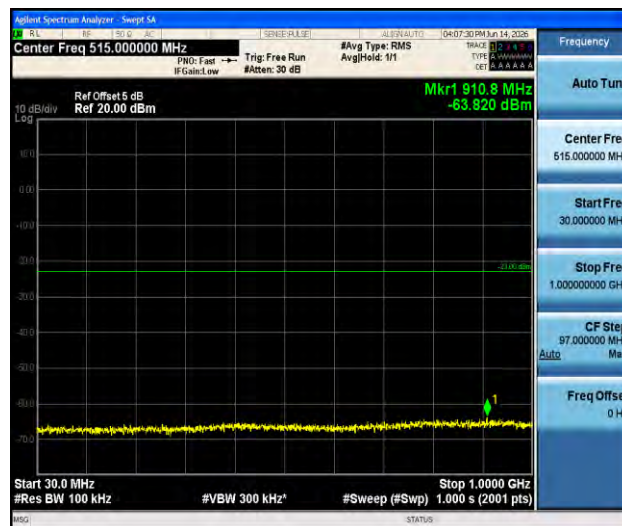
Band66-10MHz-QPSK-132322-1RB#0-30~1000-PASS
