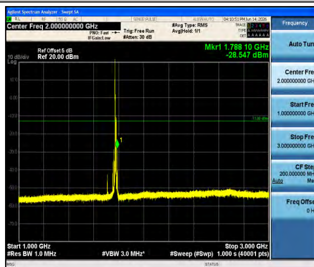
Band66-10MHz-16QAM-132622-1RB#0-1000~3000-PASS
