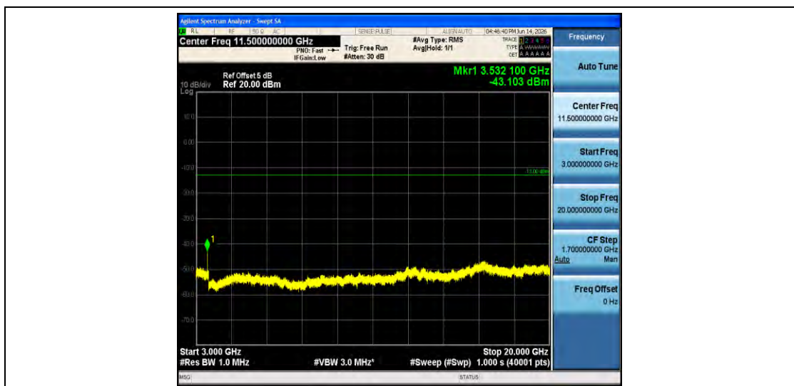
Band66-15MHz-16QAM-132597-1RB#0-3000~20000-PASS
