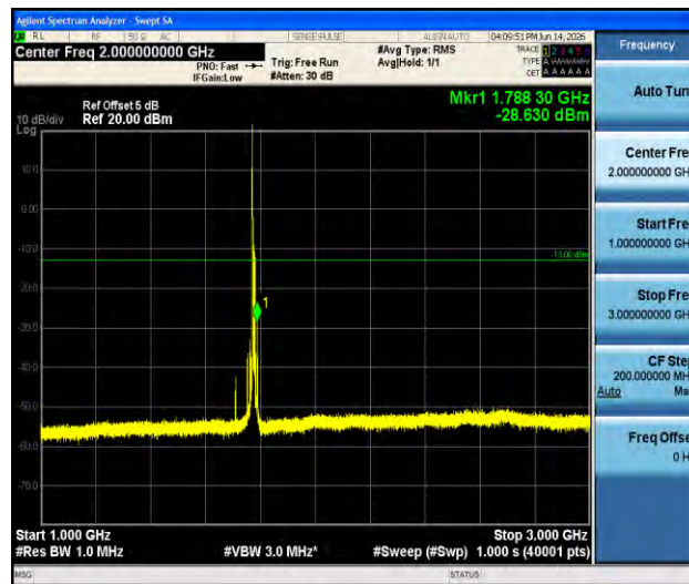
Band66-10MHz-QPSK-132622-1RB#0-1000~3000-PASS
