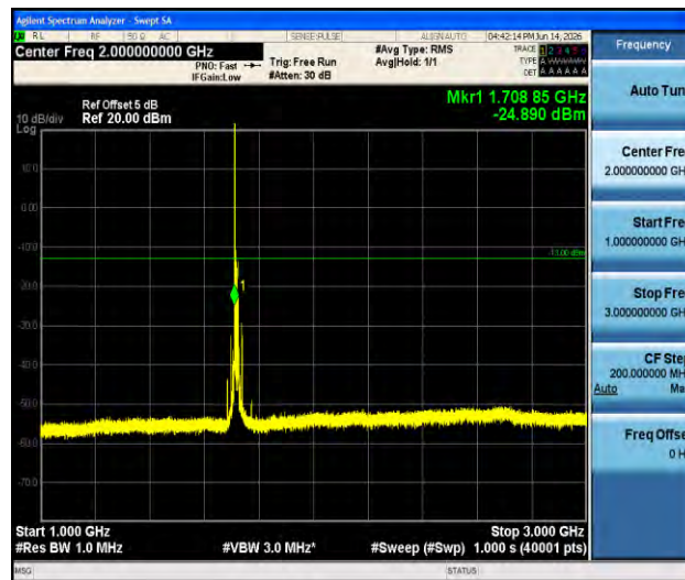
Band66-15MHz-16QAM-132047-1RB#0-1000~3000-PASS
