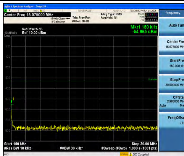
Band66-5MHz-16QAM-132647-1RB#0-0.15~30-PASS
