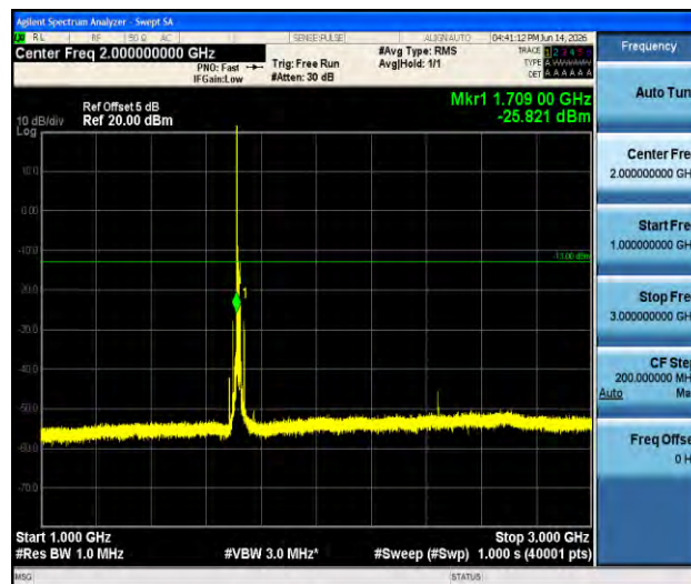
Band66-15MHz-QPSK-132047-1RB#0-1000~3000-PASS
