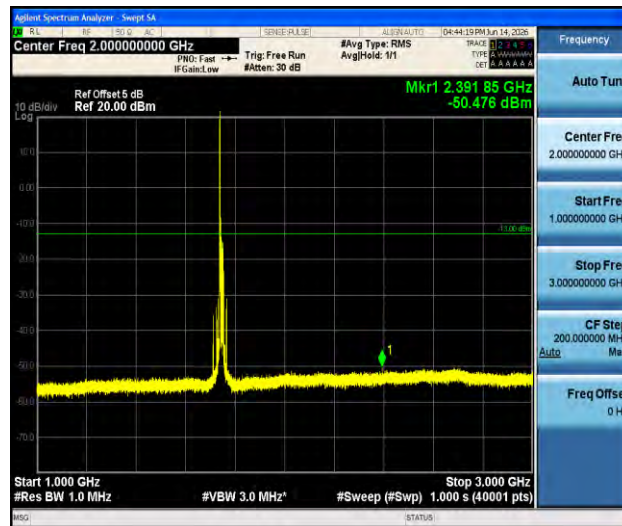
Band66-15MHz-16QAM-132322-1RB#0-1000~3000-PASS
