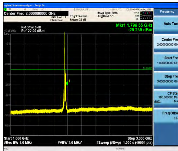
Band66-20MHz-QPSK-132572-1RB#0-1000~3000-PASS
