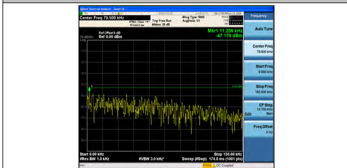
Band66-20MHz-QPSK-132322-1RB#0-0.009~0.15-PASS
