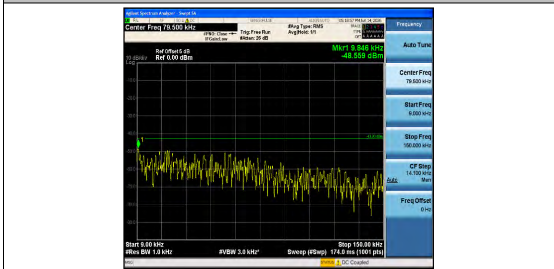
Band66-20MHz-16QAM-132322-1RB#0-0.009~0.15-PASS
