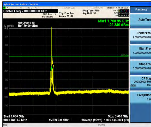
Band66-20MHz-QPSK-132072-1RB#0-1000~3000-PASS
