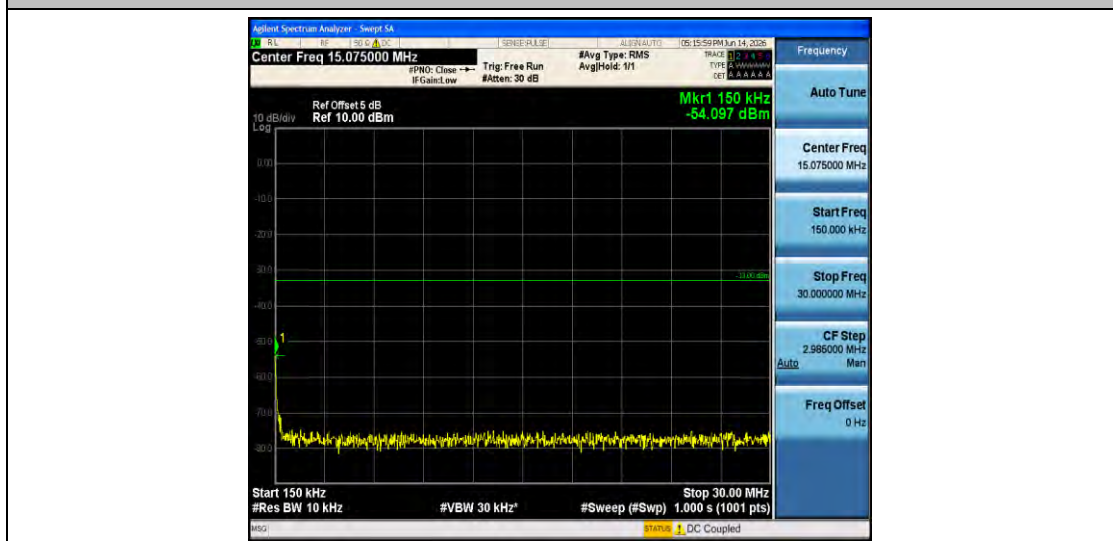
Band66-20MHz-QPSK-132072-1RB#0-0.15~30-PASS
