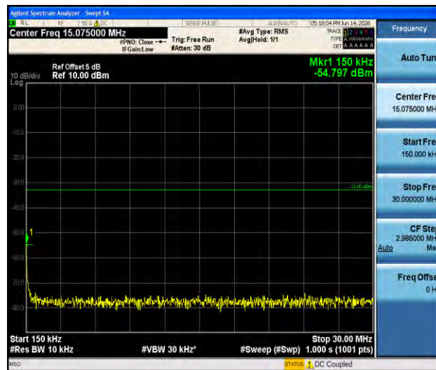
Band66-20MHz-QPSK-132322-1RB#0-0.15~30-PASS
