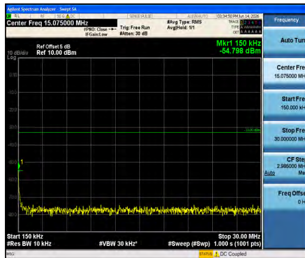
Band66-5MHz-QPSK-132647-1RB#0-0.15~30-PASS
