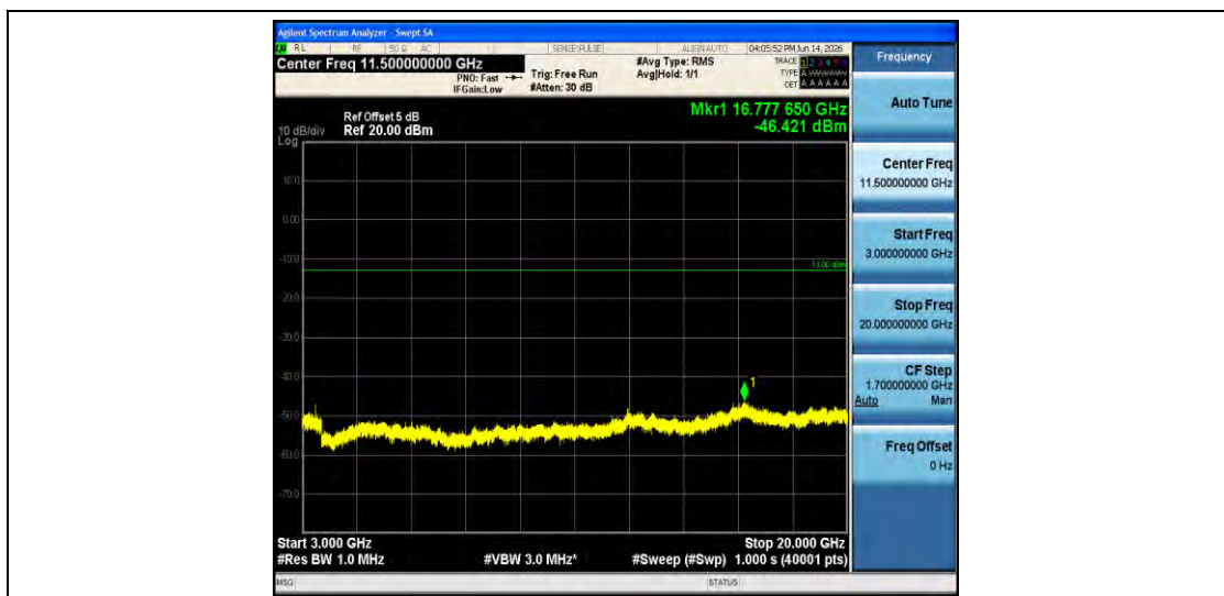
Band66-10MHz-QPSK-132022-1RB#0-3000~20000-PASS
