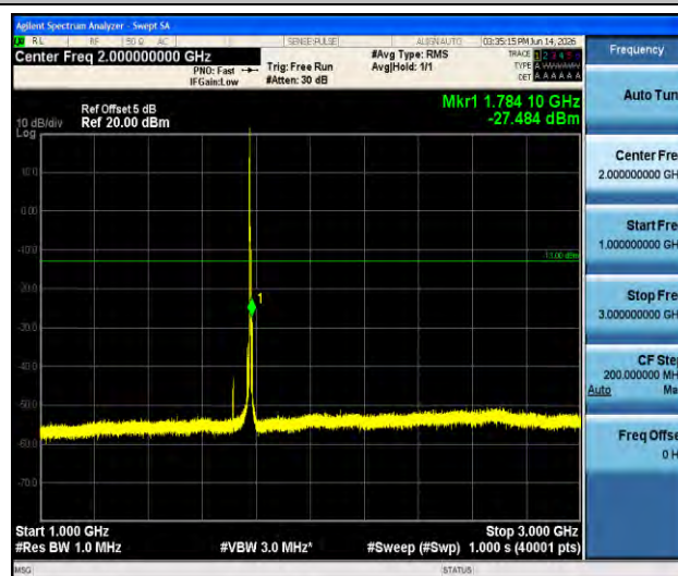
Band66-5MHz-QPSK-132647-1RB#0-1000~3000-PASS
