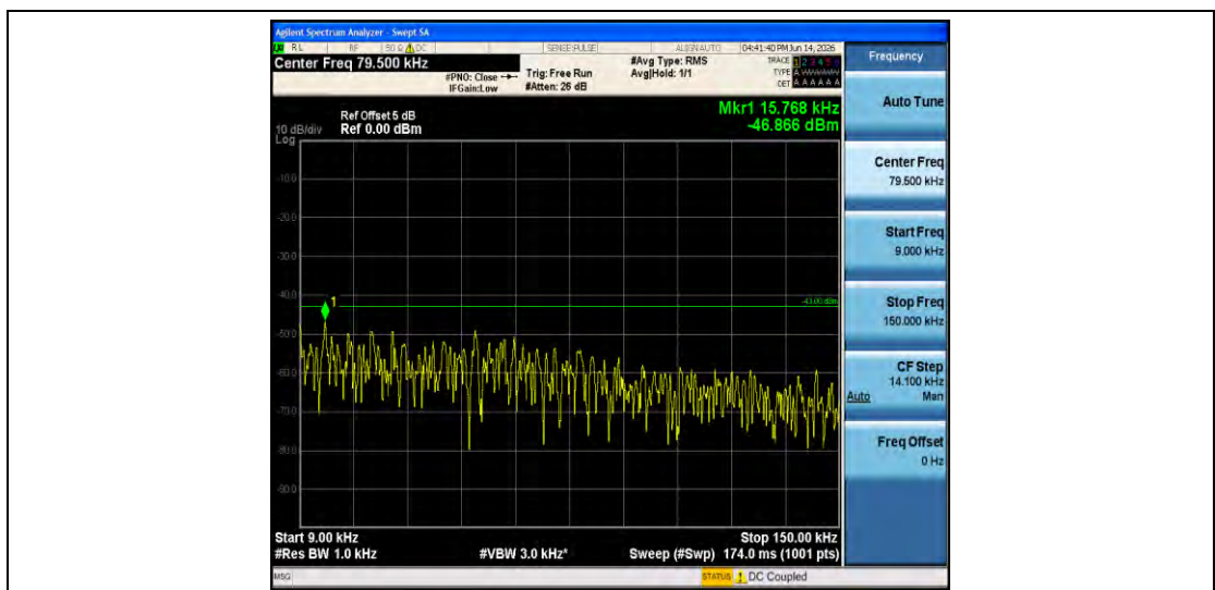
Band66-15MHz-16QAM-132047-1RB#0-0.009~0.15-PASS
