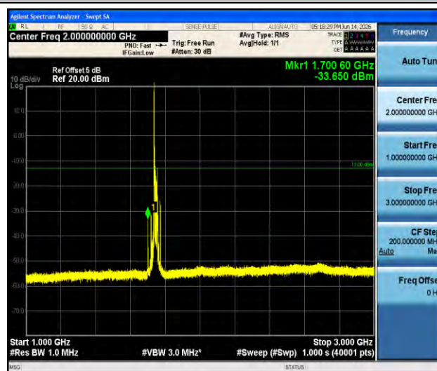
Band66-20MHz-QPSK-132322-1RB#0-1000~3000-PASS
