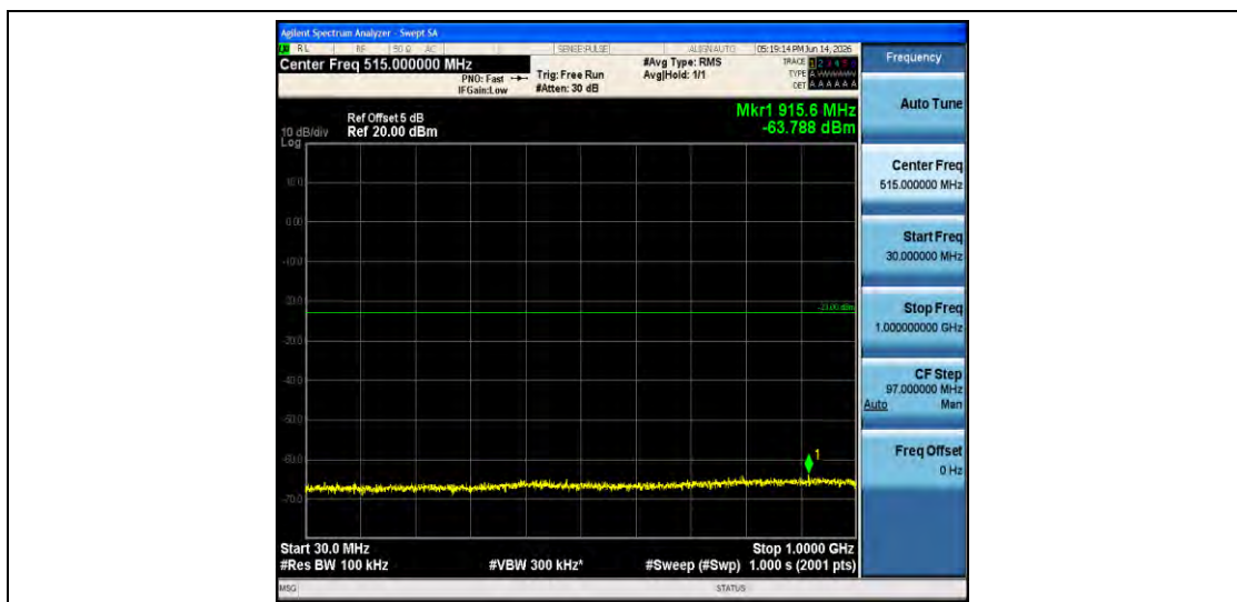
Band66-20MHz-16QAM-132322-1RB#0-30~1000-PASS
