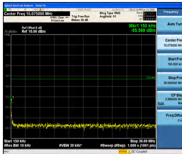
Band66-20MHz-16QAM-132572-1RB#0-0.15~30-PASS
