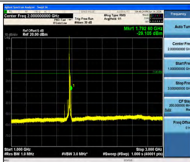
Band66-15MHz-16QAM-132597-1RB#0-1000~3000-PASS
