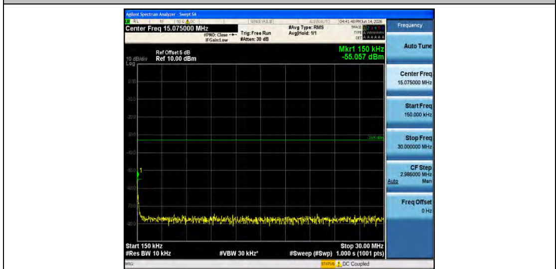
Band66-15MHz-16QAM-132047-1RB#0-0.15~30-PASS
