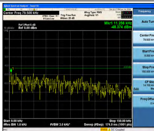
Band66-10MHz-16QAM-132622-1RB#0-0.009~0.15-PASS
