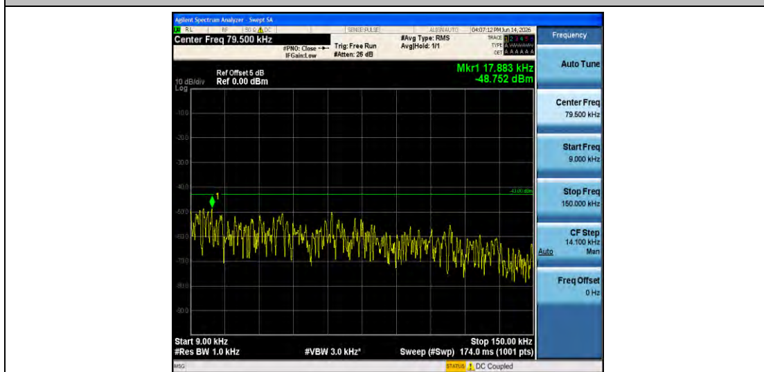
Band66-10MHz-QPSK-132322-1RB#0-0.009~0.15-PASS
