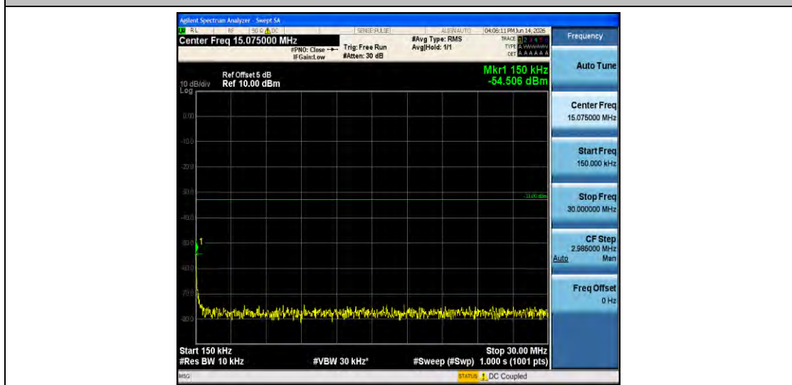
Band66-10MHz-16QAM-132022-1RB#0-0.15~30-PASS
