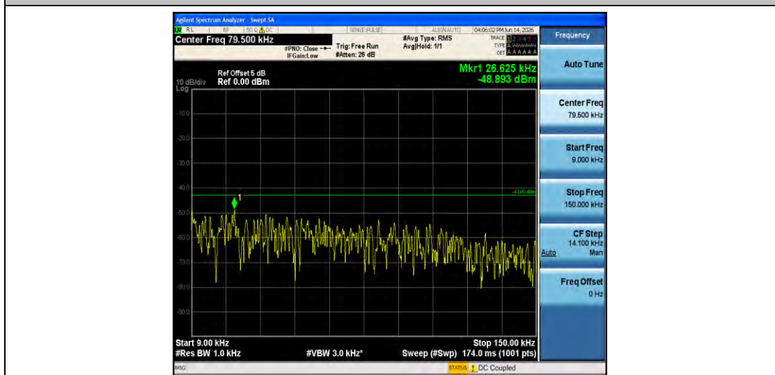
Band66-10MHz-16QAM-132022-1RB#0-0.009~0.15-PASS
