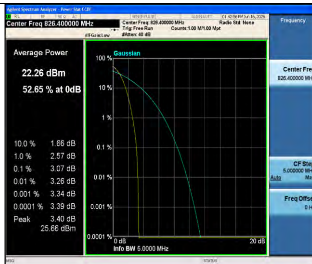
Band5-4132-1-PASS
