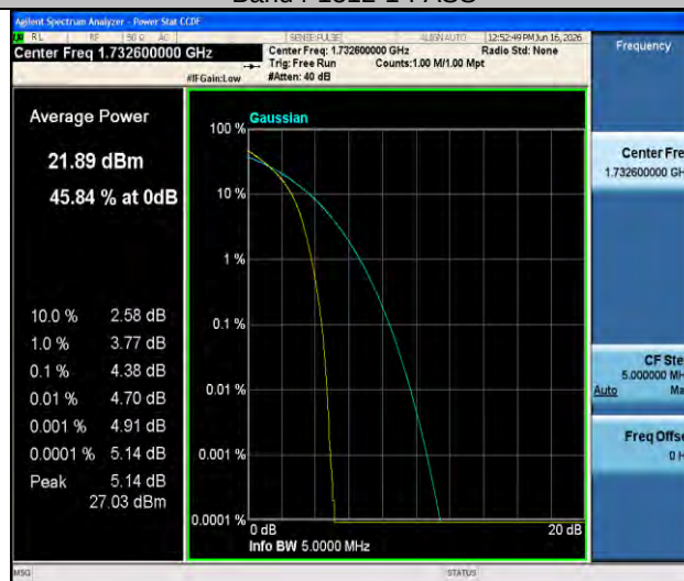
Band4-1413-1-PASS
