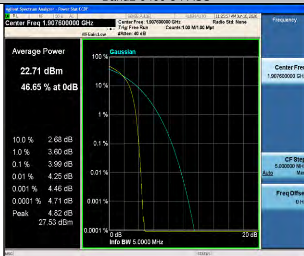
Band2-9538-5-PASS
