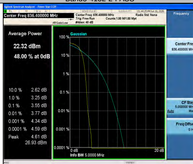
Band5-4182-2-PASS
