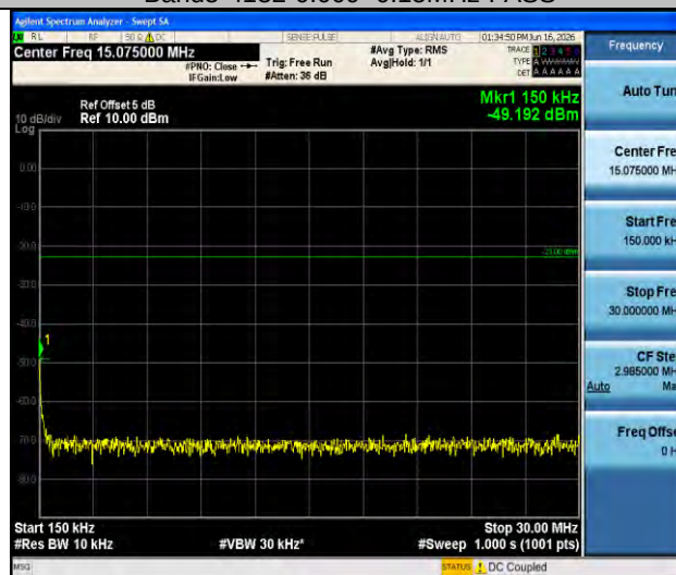
Band5-4132-0.15~30MHz-PASS
