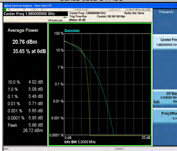
Band2-9400-2-PASS
