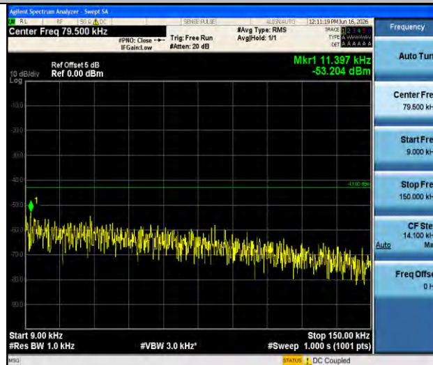
Band4-1513-0.009~0.15MHz-PASS
