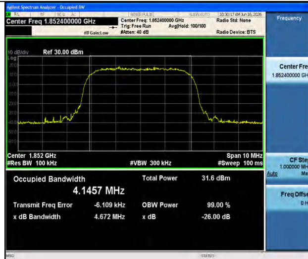
Band2-9262-PASS
