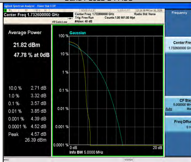
Band4-1413-2-PASS
