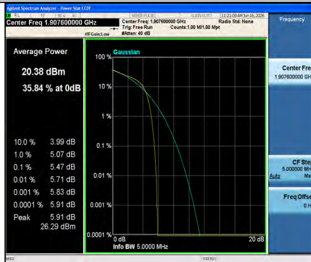
Band2-9538-2-PASS
