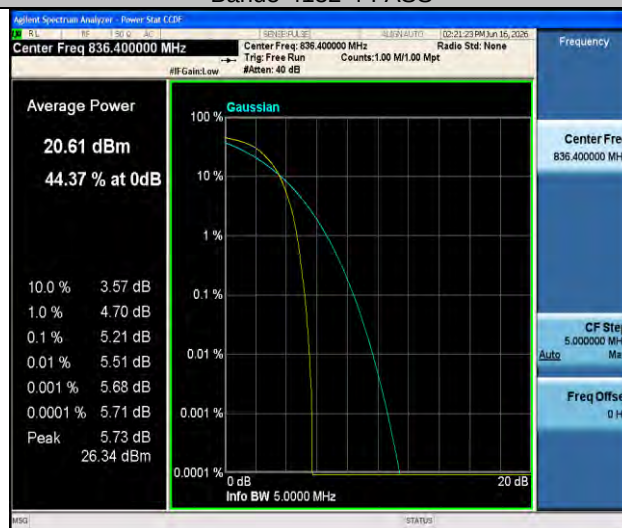
Band5-4182-4-PASS
