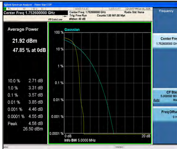
Band4-1513-2-PASS
