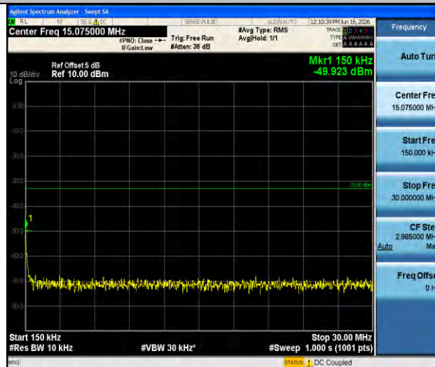
Band4-1413-0.15~30MHz-PASS
