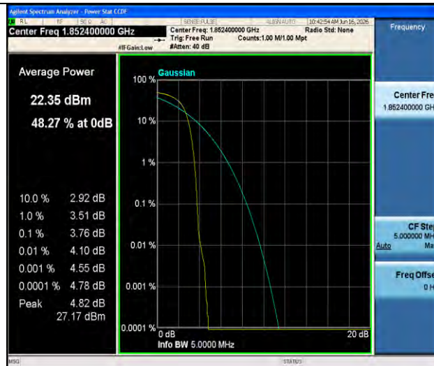
Band2-9262-3-PASS
