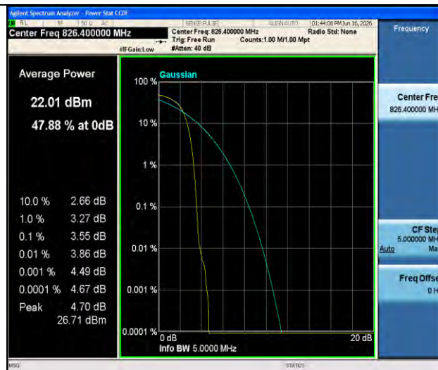
Band5-4132-2-PASS
