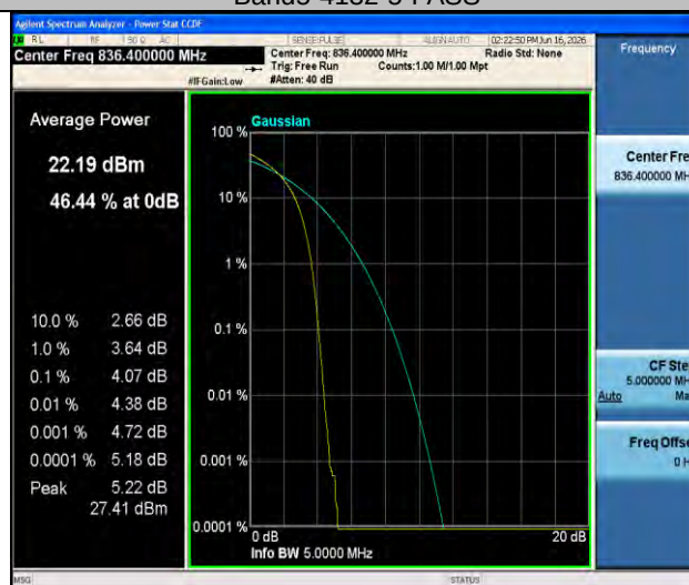
Band5-4182-5-PASS
