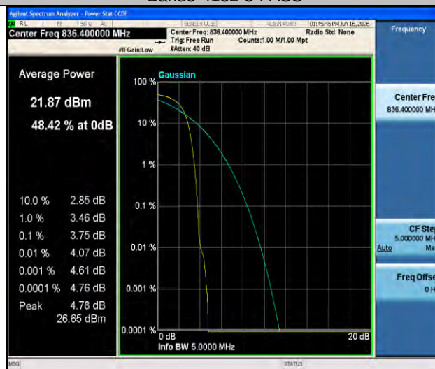
Band5-4182-3-PASS
