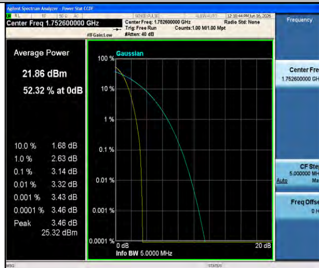
Band4-1513-1-PASS
