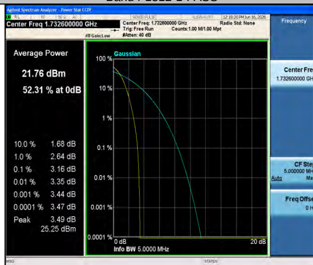
Band4-1413-1-PASS
