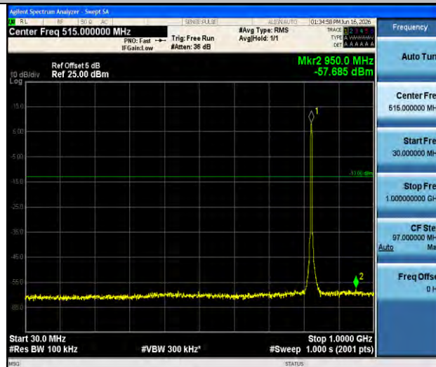
Band5-4132-30~1000MHz-PASS
