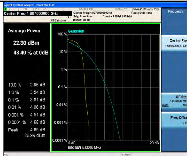
Band2-9538-4-PASS
