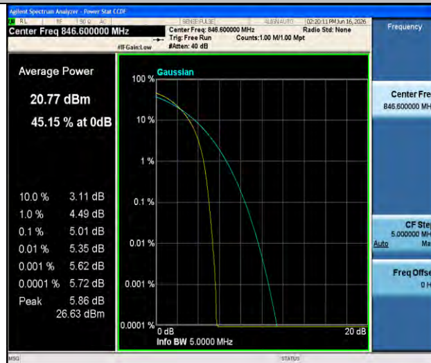
Band5-4233-3-PASS
