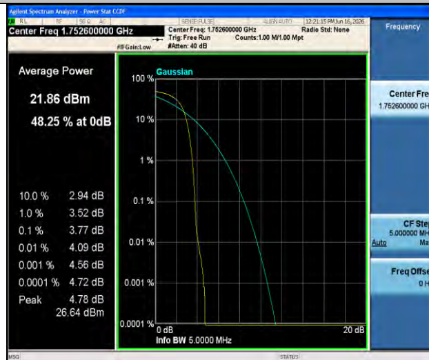
Band4-1513-3-PASS
