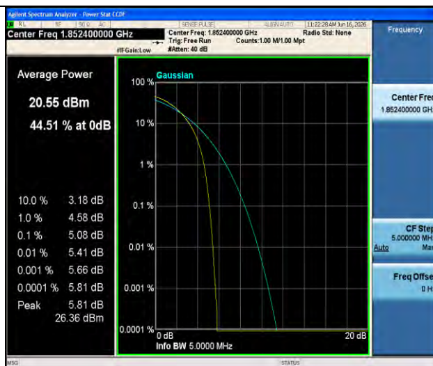
Band2-9262-3-PASS
