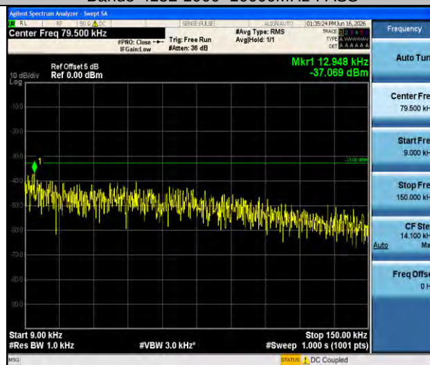
Band5-4182-0.009~0.15MHz-PASS
