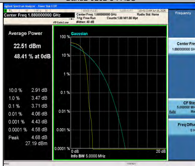
Band2-9400-3-PASS
