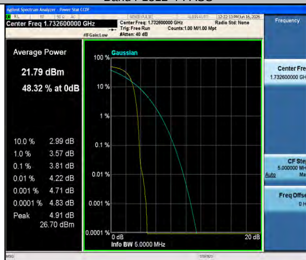
Band4-1413-4-PASS
