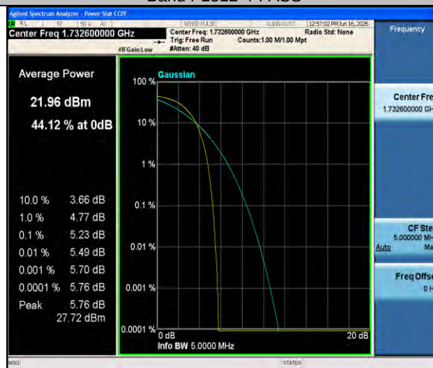
Band4-1413-4-PASS
