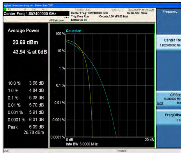
Band2-9262-4-PASS
