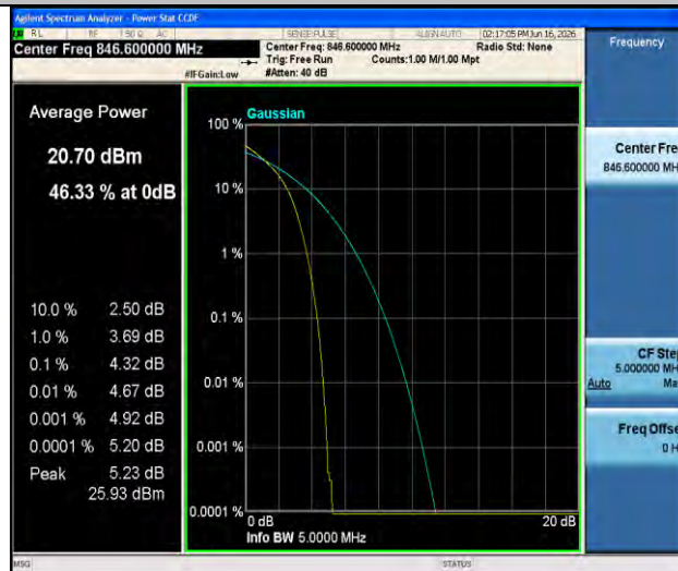
Band5-4233-1-PASS
