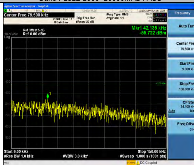
Band4-1413-0.009~0.15MHz-PASS
