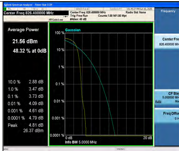
Band5-4132-3-PASS
