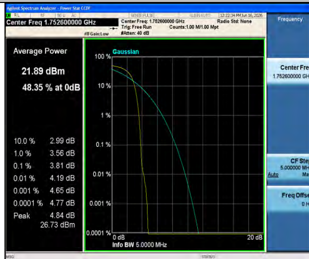
Band4-1513-4-PASS
