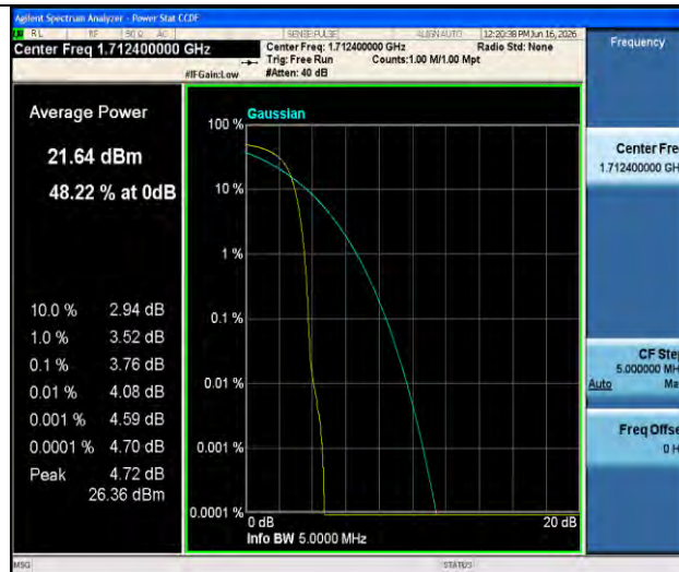
Band4-1312-3-PASS
