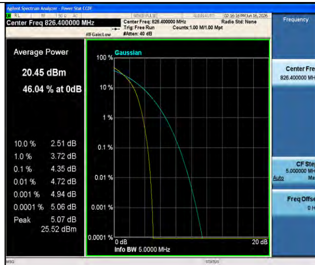
Band5-4132-1-PASS
