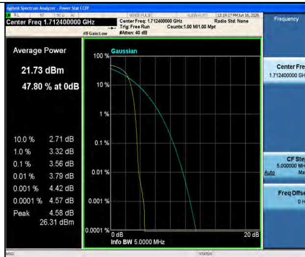
Band4-1312-2-PASS
