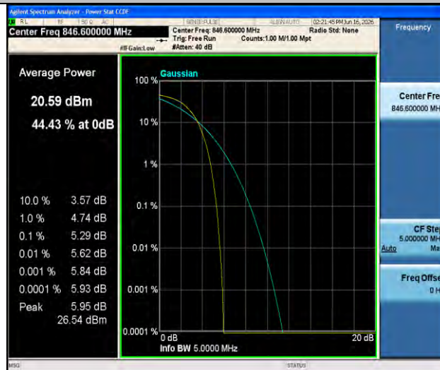
Band5-4233-4-PASS
