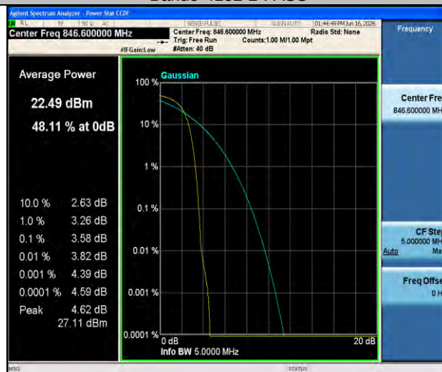
Band5-4233-2-PASS
