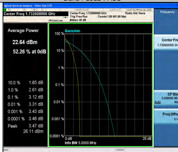
Band4-1413-PASS
