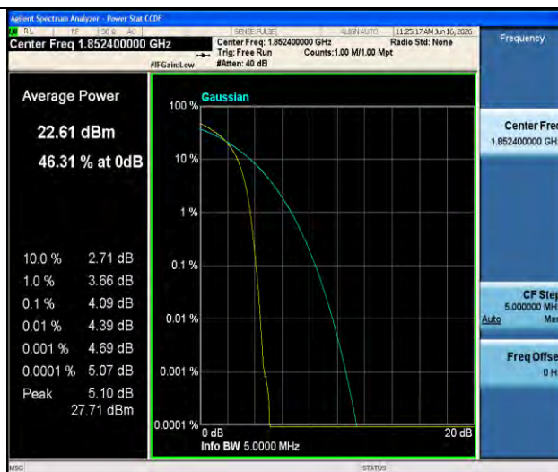
Band2-9262-5-PASS
