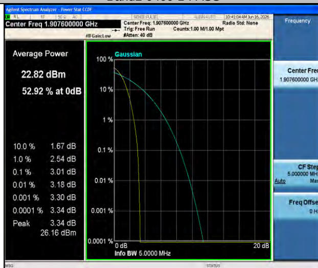
Band2-9538-1-PASS
