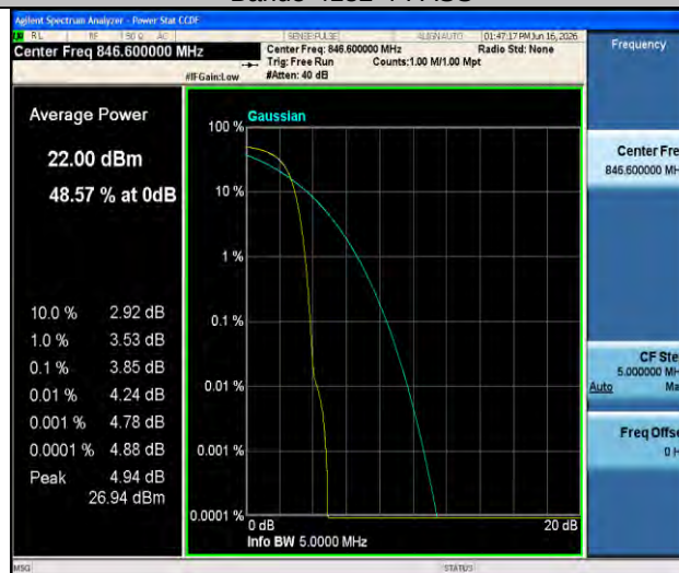
Band5-4233-4-PASS
