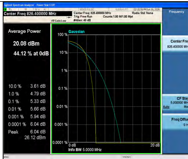
Band5-4132-4-PASS
