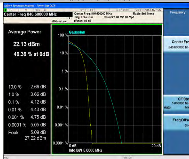
Band5-4233-5-PASS
