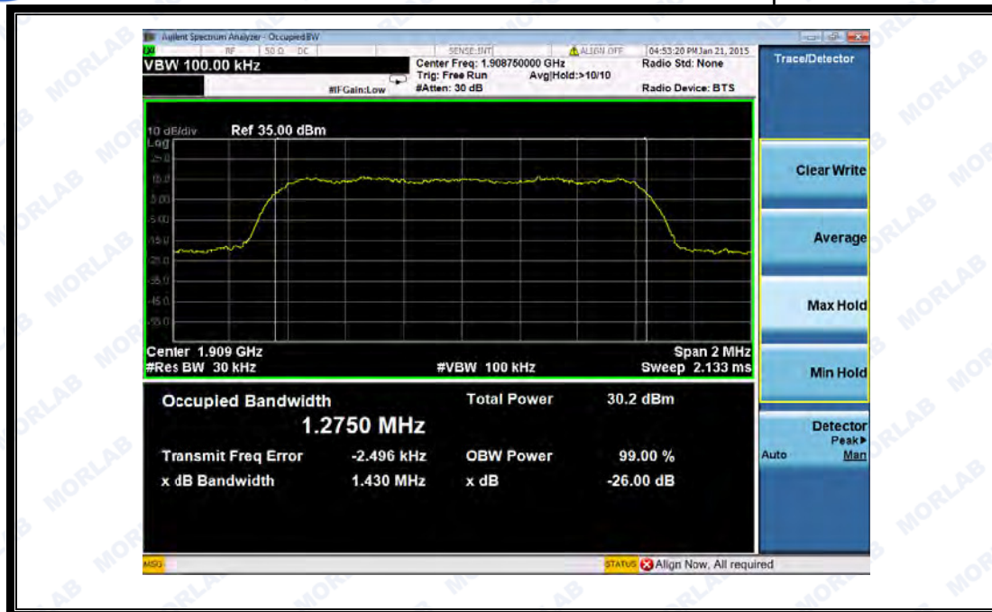
(Plot I: CDMA 1900MHz: BC 1 Channel = 1175)
