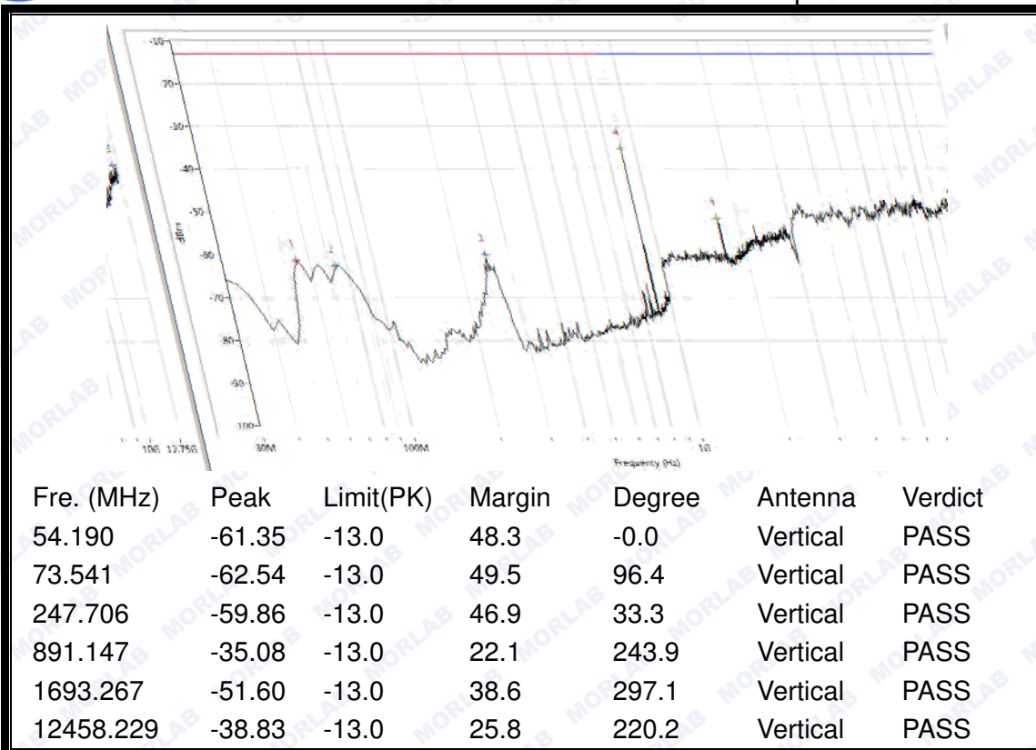
(Plot C.2: CDMA 800MHz: BC 0 Channel = 777, Test Antenna Vertical)
