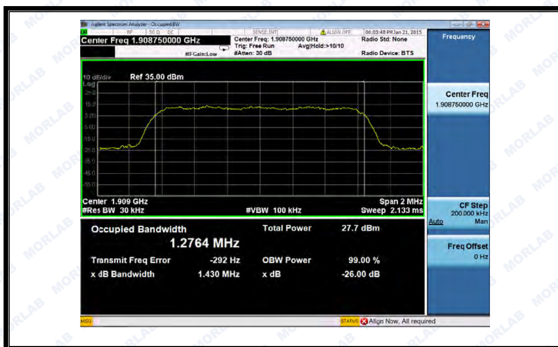
(Plot L: EVDO 0 1900MHz: BC 1 Channel = 1175)
