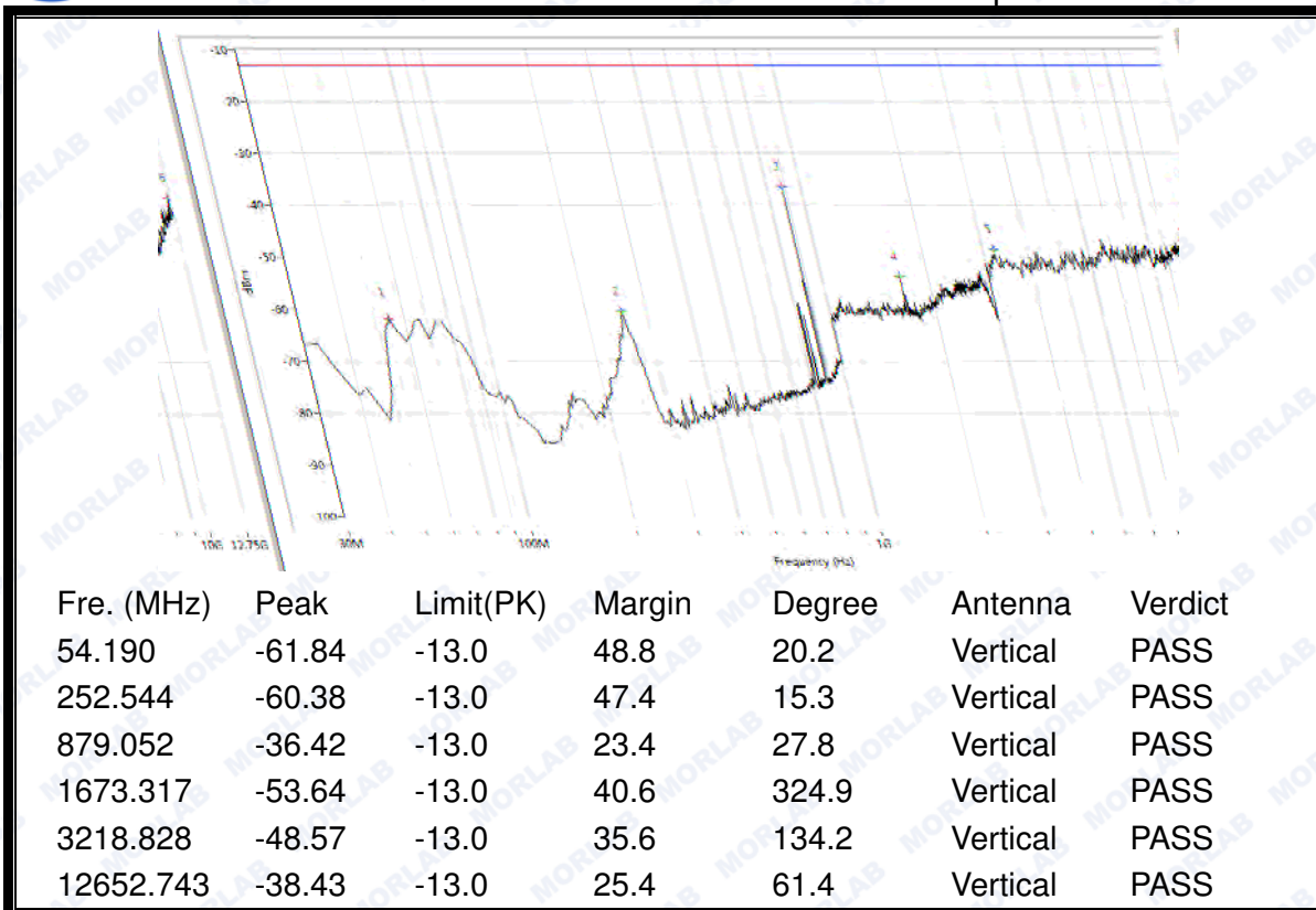
(Plot B.2: CDMA 800MHz: BC 0 Channel = 384, Test Antenna Vertical)
