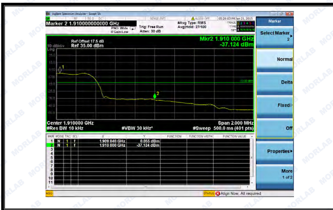
(Plot D: CDMA 1900MHz: BC 0 Channel = 1175)
