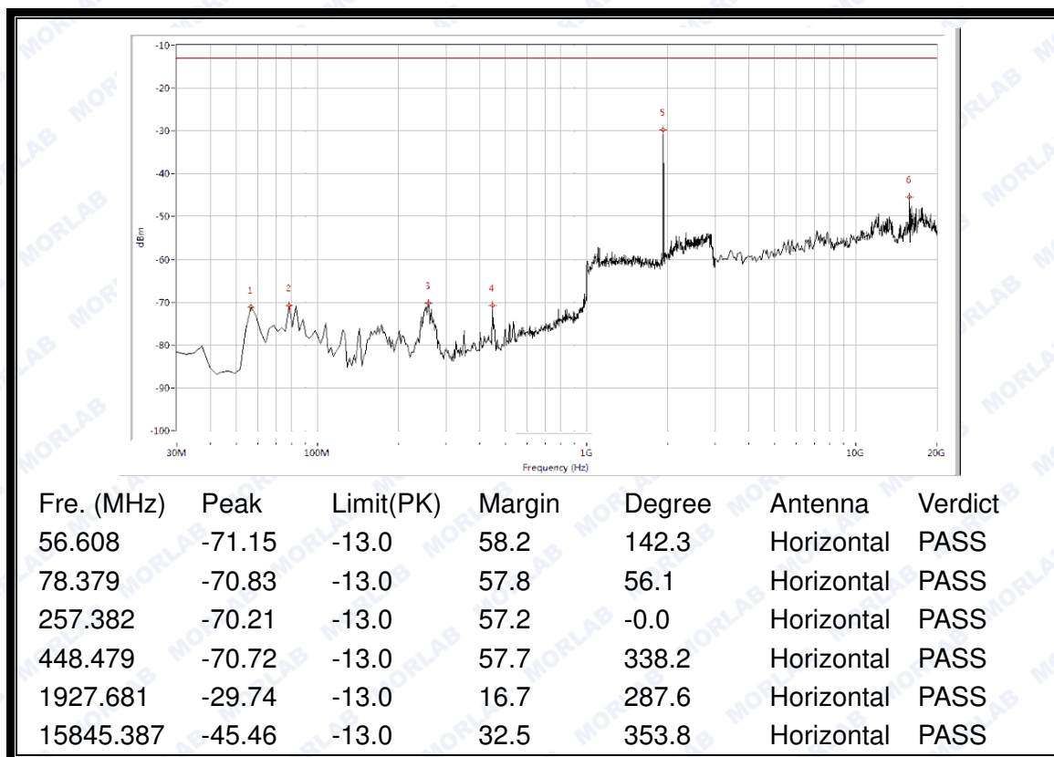
(Plot D.1: CDMA 1900MHz: BC 1 Channel = 25, Test Antenna Horizontal)
