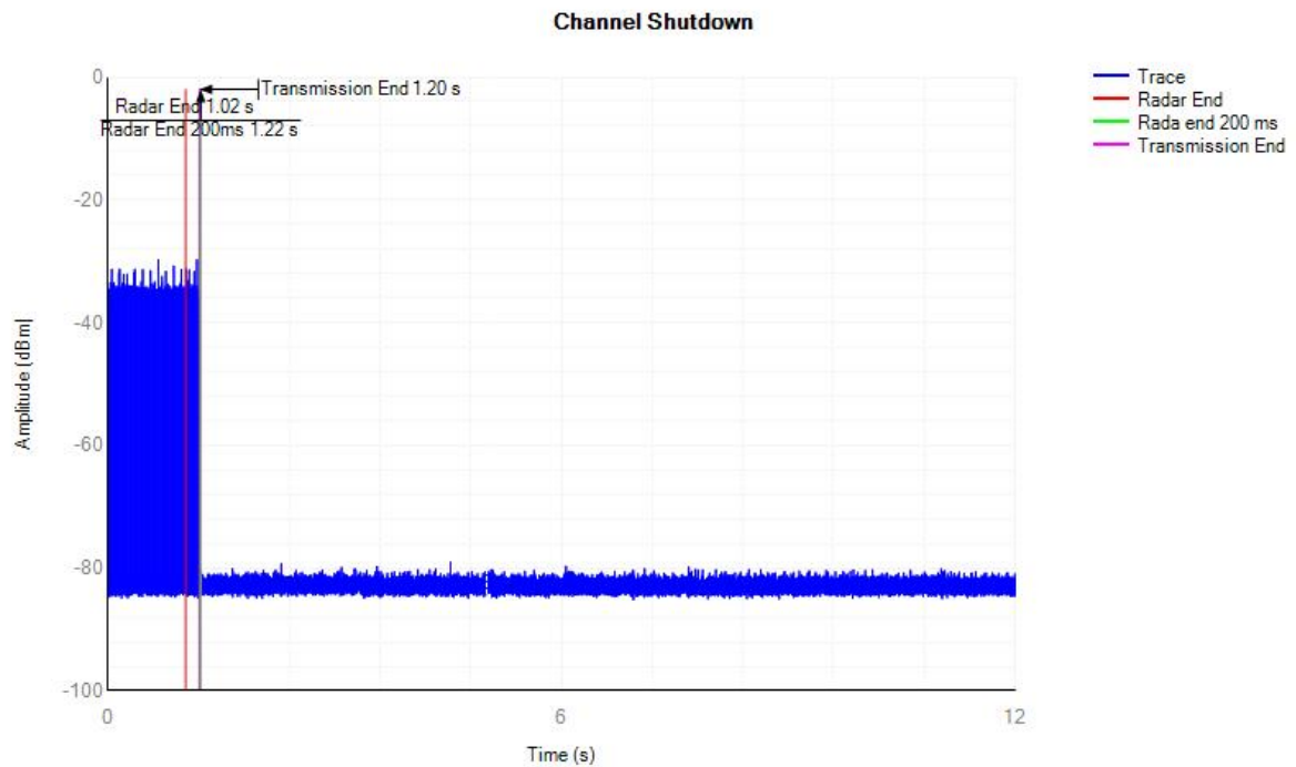
ax80 5530MHz Shutdown
