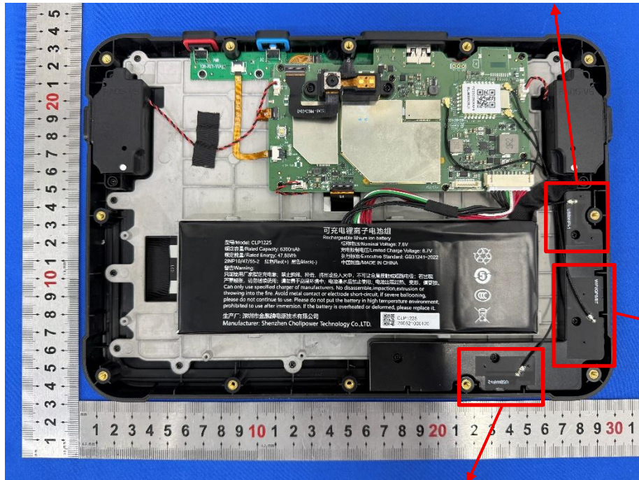
USB Module WIFI Antenna 2
