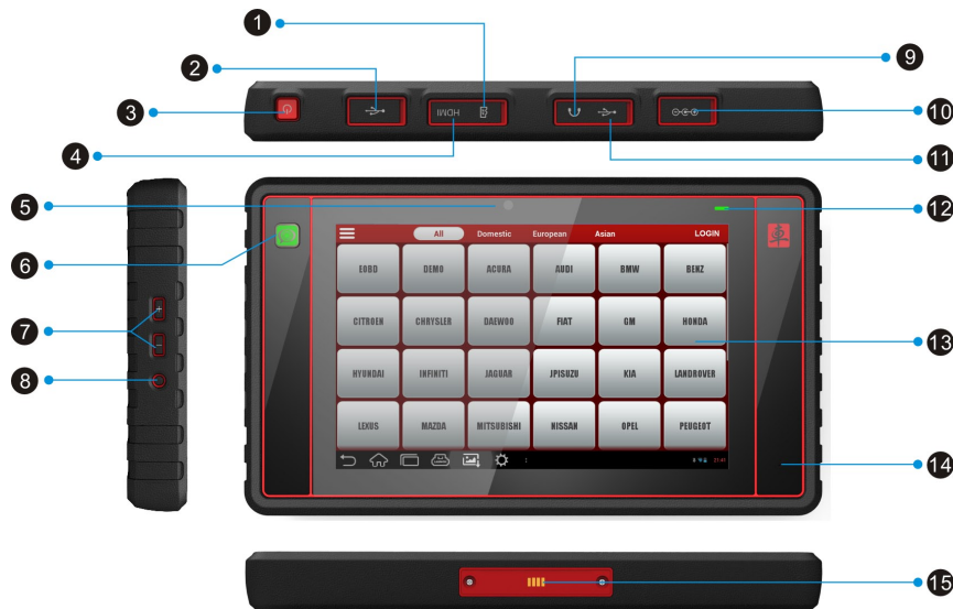
Fig. 2-4 X-431 PADII Tablet (front & side view)
