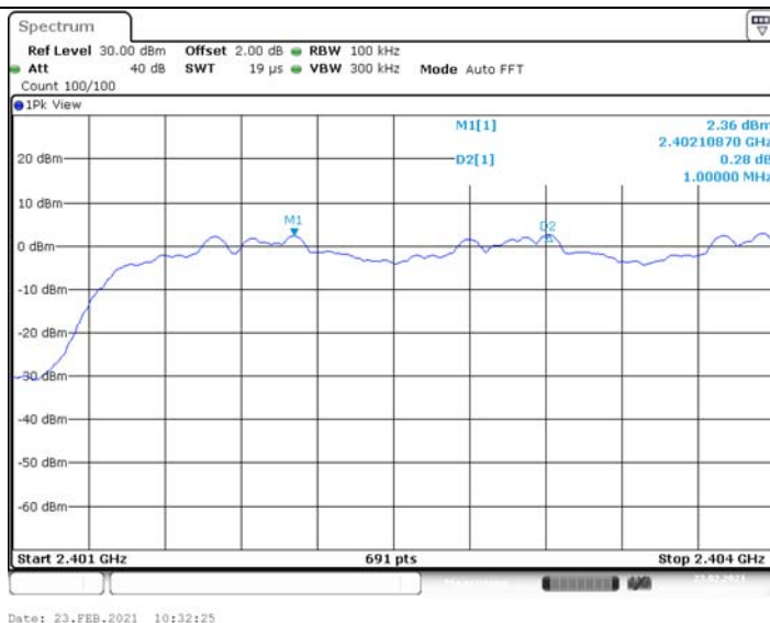
\pi /4-DQPSK_Hop_2441
