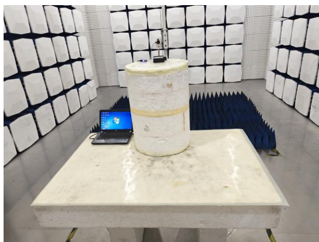
RE (18GHz-40GHz)
