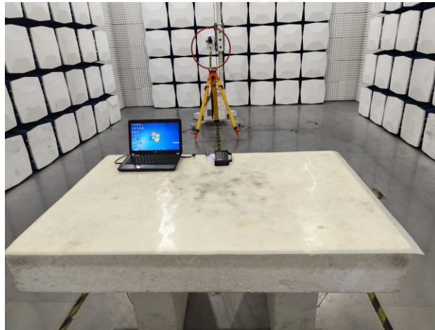
RE (30MHz-1GHz)
