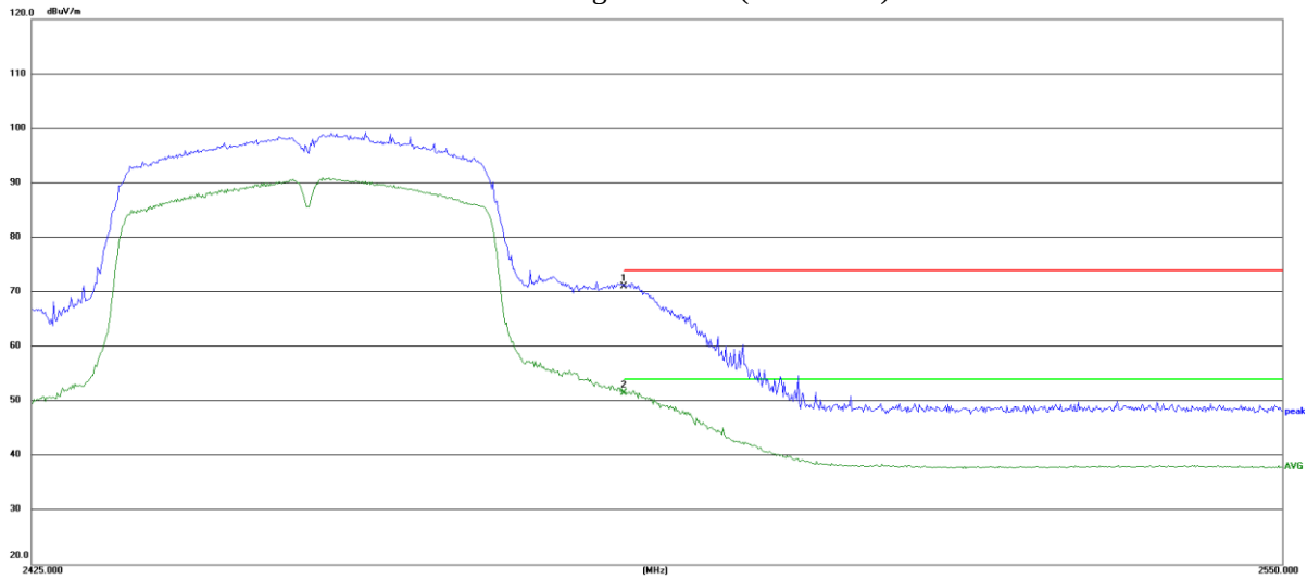
802.11n40 Horizontal High Channel (2452 MHz)-Above 1G
