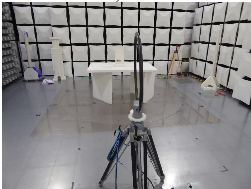
Antenna Position 2 – perpendicular Test setup semi-anechoic chamber M276 Preliminary measurement
