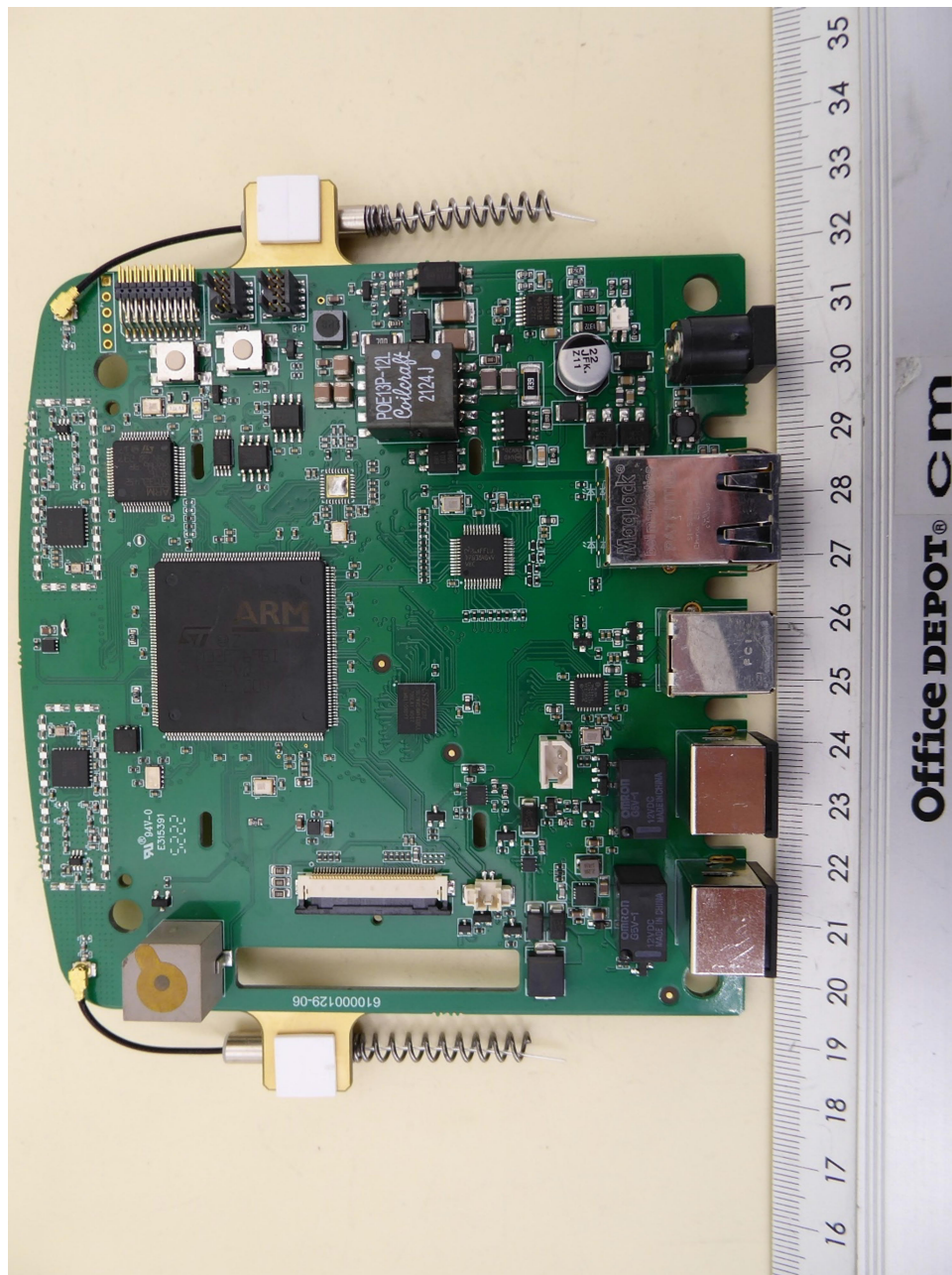
PCB, bottom view, shielding removed
