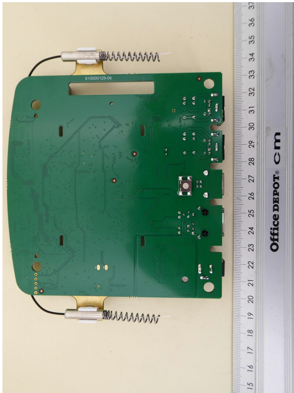
PCB, top view, display removed
