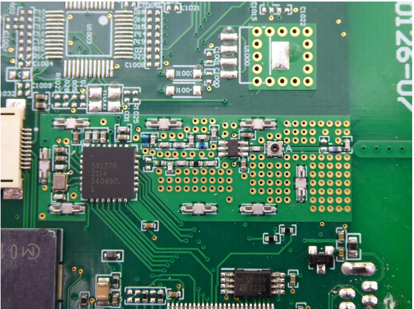
PCB Radio chip detail view
