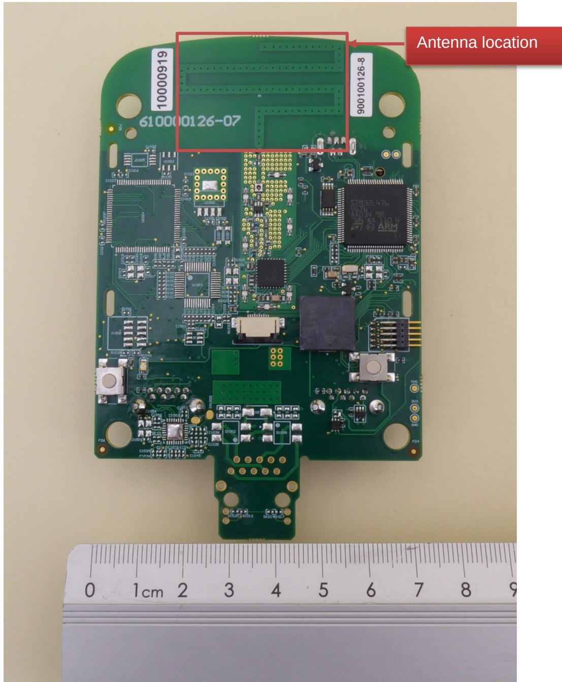
PCB Bottom view (Battery slot removed)
