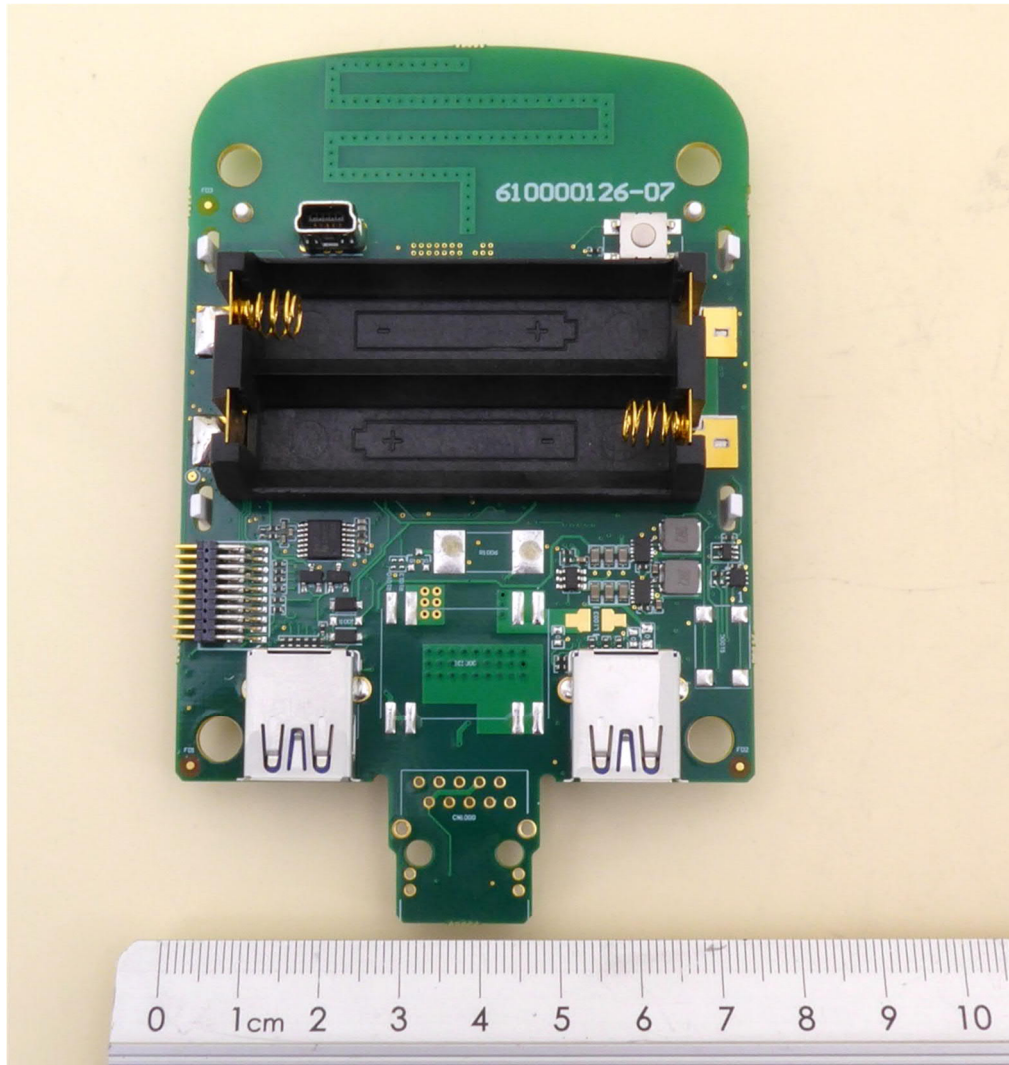
EUT – PCB Bottom view
