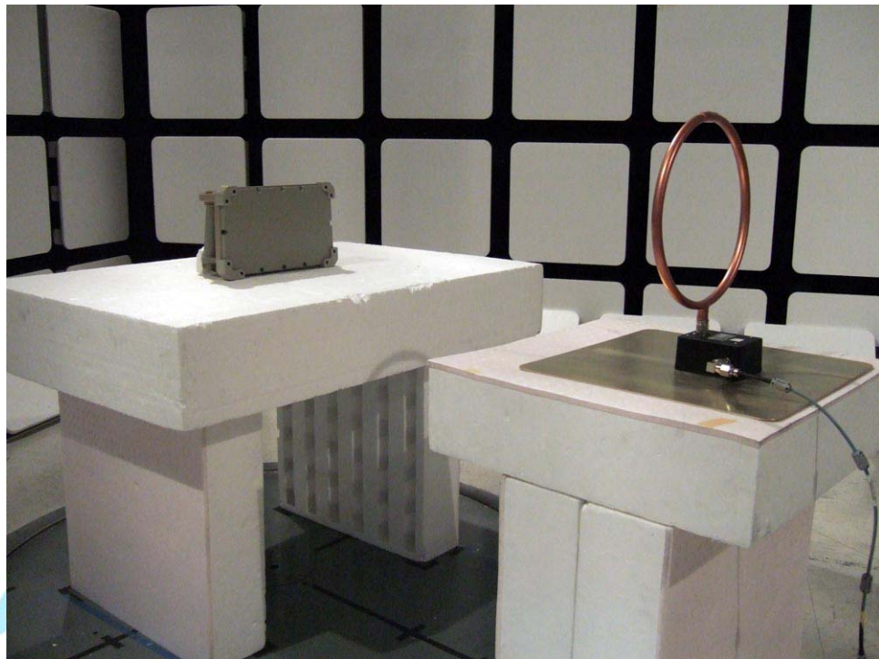
Test Configuration 4: 20 kHz to 30 MHz
