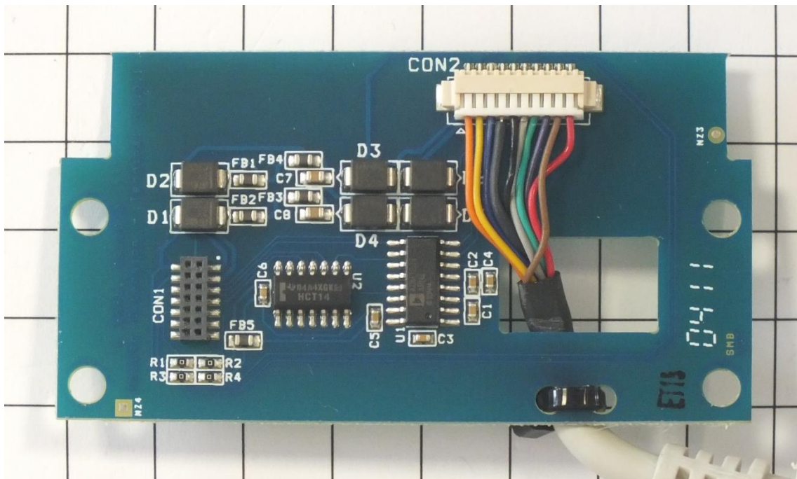
Circuit board:
