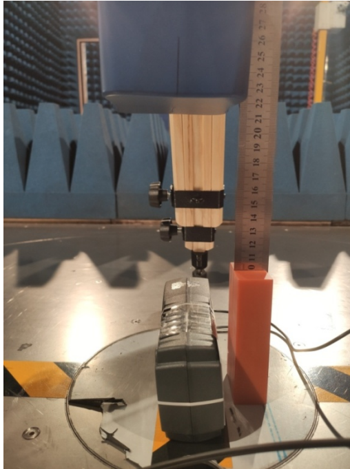
Left Edge_15mm
