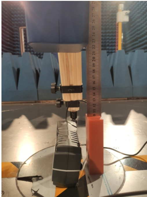
Right Edge_15mm
