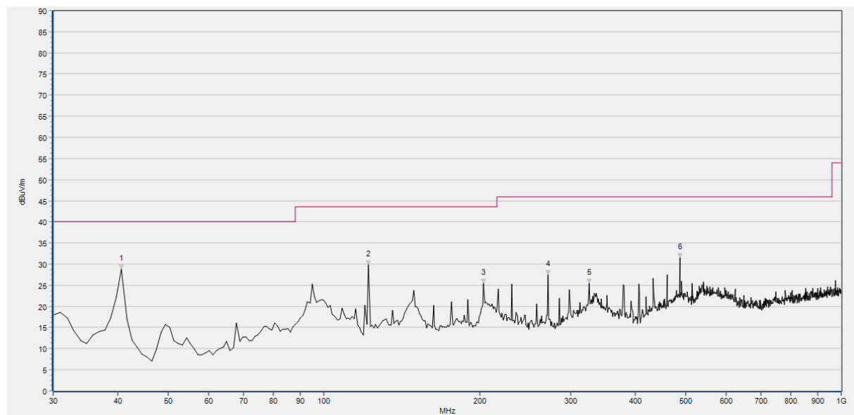
(Plot C: 30MHz – 1GHz, Test Antenna Vertical)
