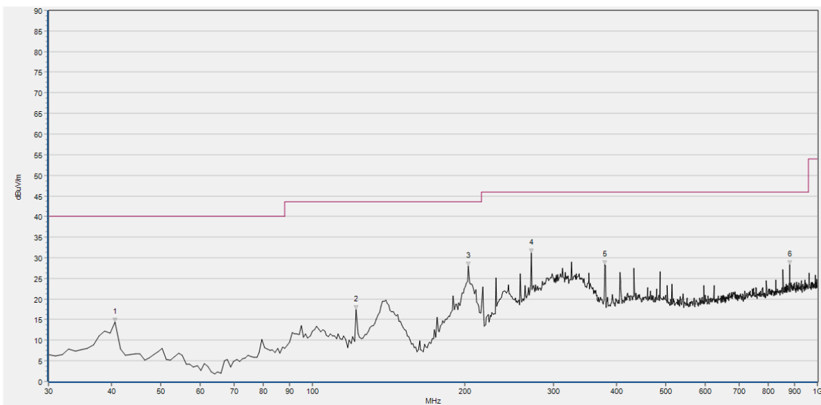
(Plot B: 30MHz – 1GHz, Test Antenna Horizontal)
