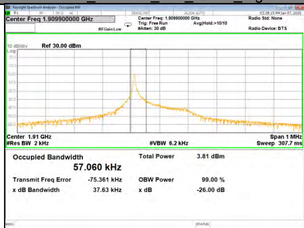
Band 2 3.75KHz 1#0_QPSK_High
