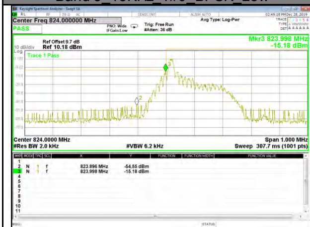
Band 5 15KHz 1#0 BPSK Low
