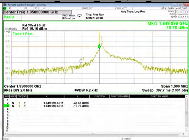
Band 2 3.75KHz 1#47_QPSK_High
