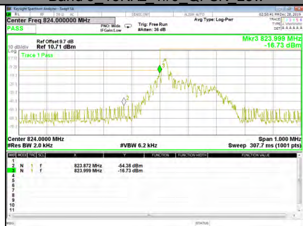
Band 5 15KHz 1#0 QPSK Low
