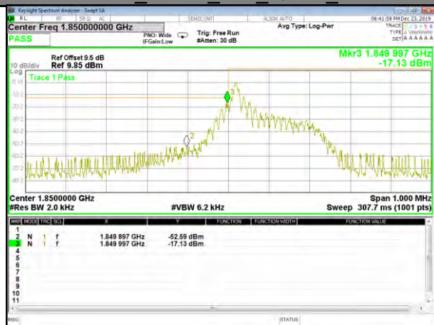
Band 2 15KHz 1#0_QPSK_Low
