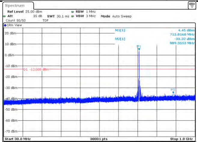
Band 12_3.75KHz_1#47_QPSK_High
