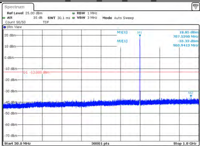
Band 12_15KHz_1#11_BPSK_Mid
