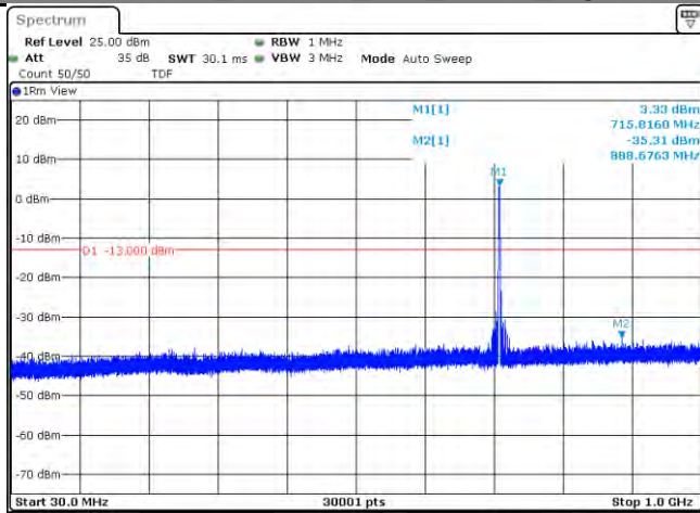
Band 12_3.75KHz_1#0_QPSK_High
