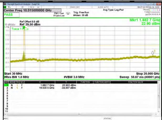
Band 25 3.75KHz 1#47 QPSK Mid
