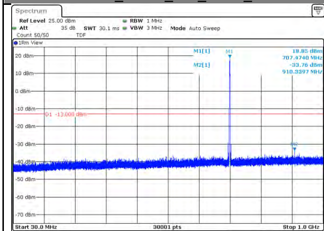
Band 12_15KHz_1#0_BPSK_Mid
