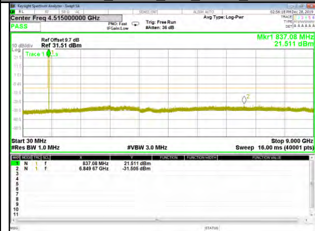
Band 5 15KHz 1#0 BPSK High
