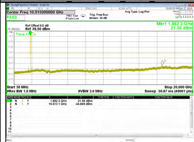
Band 25 15KHz 1#0 BPSK Mid
