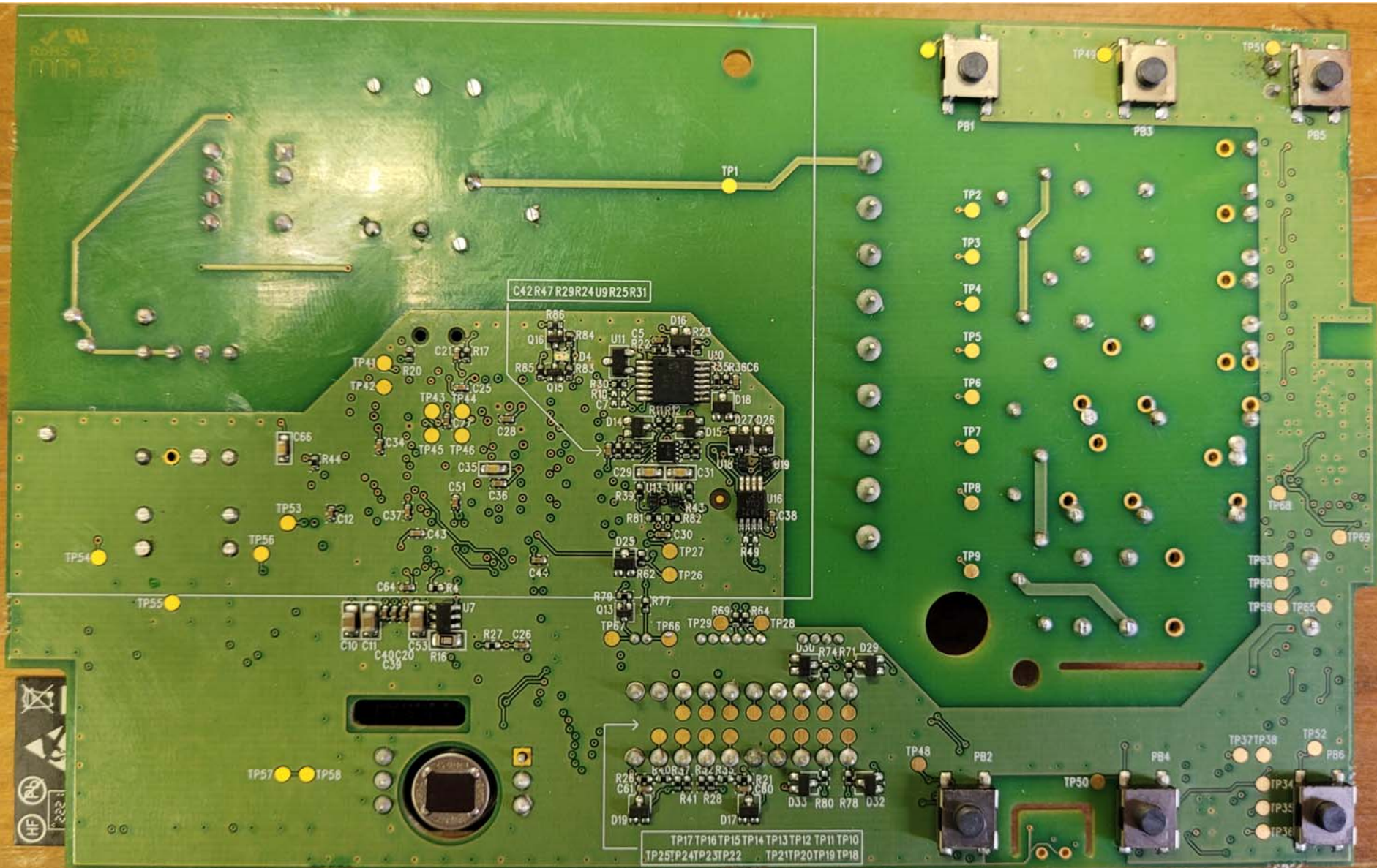
NO Display - Bottom View of the PCB - View #2
