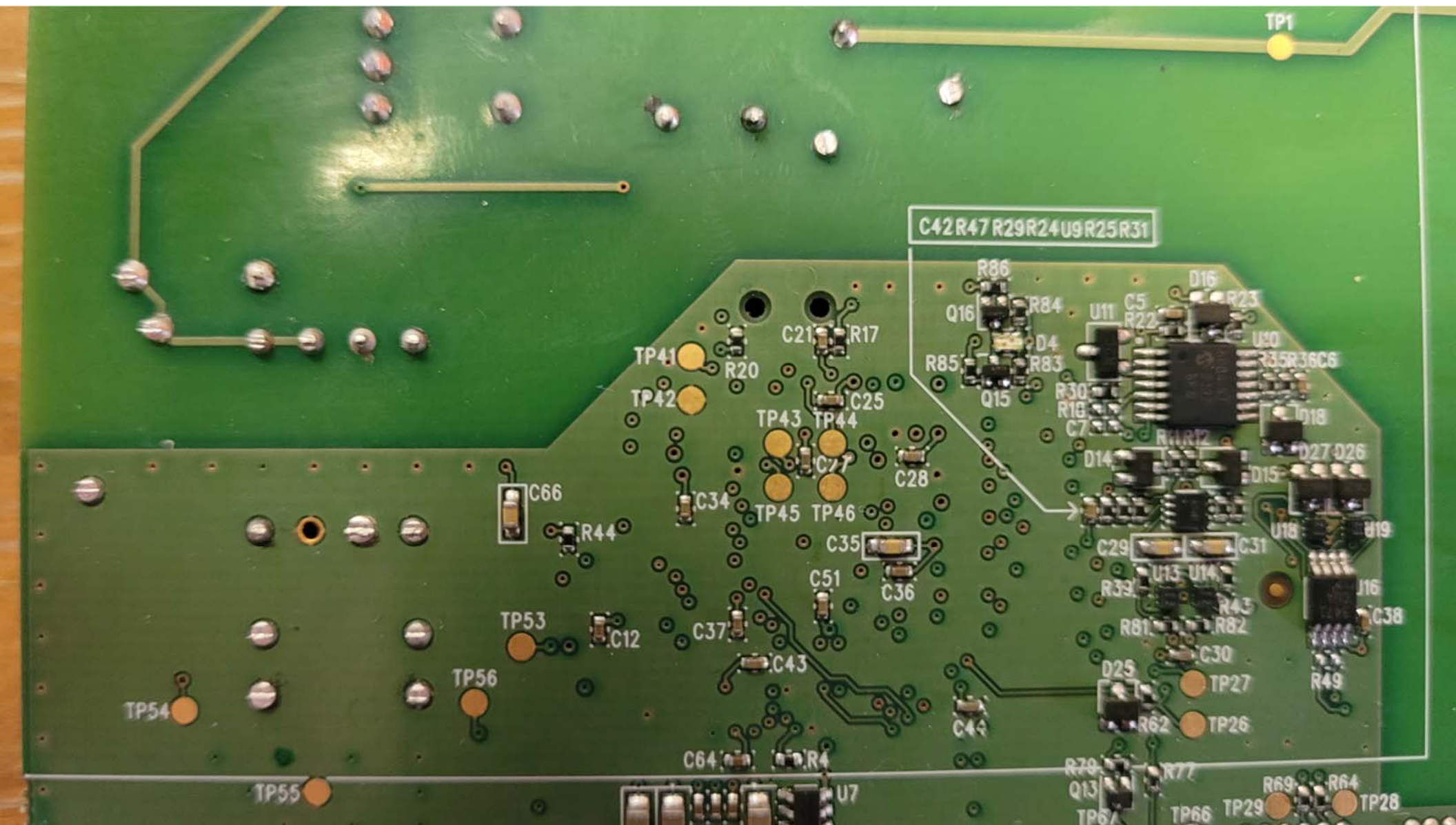
NO Display - Bottom View of the PCB - Closeup #2
