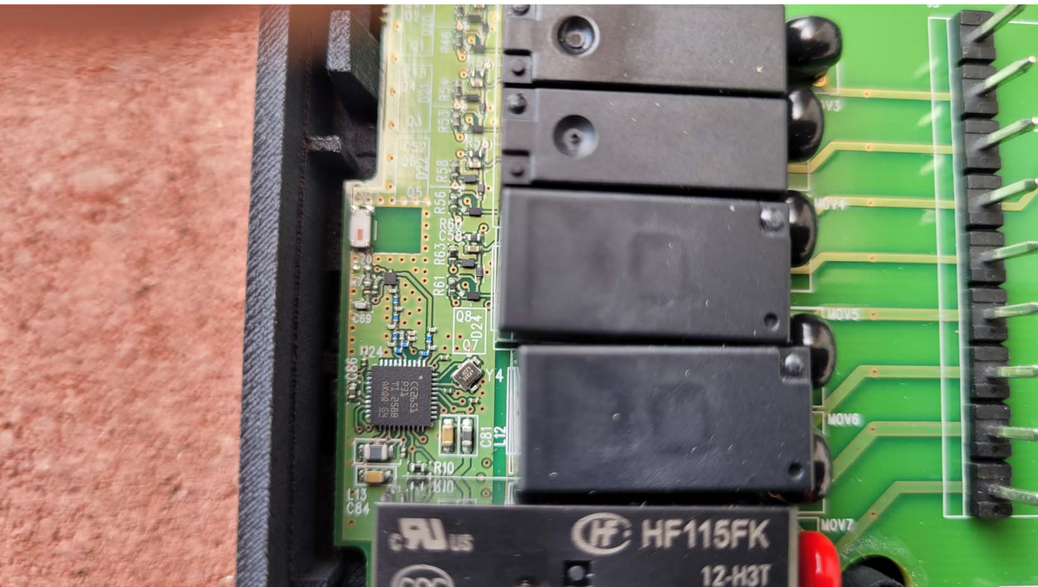
Top View of PCB - Closeup #8 - No Display
