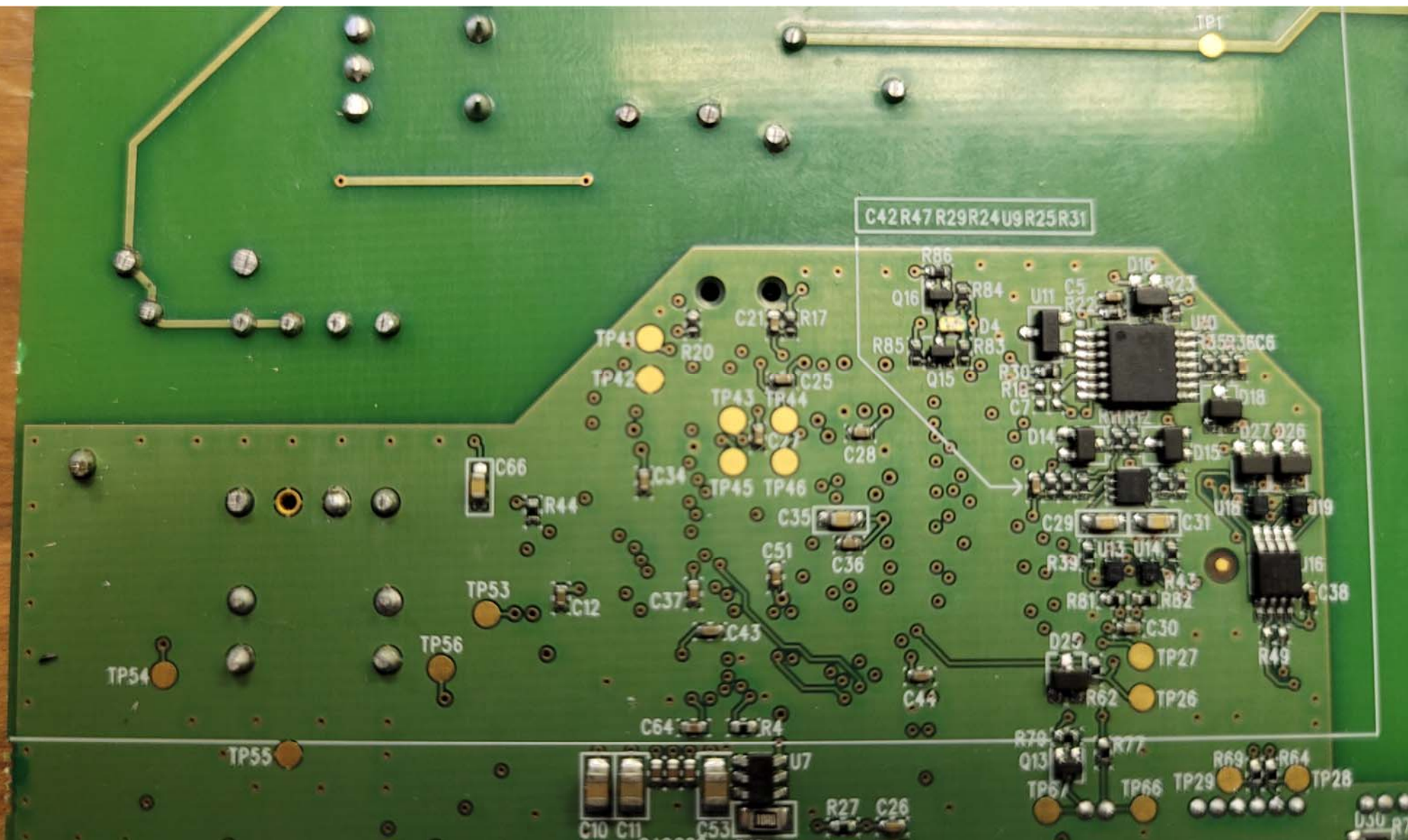
With Display - Bottom View of the PCB - Closeup #2
