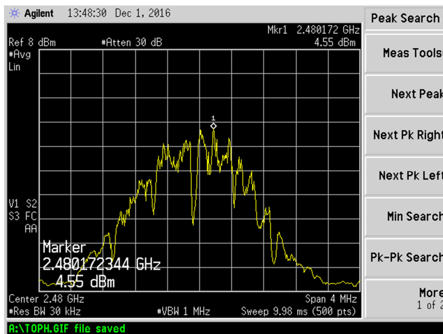
Figure 2.8.9-4 - High Channel PSD
