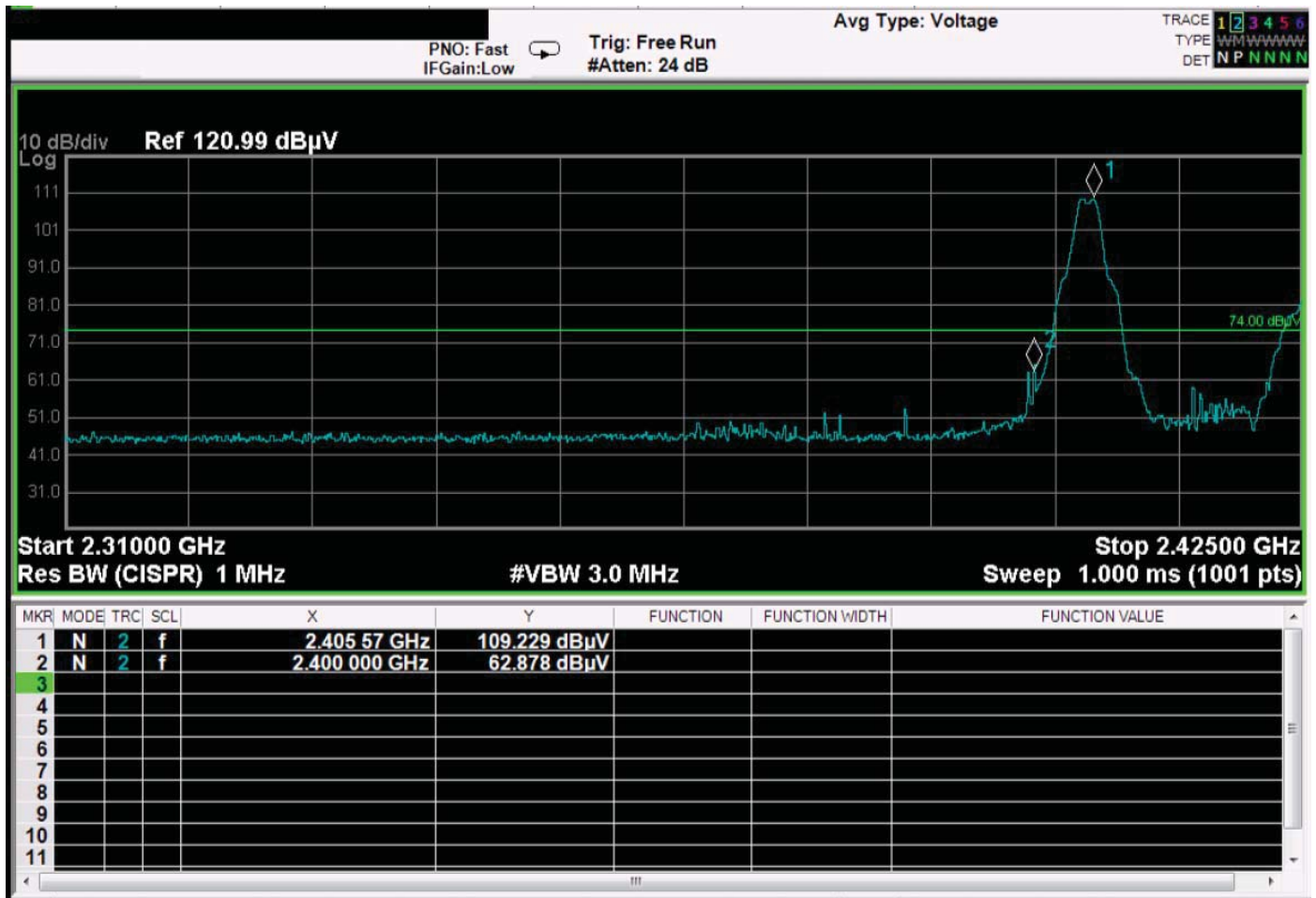
Band Edge – Vertical Polarization – Low Channel – X-Axis Worst Case
