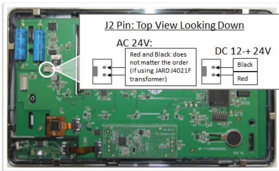
Figure 28: J2 Pin
