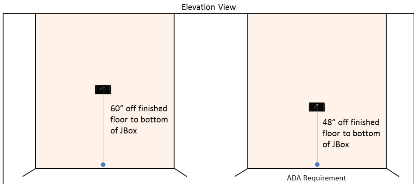
Figure 24: Mounting Height
