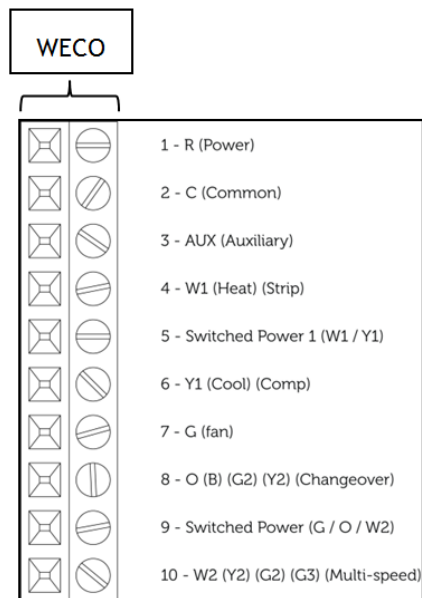
Figure 7: Wiring
