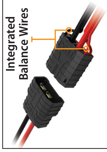
Traxxas High-Current Connector (4S) with iD and integrated balance wires
