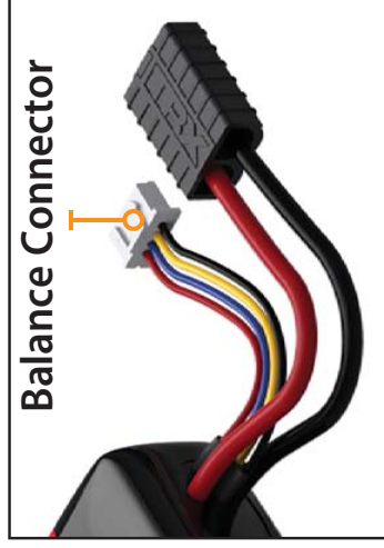
LiPo Balance Connector (without iD)
