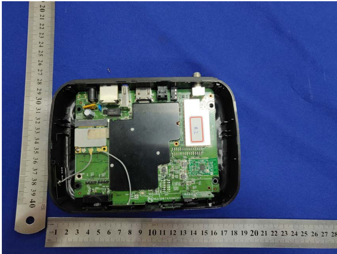
Host Device
