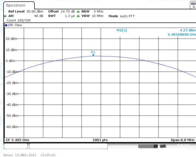
3DH5_2402
