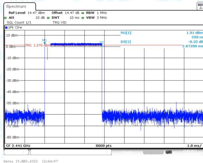
2DH5_Hop
