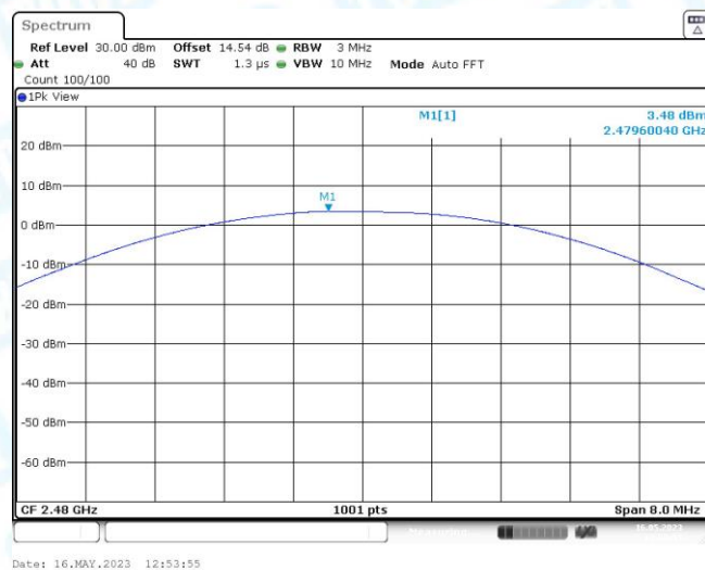
2DH5_2480
