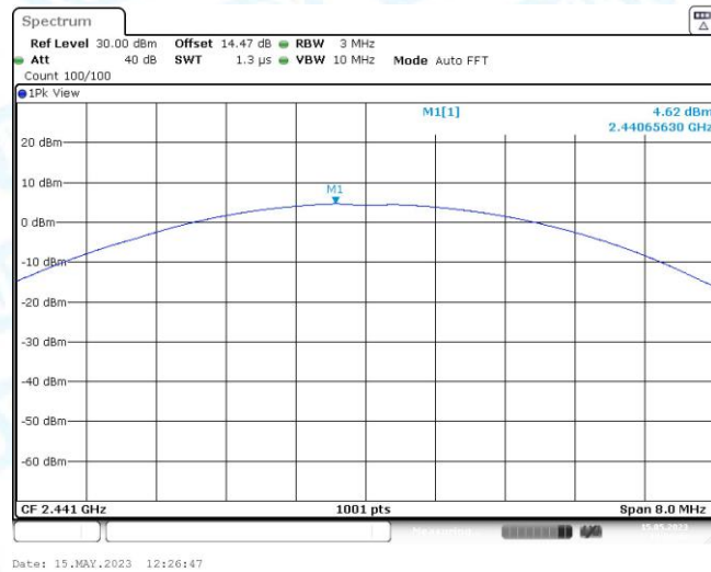
3DH5_2441
