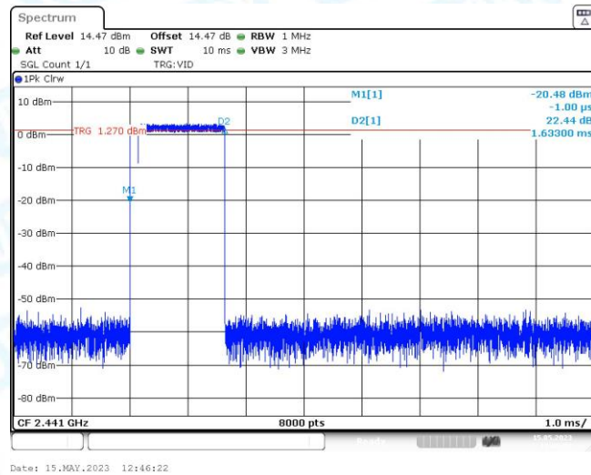
2DH3_Hop
