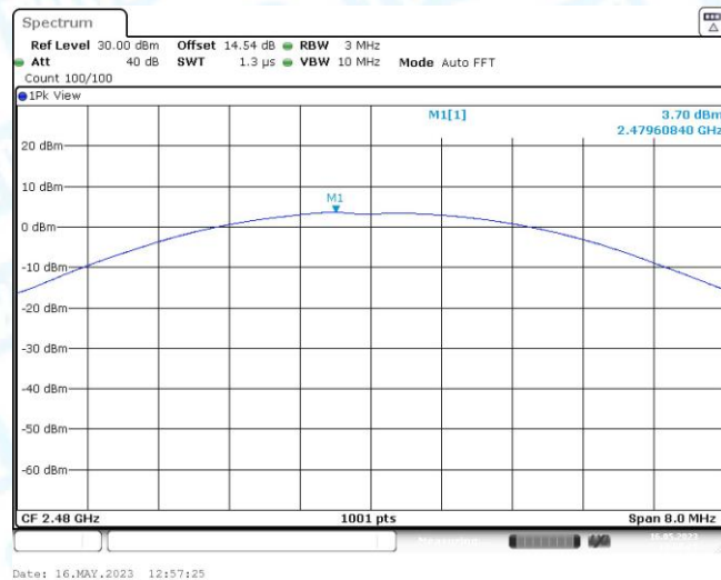
3DH5_2480
