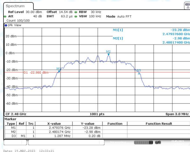
2DH5_2480
