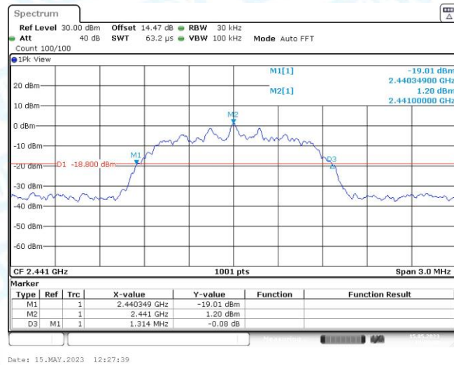
2DH5_2441
