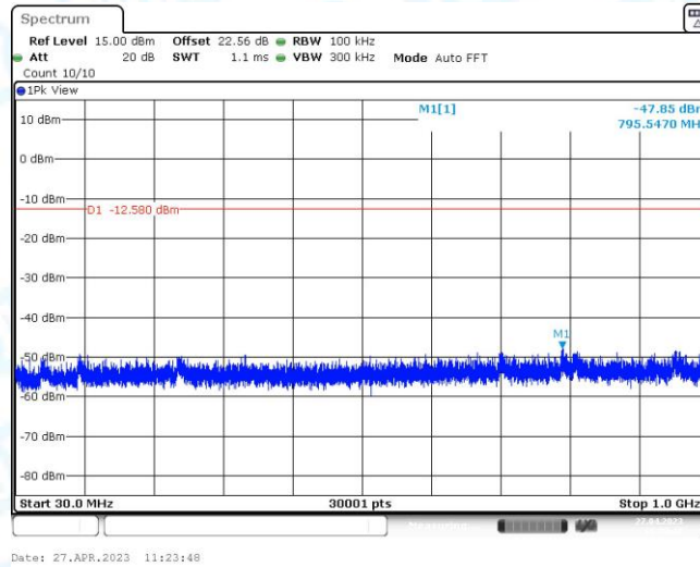
11G_Ant1_2437_30~1000
