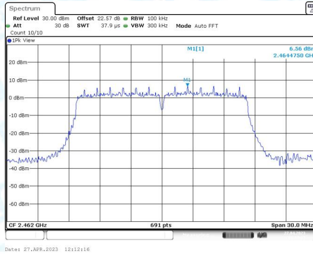
11G_Ant2_2462_0~Reference
