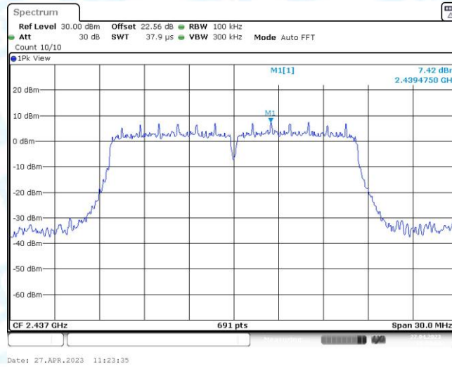
11G_Ant1_2437_0~Reference
