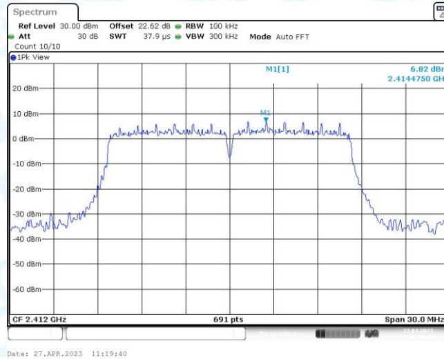
11G_Ant1_2412_0~Reference
