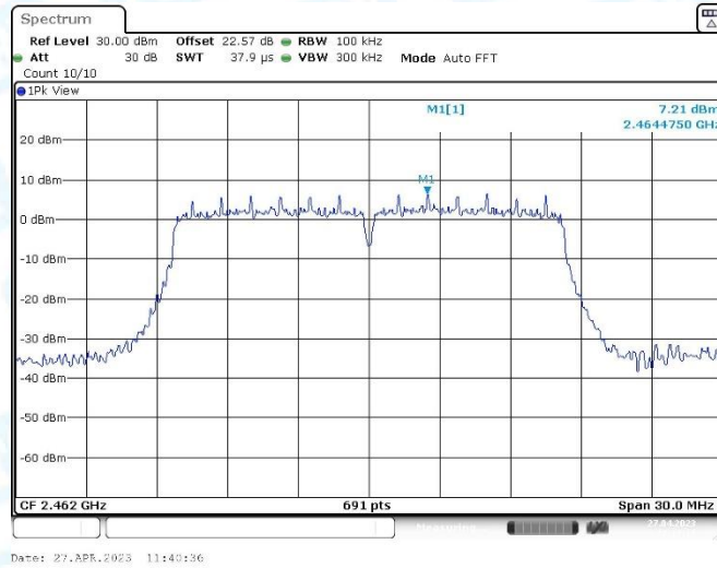
11G_Ant1_2462_0~Reference
