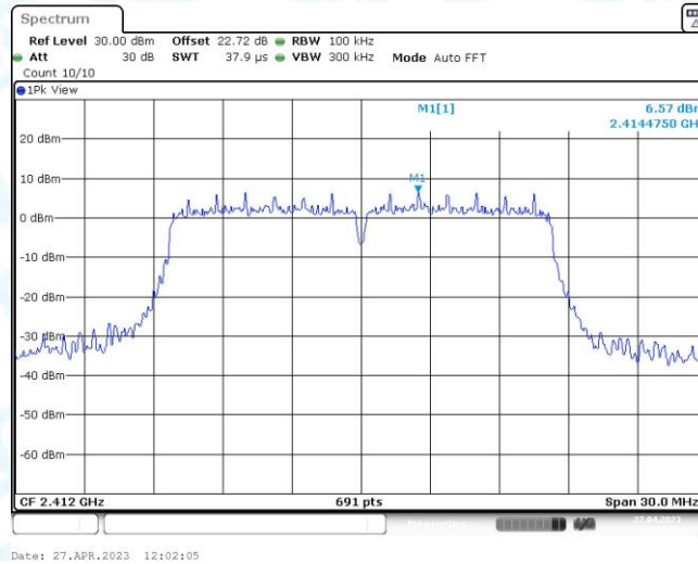
11G_Ant2_2412_0~Reference
