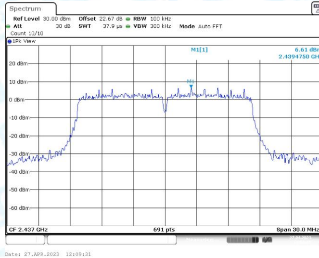
11G_Ant2_2437_0~Reference
