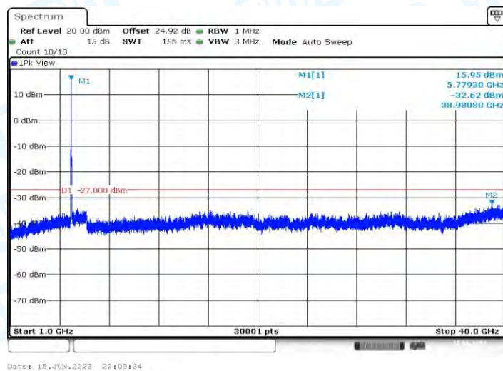
11AC20MIMO_Ant1_5785_1000~40000
