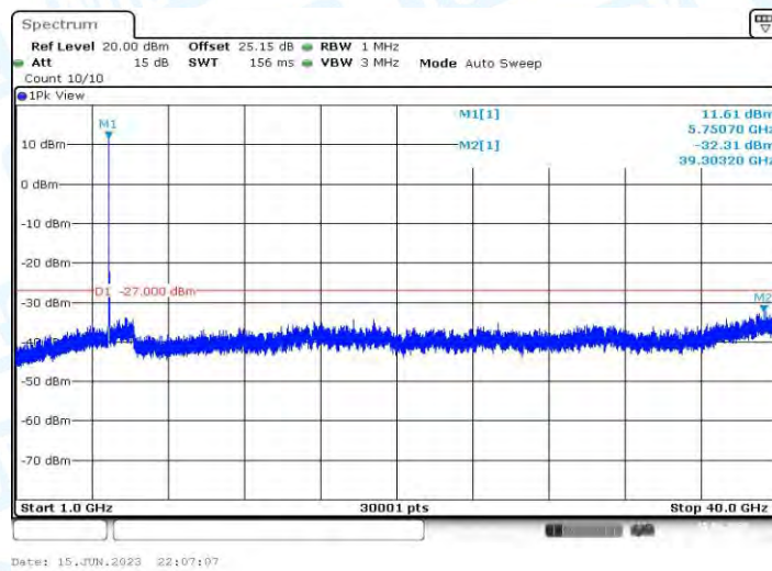
11AC20MIMO_Ant1_5745_1000~40000
