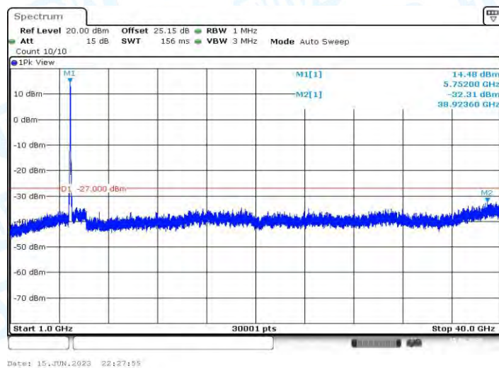
11AC40MIMO_Ant1_5755_1000~40000
