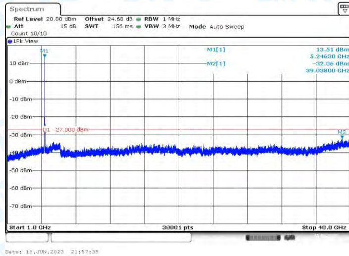
11AC20MIMO_Ant1_5240_1000~40000
