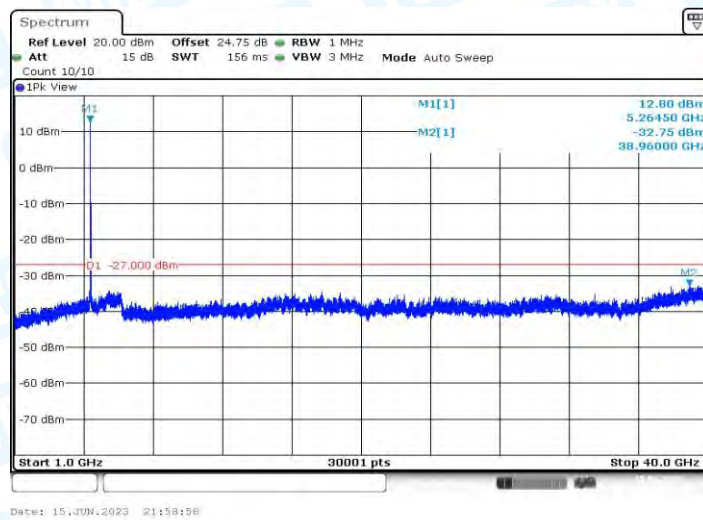
11AC20MIMO_Ant1_5260_1000~40000
