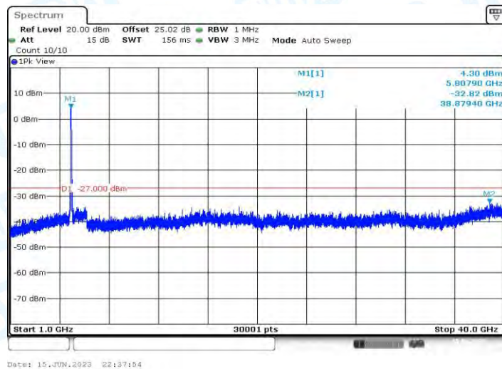
11AC80MIMO_Ant1_5775_1000~40000
