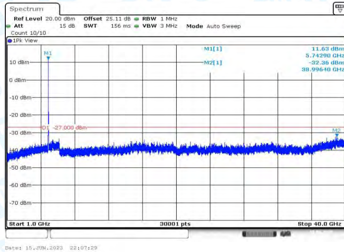
11AC20MIMO_Ant2_5745_1000~40000
