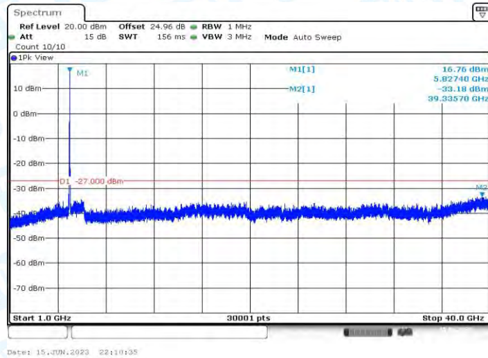
11AC20MIMO_Ant1_5825_1000~40000
