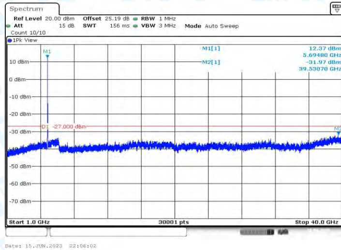
11AC20MIMO_Ant1_5700_1000~40000
