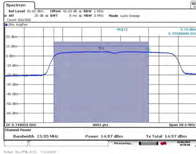
11AC20_Ant1&Ant2_5720_UNII-2C
