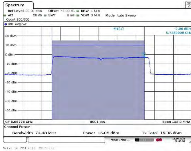
11AX80_Ant1&Ant2_5690_UNII-2C
