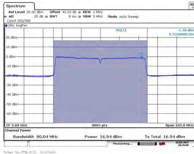
11AC80_Ant1&Ant2_5690
