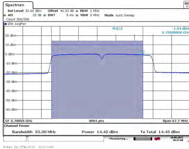
11AC40_Ant1&Ant2_5710_UNII-2C
