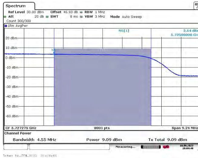
11AX20_Ant1&Ant2_5720_UNII-3
