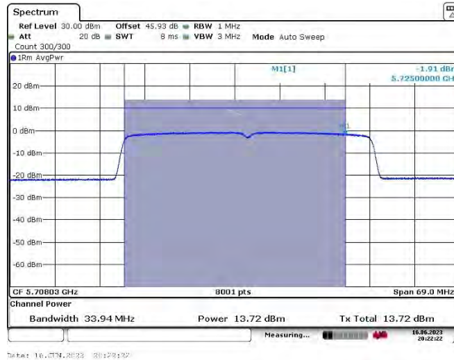
11AX40_Ant1&Ant2_5710_UNII-2C
