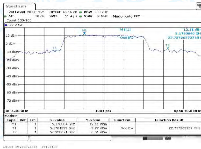
11A_Ant2_5180
