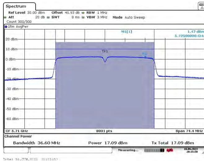
11AC40_Ant1&Ant2_5710
