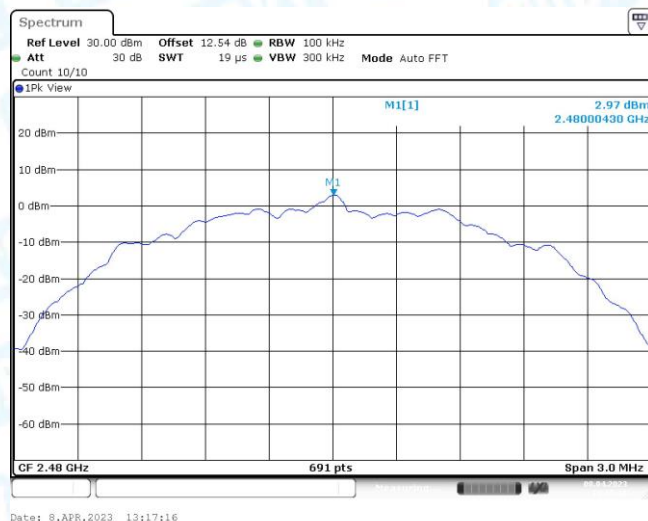
BLE_2M_2480_0~Reference
