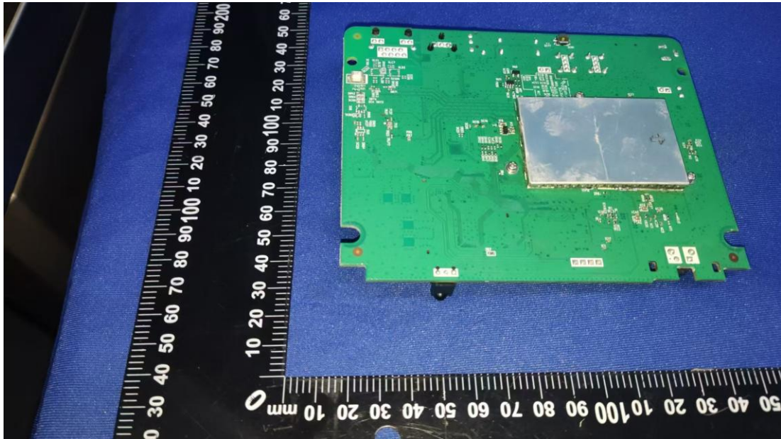
Figure 15 Inside of the EUT
