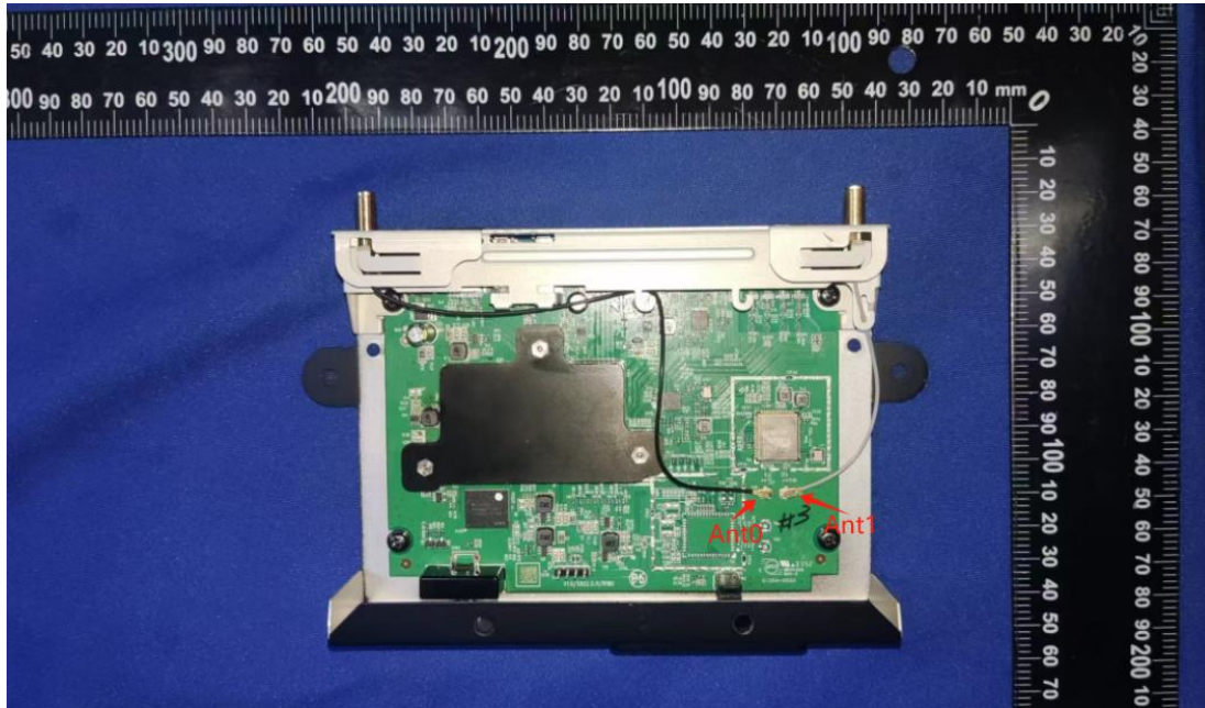
Figure 9 Inside of the EUT
